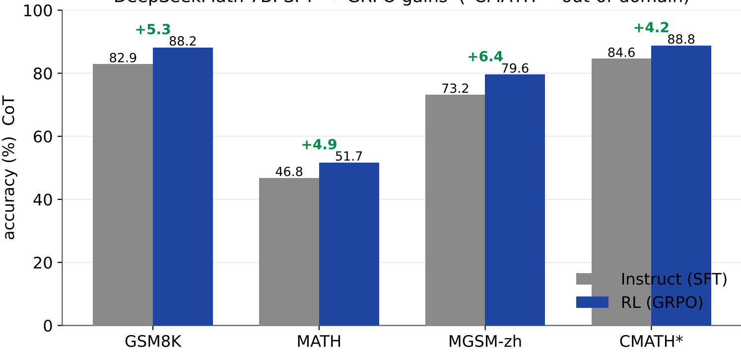
DeepSeekMath 7B: SFT → GRPO gains (*CMATH = out-of-domain)
