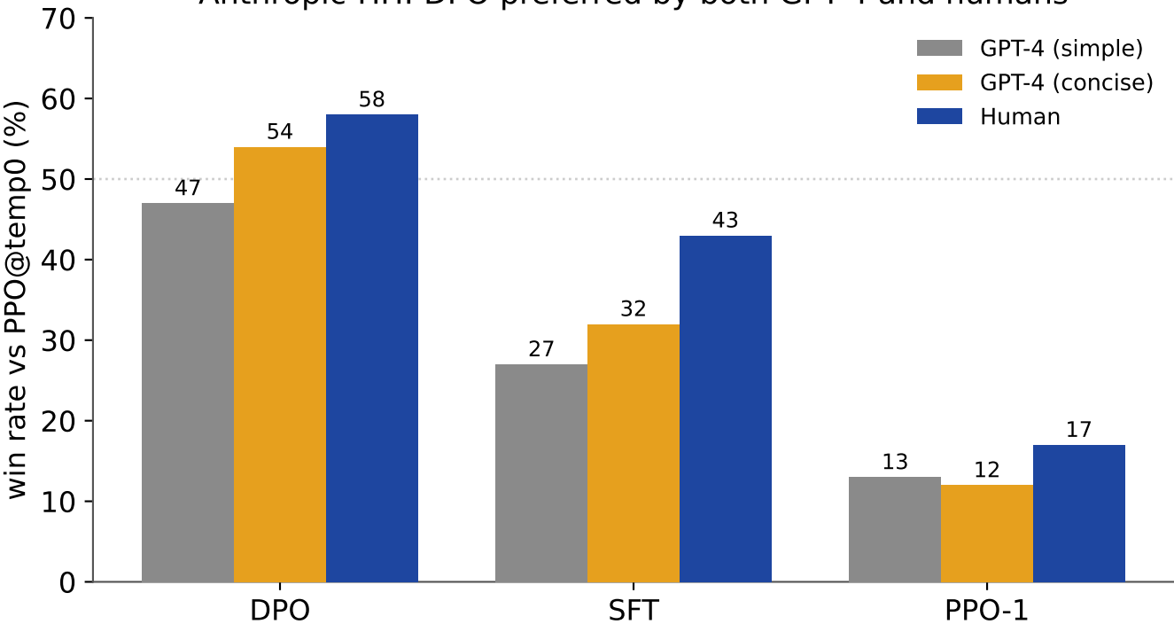
Anthropic-HH: DPO preferred by both GPT-4 and humans
