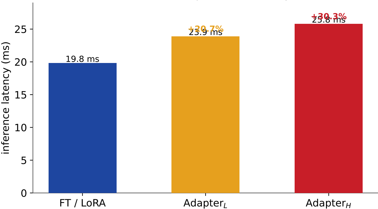
Online inference (batch 1): adapters add latency, LoRA adds none
