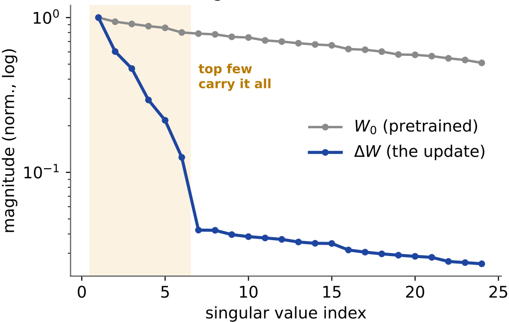
\Delta W 's singular values fall off a cliff
