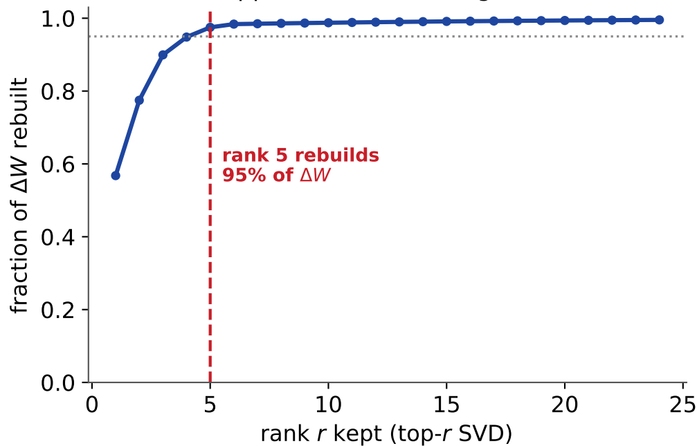
Best rank- r approx (Eckart--Young) is near-lossless
