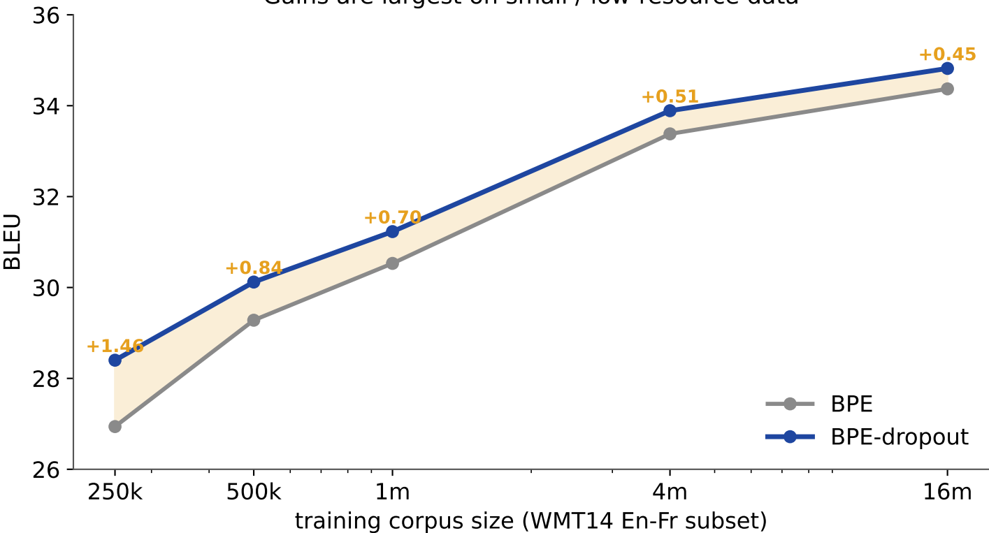
Gains are largest on small / low-resource data
