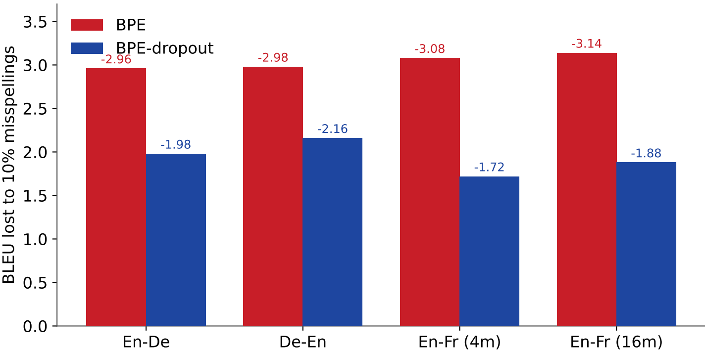
Robustness to noisy input: BPE-dropout degrades far less (lower is better)
