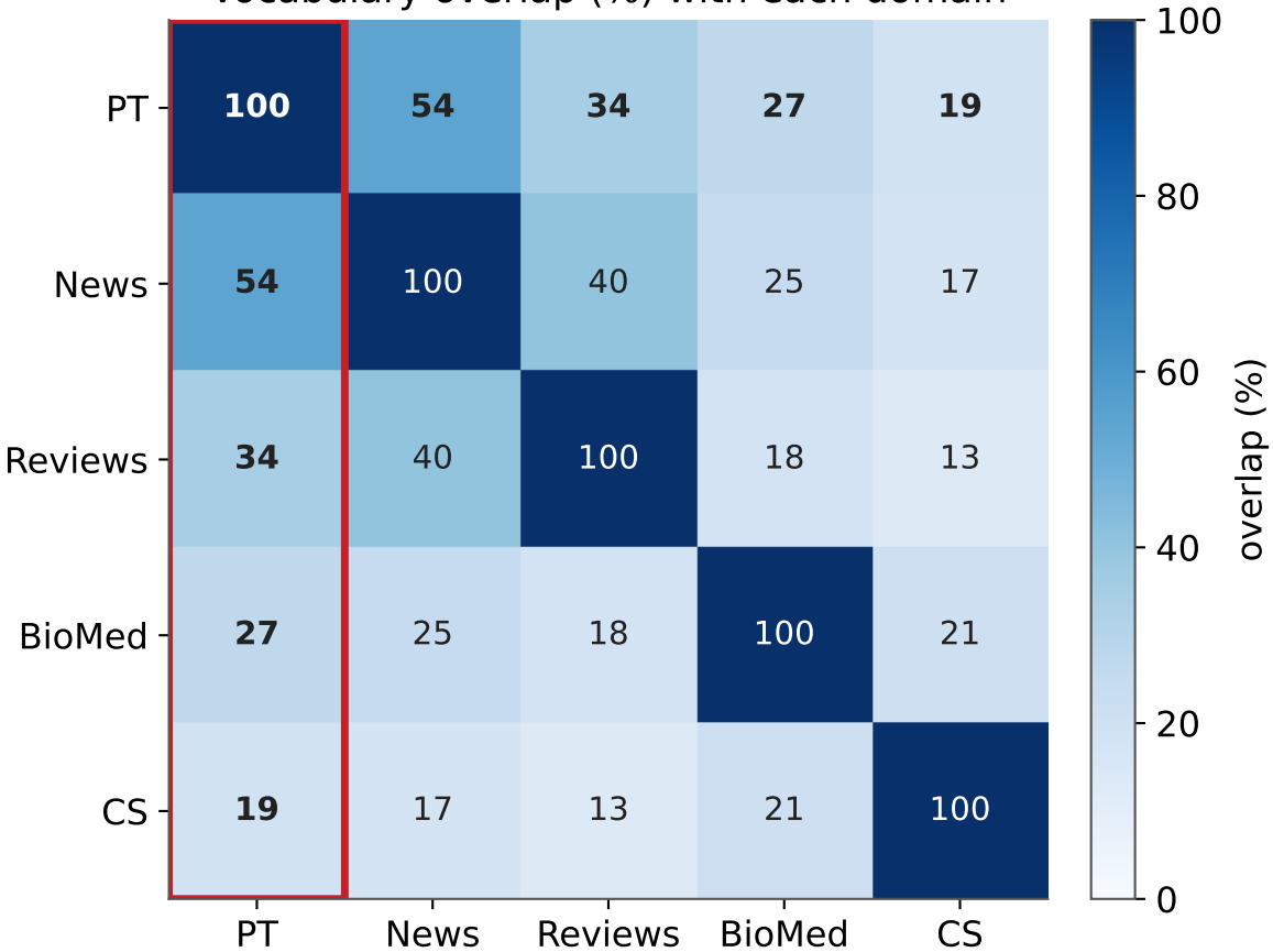
Vocabulary overlap (%) with each domain
