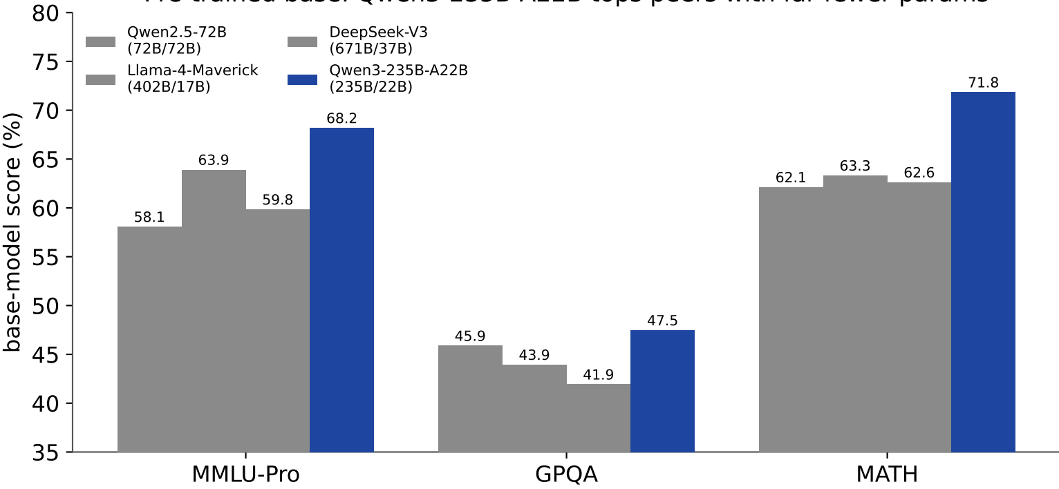
Pre-trained base: Qwen3-235B-A22B tops peers with far fewer params
