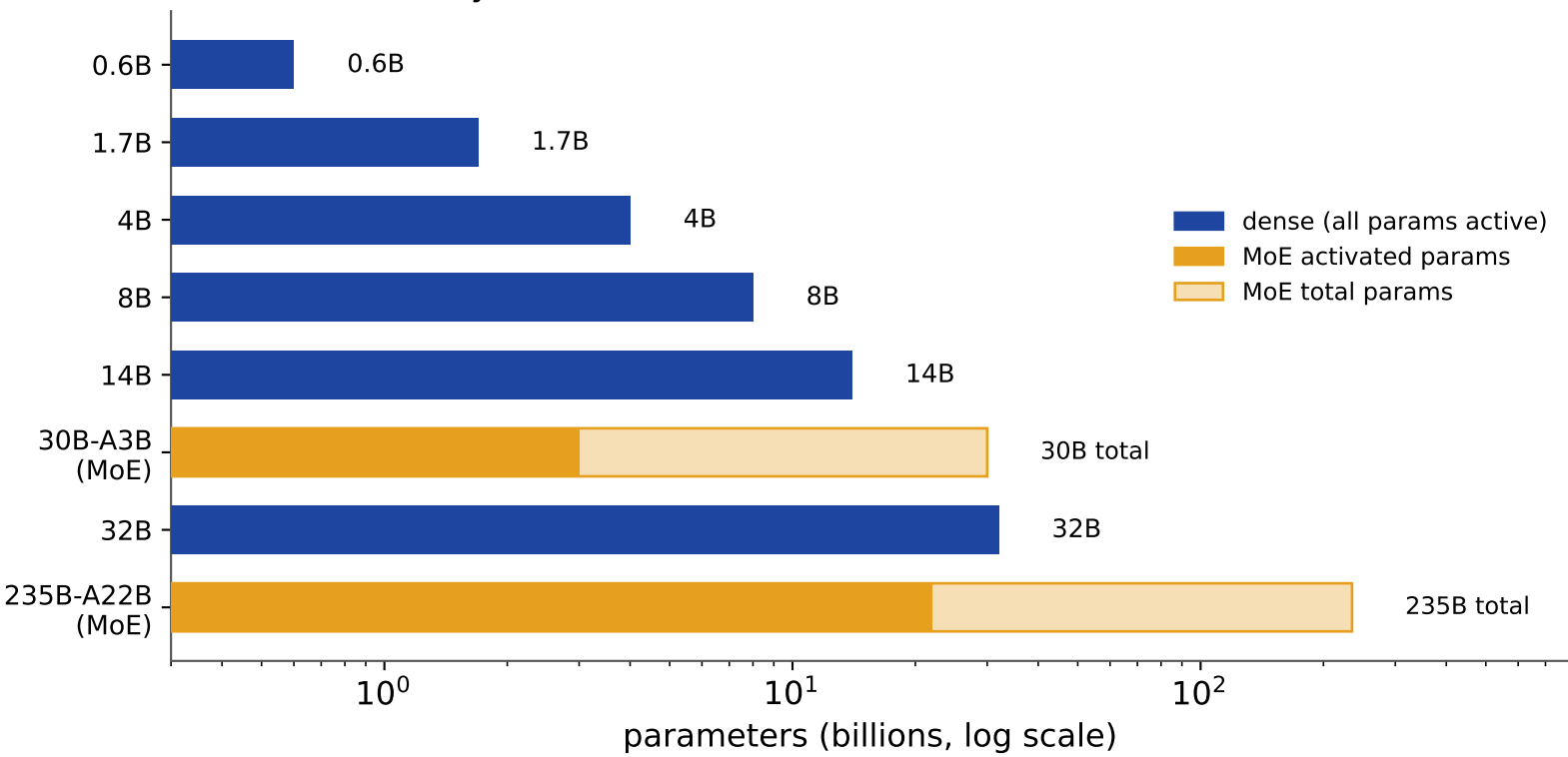
Qwen3 family: 6 dense + 2 MoE models; MoE activates a small fraction
