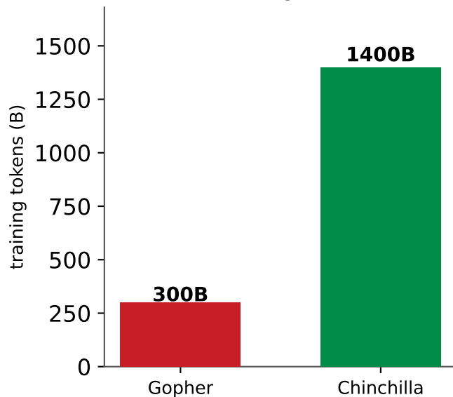
Training data
