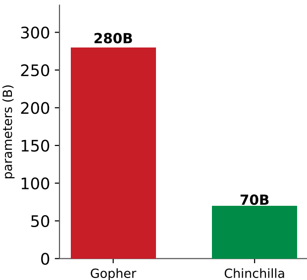
Model size
