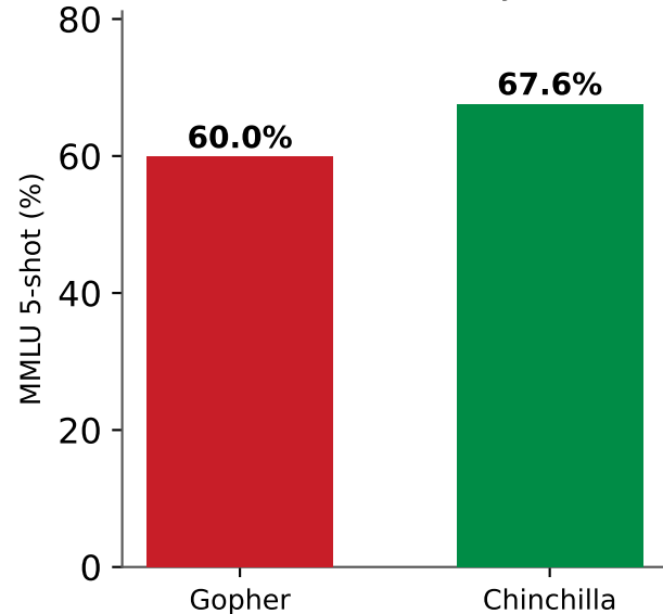
MMLU accuracy
