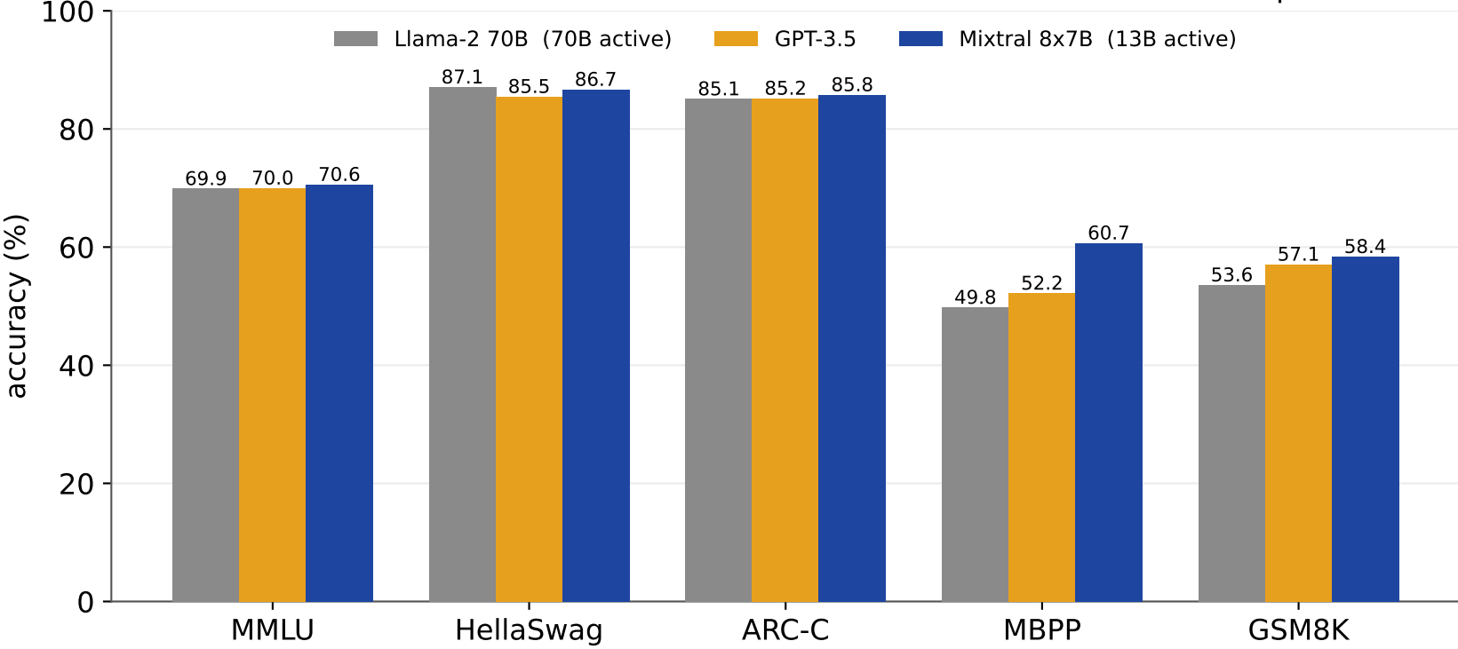
Mixtral 8x7B matches/beats Llama-2 70B & GPT-3.5 at 5x fewer active params
