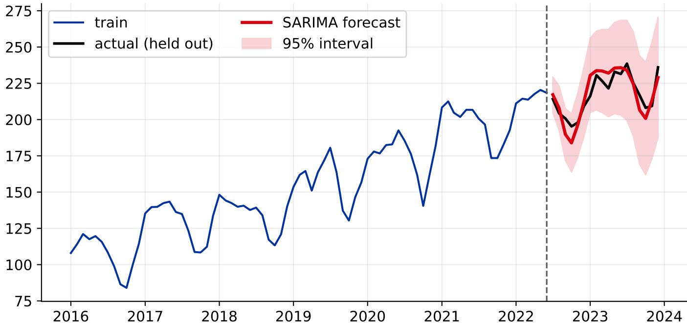
SARIMA(0,1,1)(0,1,1) 12 forecast -- the 'airline model'
