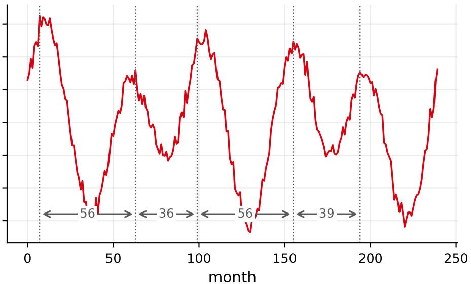
Cycle: swings with NO fixed period
