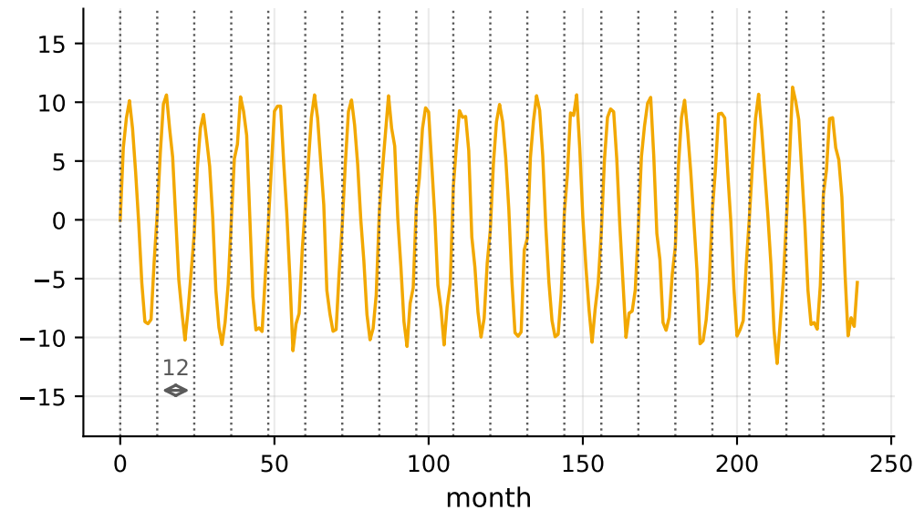
Seasonality: period is FIXED (every 12 steps)
