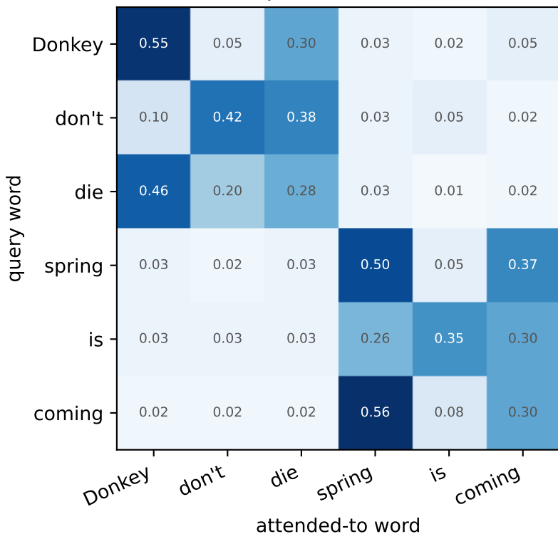
An attention pattern that makes sense
