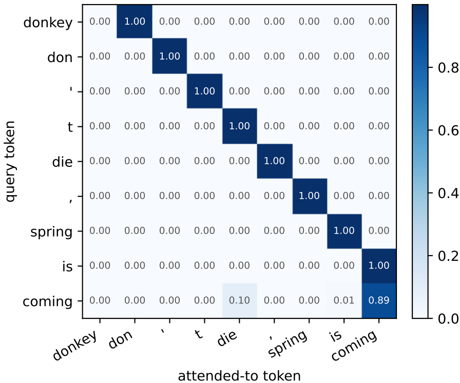
DistilBERT self-attention (layer 2, head 10)
