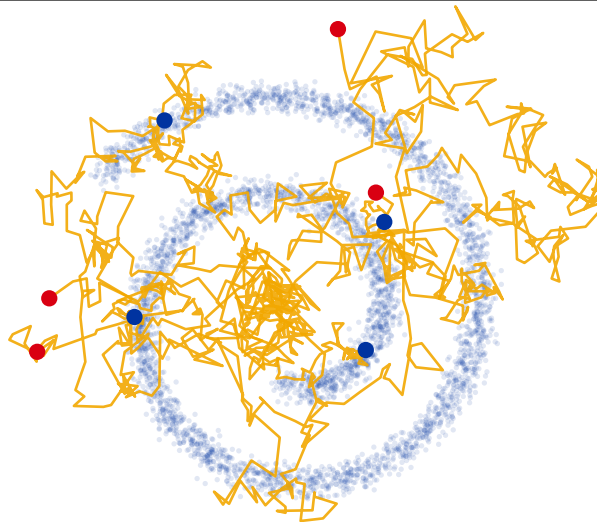
Noising one point = a random walk
