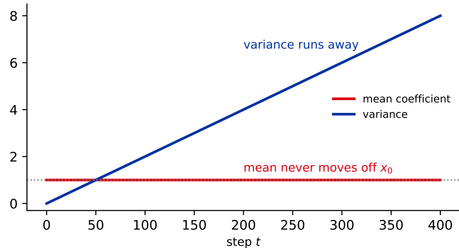
Variance exploding: x_t = x_0 + \sqrt{t\beta} \varepsilon
