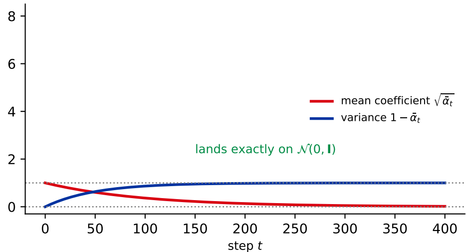
Variance preserving: x_t = \sqrt{\bar{\alpha}_t} x_0 + \sqrt{1 - \bar{\alpha}_t} \varepsilon
