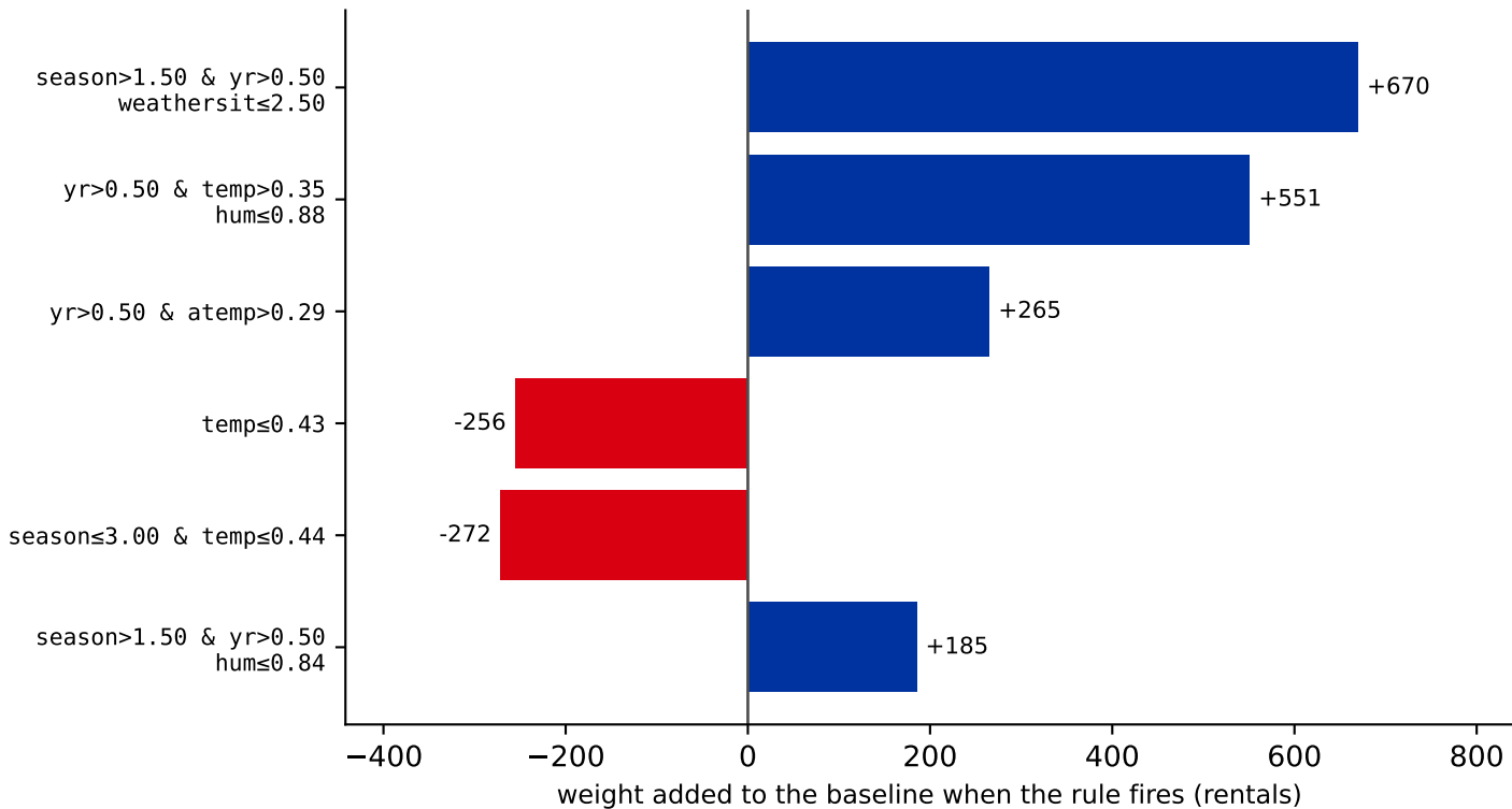
RuleFit scorecard on bike (baseline \approx 4,504 rentals)
