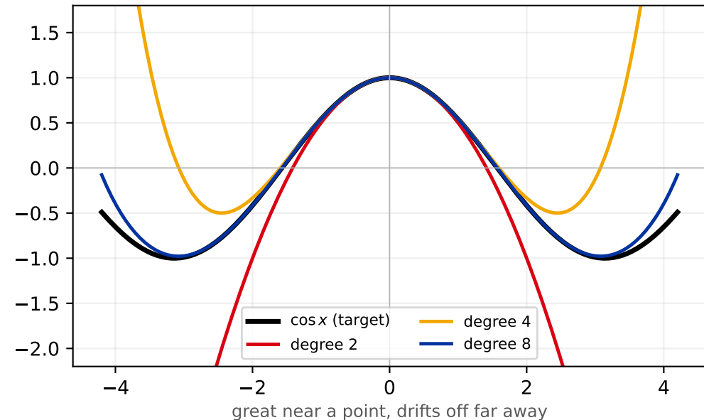
Taylor: sum of POWERS 1, x^2, x^4, \dots
