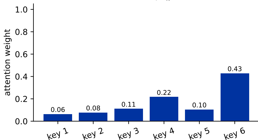
softmax of QK^\top / \sqrt{d_k} ( \approx \pm 1 )
