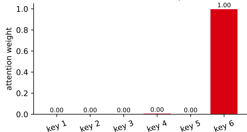
softmax of raw QK^\top (scores spread \approx \pm 5 )
