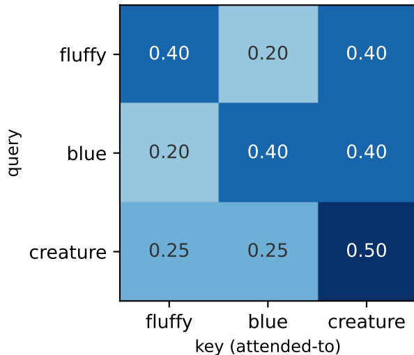
weights = \text{softmax}(S/\sqrt{d})
