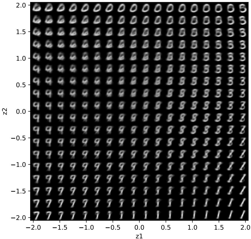
VAE latent grid: every point is a valid digit
