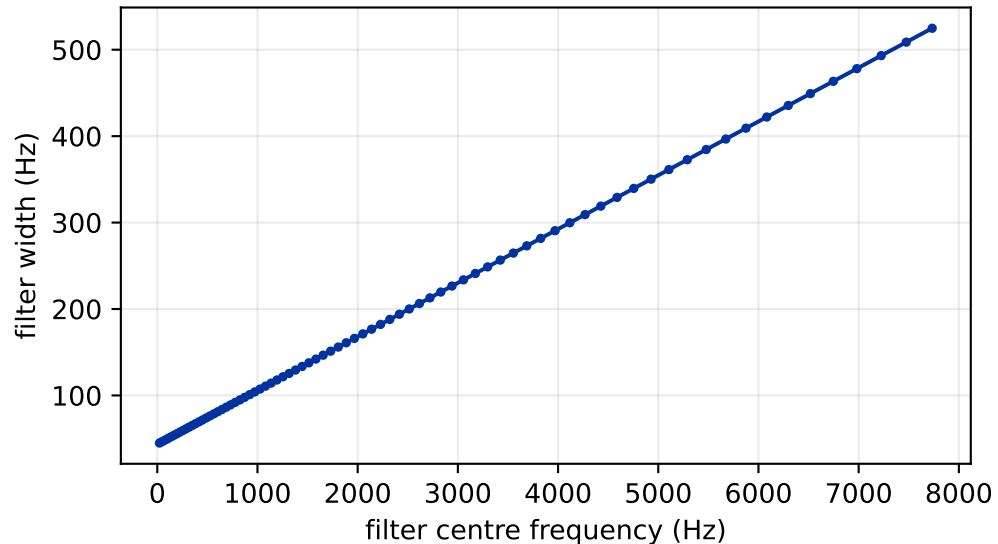
a filter near 8 kHz is \sim 9\times wider than one near 200 Hz
