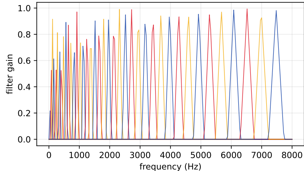
80 triangular mel filters (every 2nd shown)
