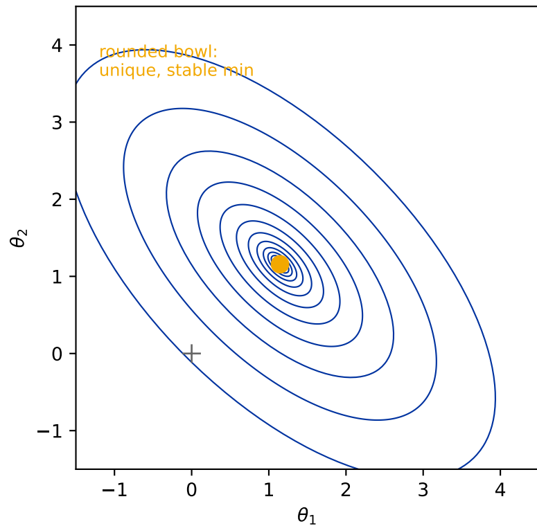
Add \lambda to the diagonal of X^T X
