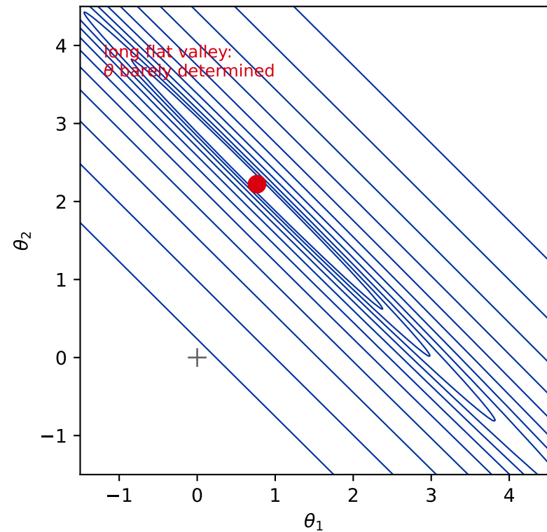
Collinear features: a least-squares ``ridge''
