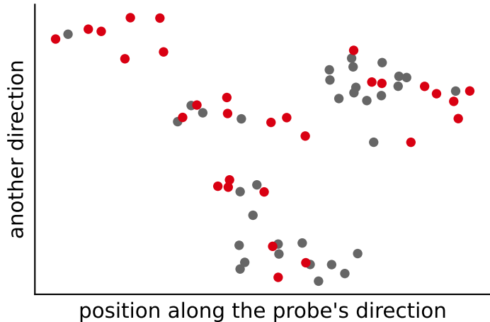
layer 0: 38% of unseen prompts right (chance is 50%)
