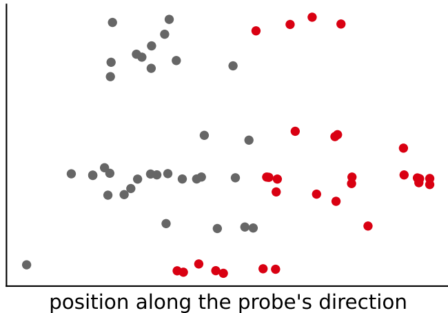
layer 3: 86% of unseen prompts right (trained on 64 prompts)
