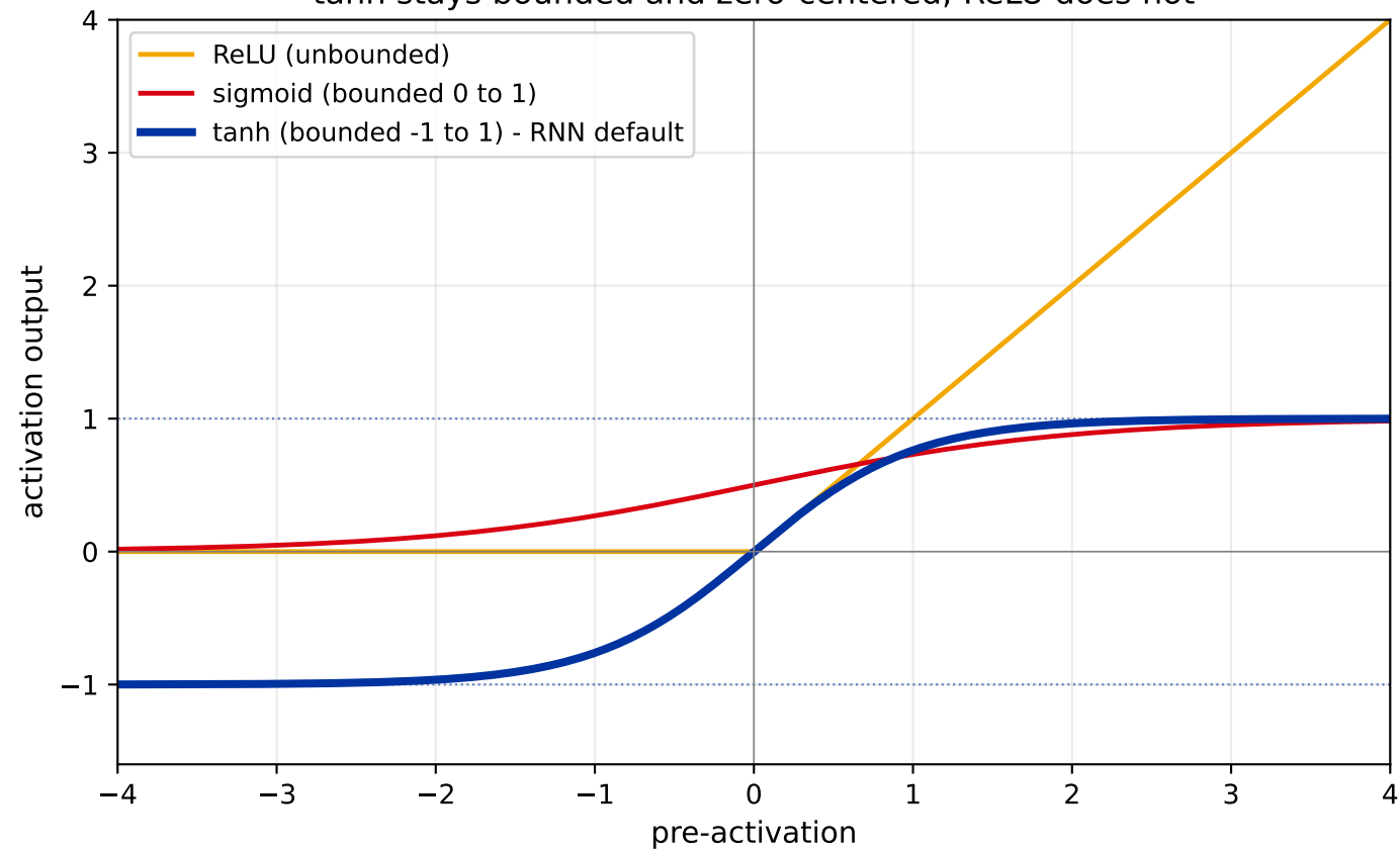
tanh stays bounded and zero-centered; ReLU does not
