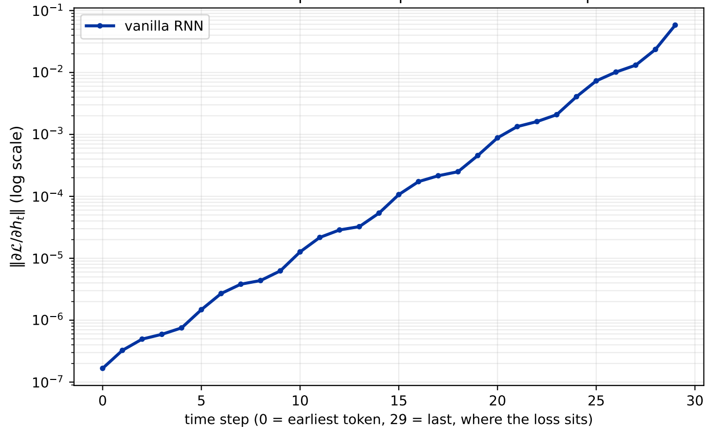
Gradient norm per time-step: dead within ~15 steps
