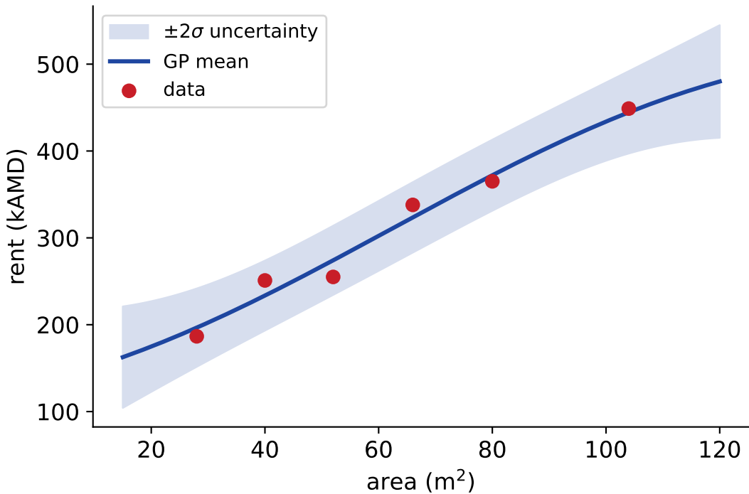
GP: band pinches at data, balloons away
