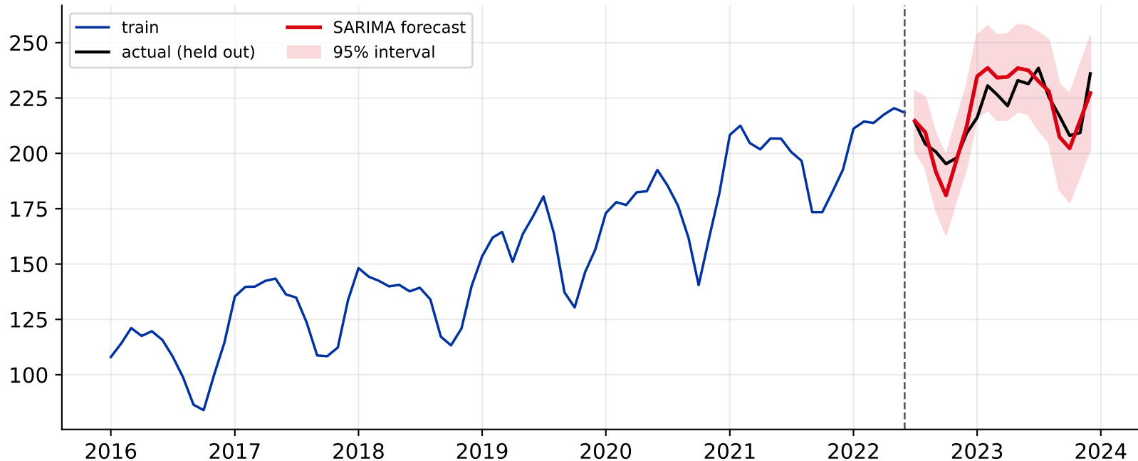
SARIMA(1,1,1)(1,1,0) 12 forecast
