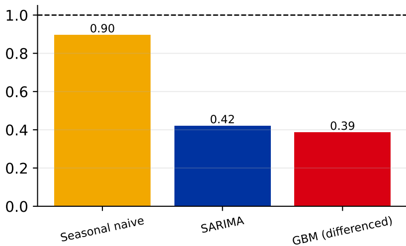
MASE (vs seasonal naive = 1.0)
