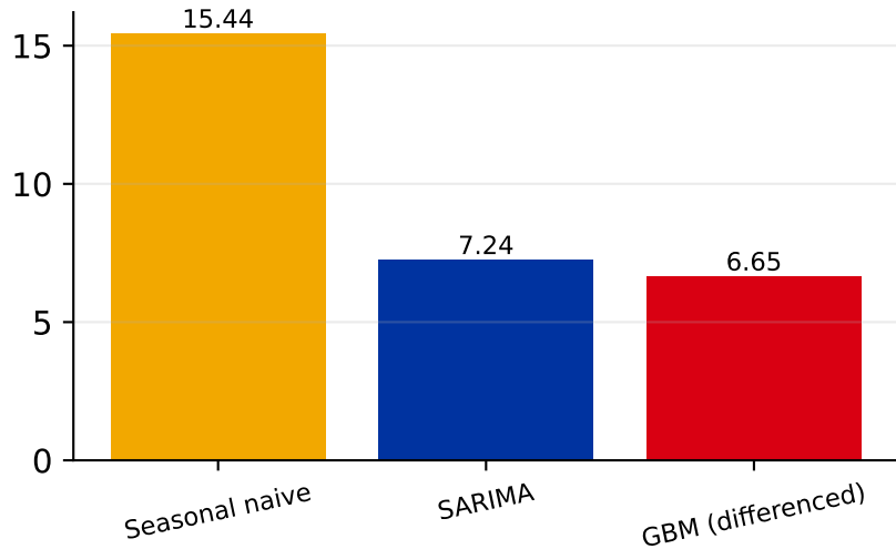
MAE (lower is better)
