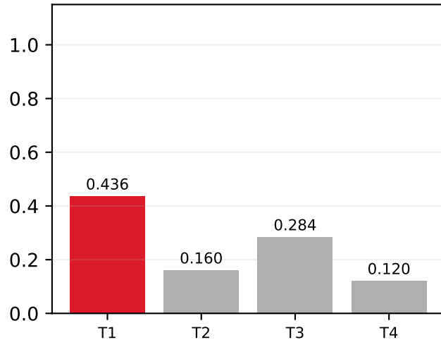
3. softmax of row I1 loss for this row = -\ln 0.436 = 0.83
