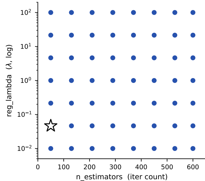
Grid - 56 pts (lattice)
