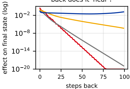
Before training: how far back does it 'hear'?
