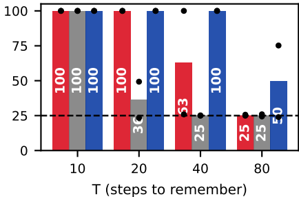
After training: recall the first token after T steps
