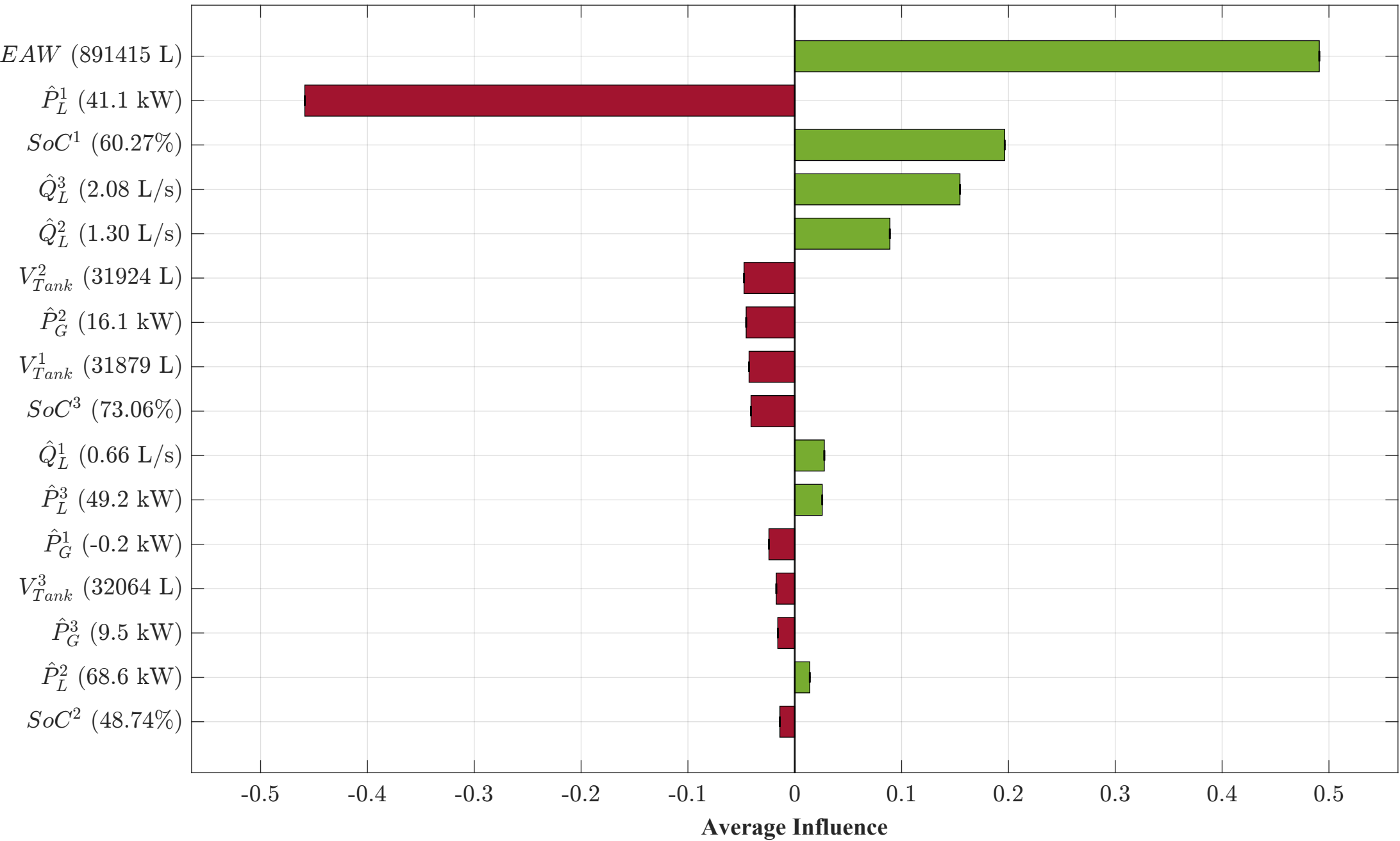
Scenario B: Aquifer Constraint Compliance MG3 — Day 4, 13:00 — Q_p^3 = -0.673 L/s (Pumping)
