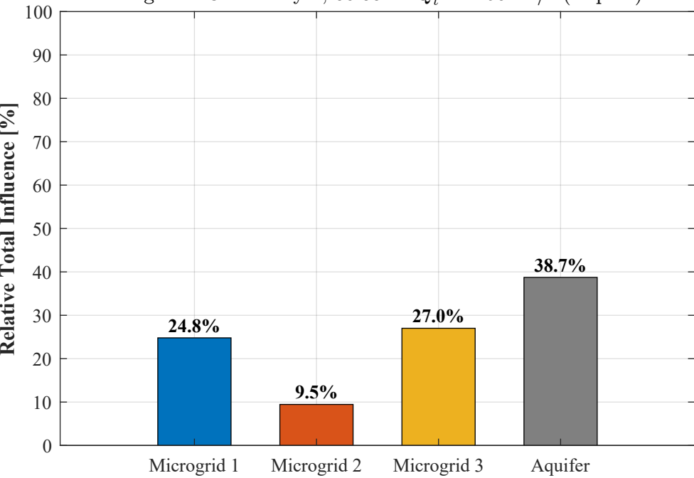
Interaction Analysis: Scenario B: Active Water Export Target: MG2 — Day 2, 08:00 — Q_t^2 = 2.561 L/s (Export)
