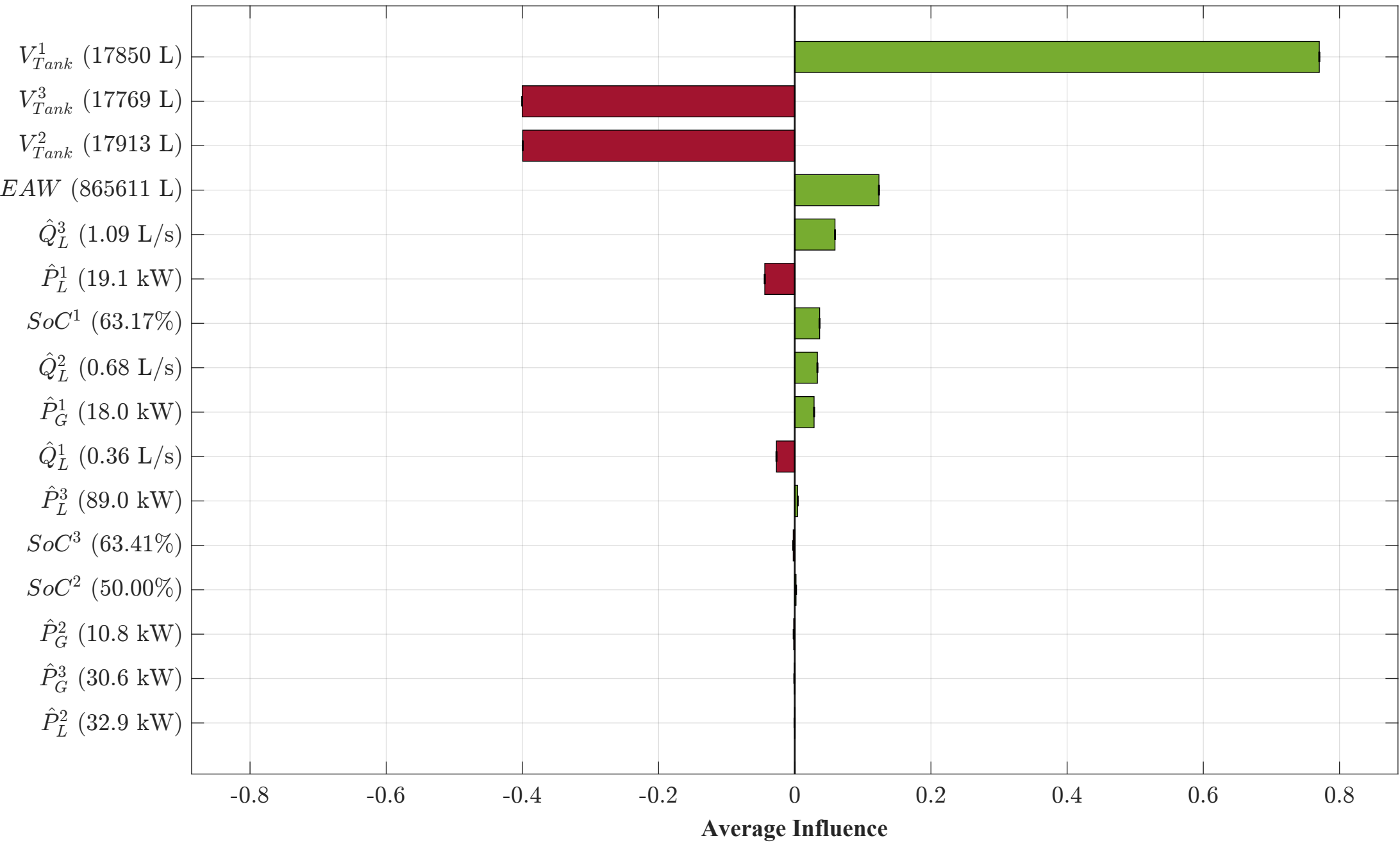
Scenario B: Active Water Export MG1 — Day 7, 07:30 — Q_t^1 = 2.324 L/s (Export)
