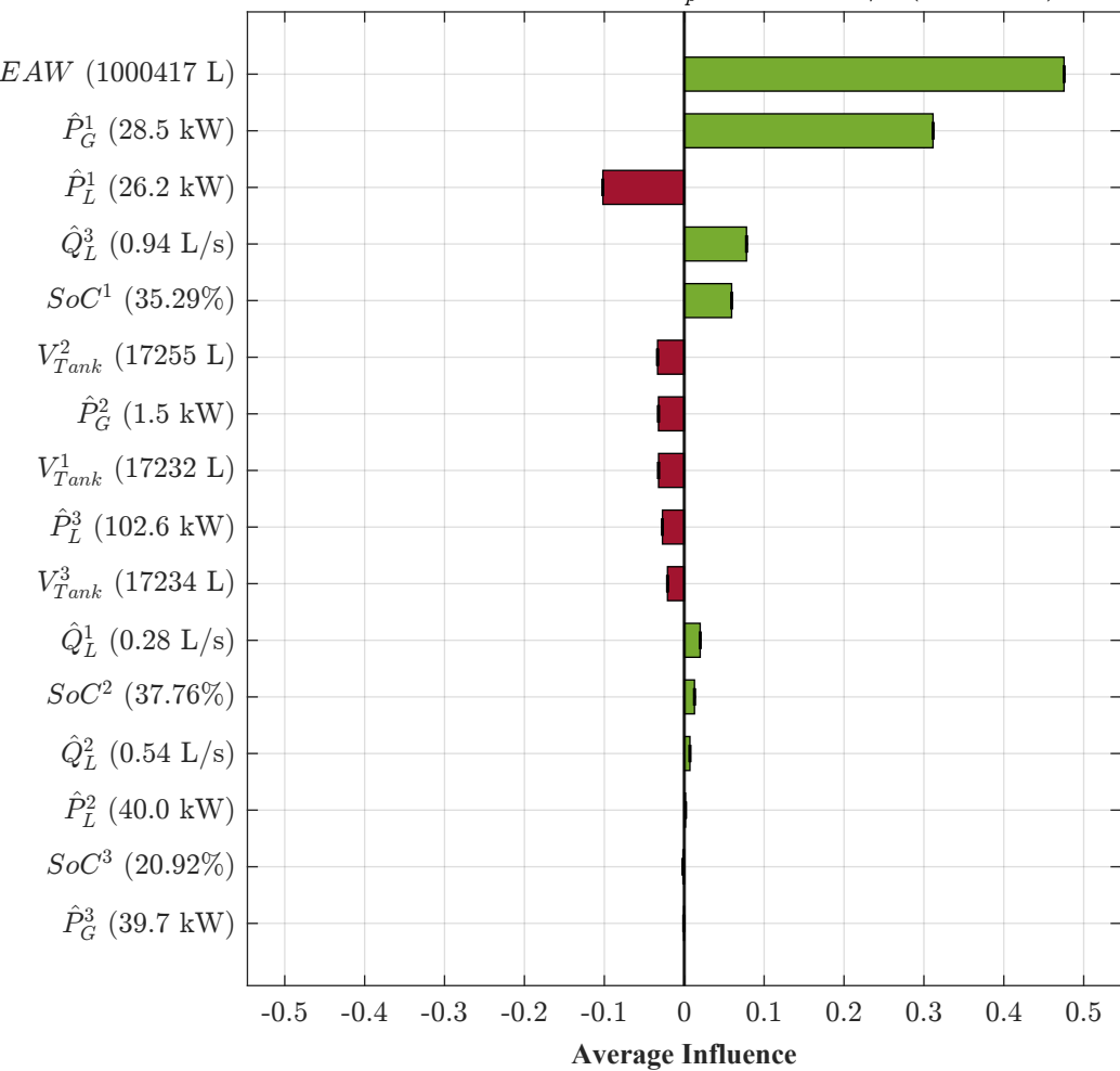
Scenario A: Energy Efficiency (Solar Pumping) MG3 — Day 1, 05:30 — Q_p^3 = -0.486 L/s (Pumping)
