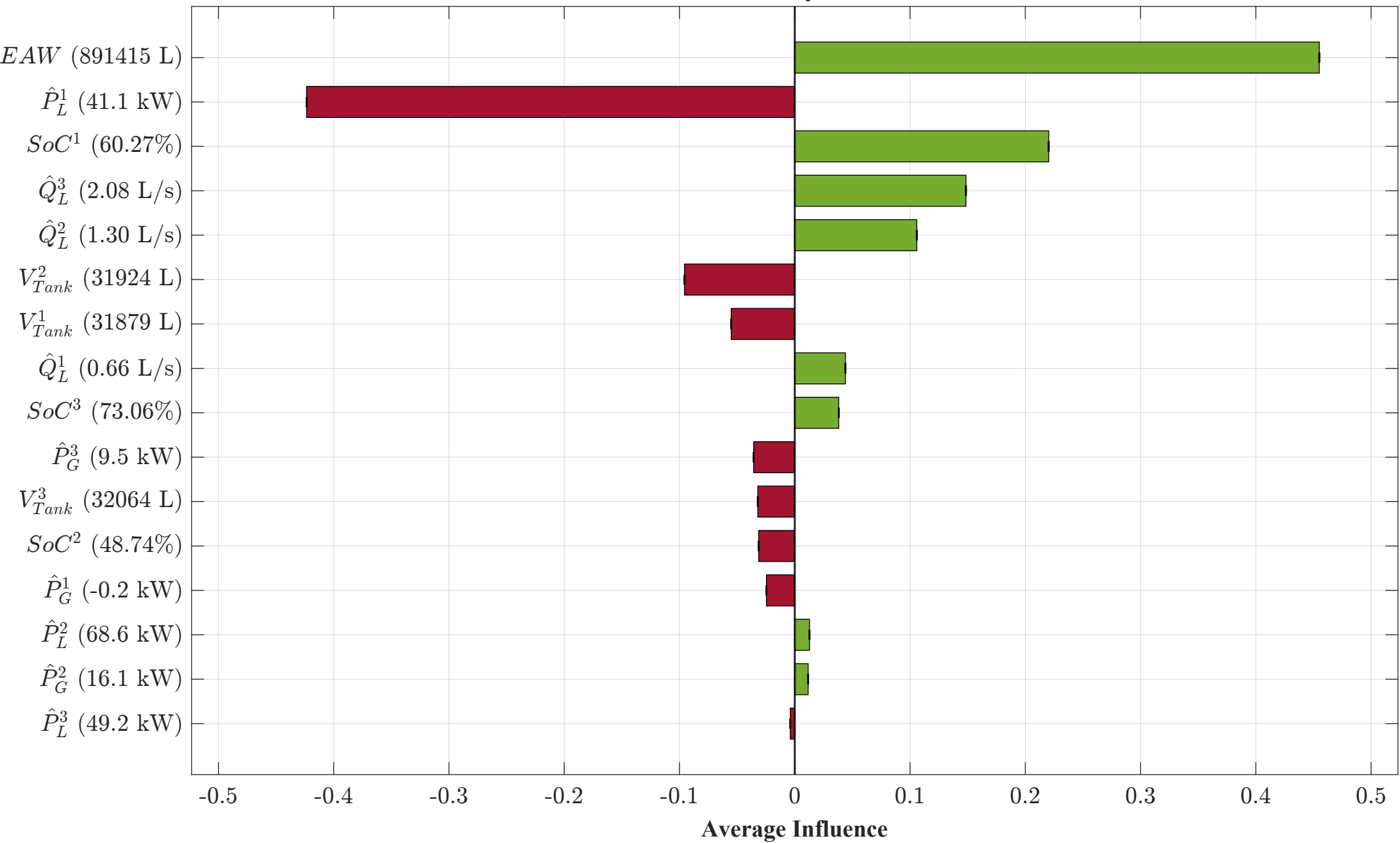
Scenario B: Aquifer Constraint Compliance MG2 — Day 4, 13:00 — Q_p^2 = 0.000 L/s (Pumping)
