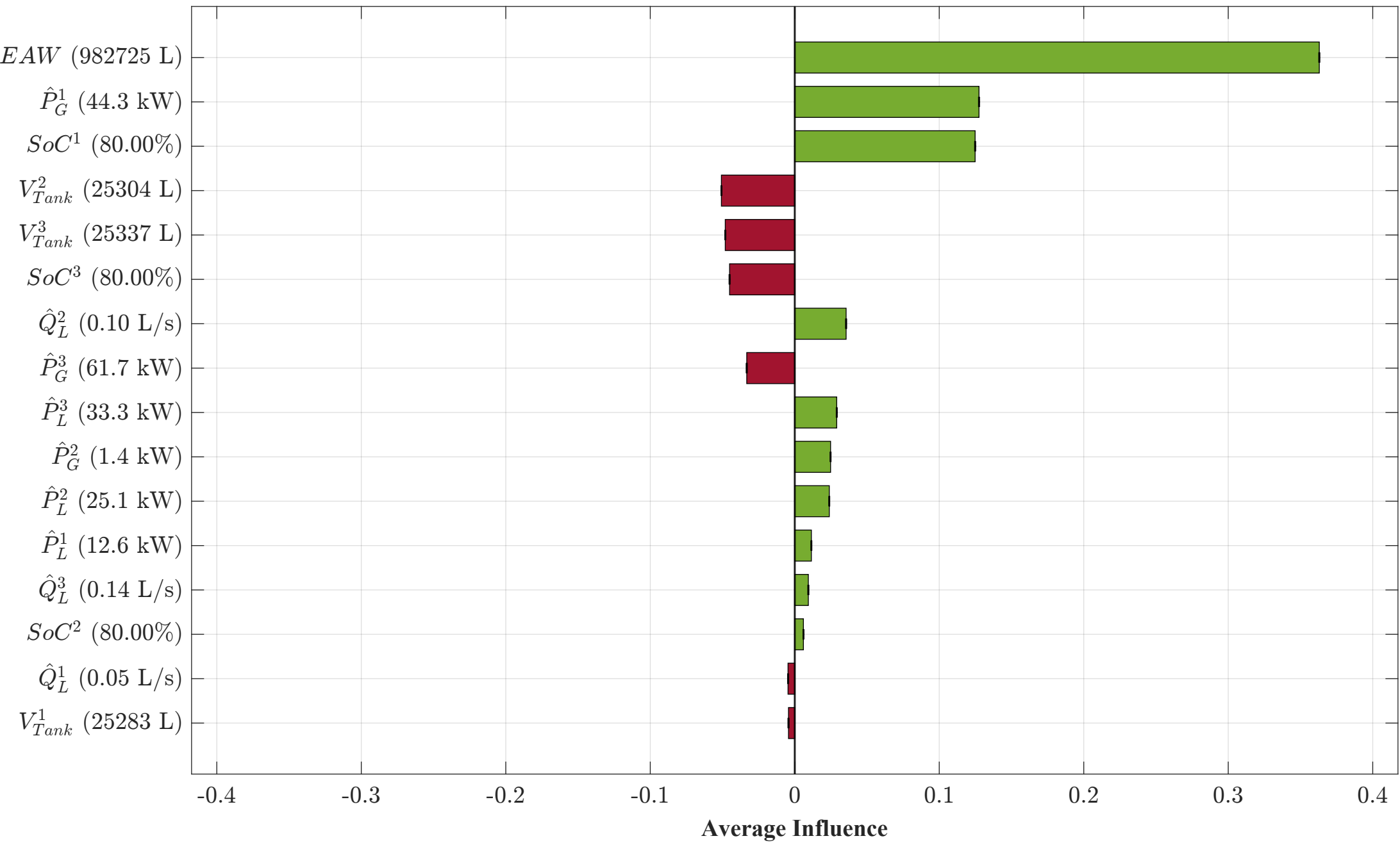
Scenario A: Global Peak Interaction MG2 — Day 2, 08:30 — Q_t^2 = 2.626 L/s (Export)
