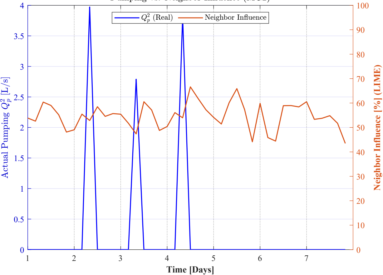
Pumping vs. Neighbor Influence (MG2)
