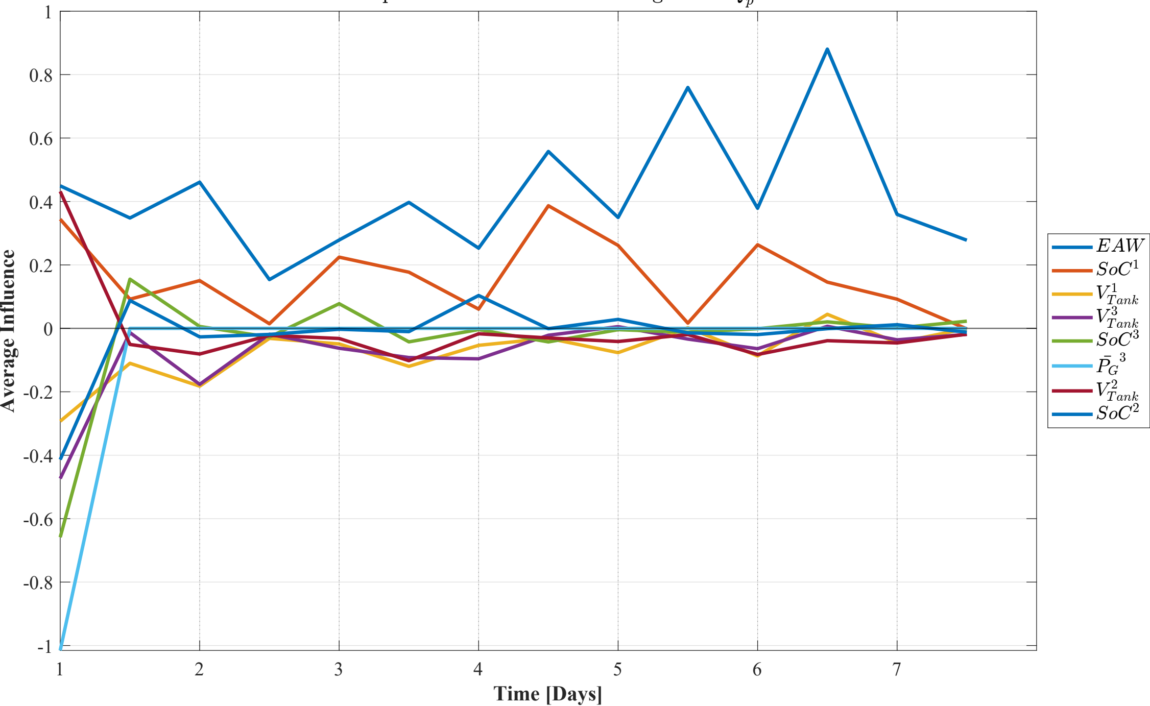
Temporal Evolution of LIME Weights for Q_p^3
