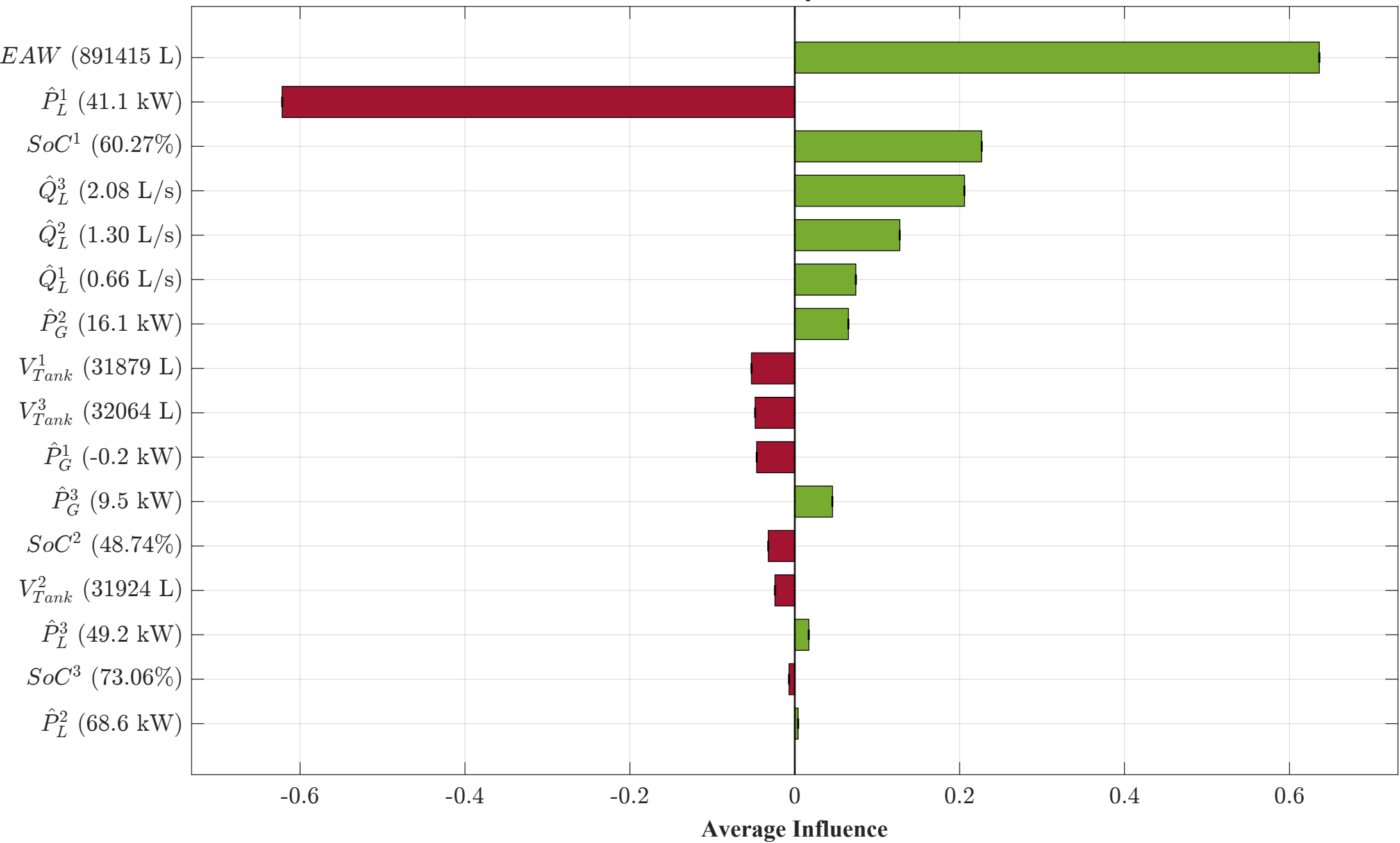
Scenario B: Aquifer Constraint Compliance MG3 — Day 4, 13:00 — Q_p^3 = 0.000 L/s (Pumping)
