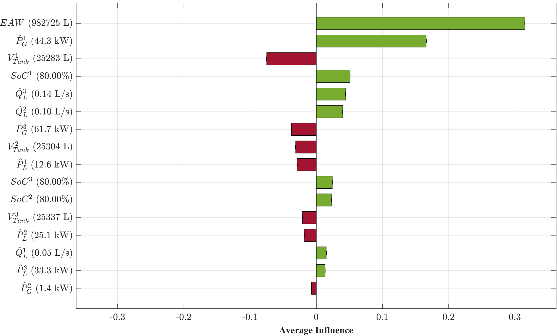
Scenario B: Active Water Export MG3 — Day 2, 08:30 — Q_t^3 = -1.626 L/s (Import)
