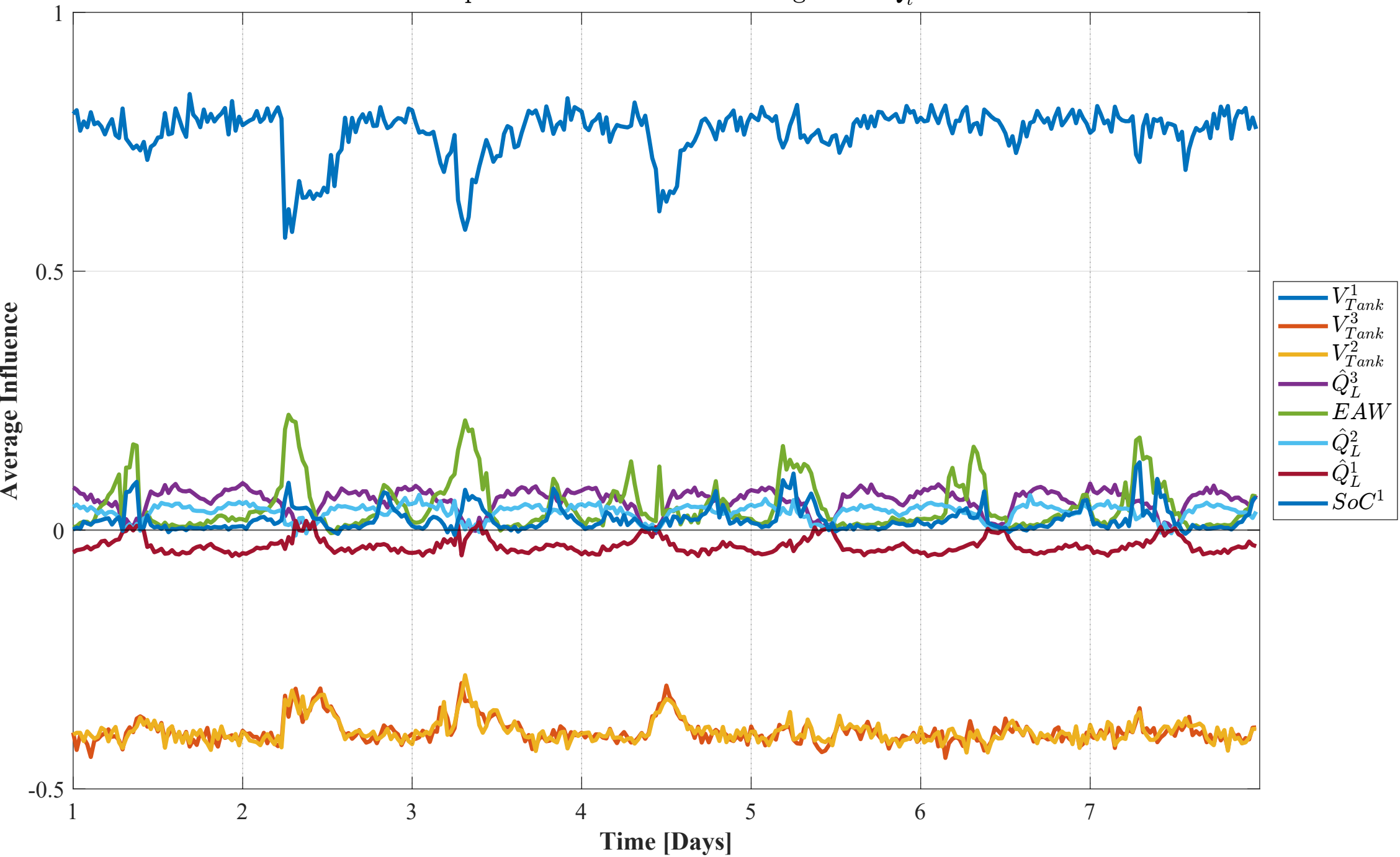
Temporal Evolution of LIME Weights for Q_t^1
