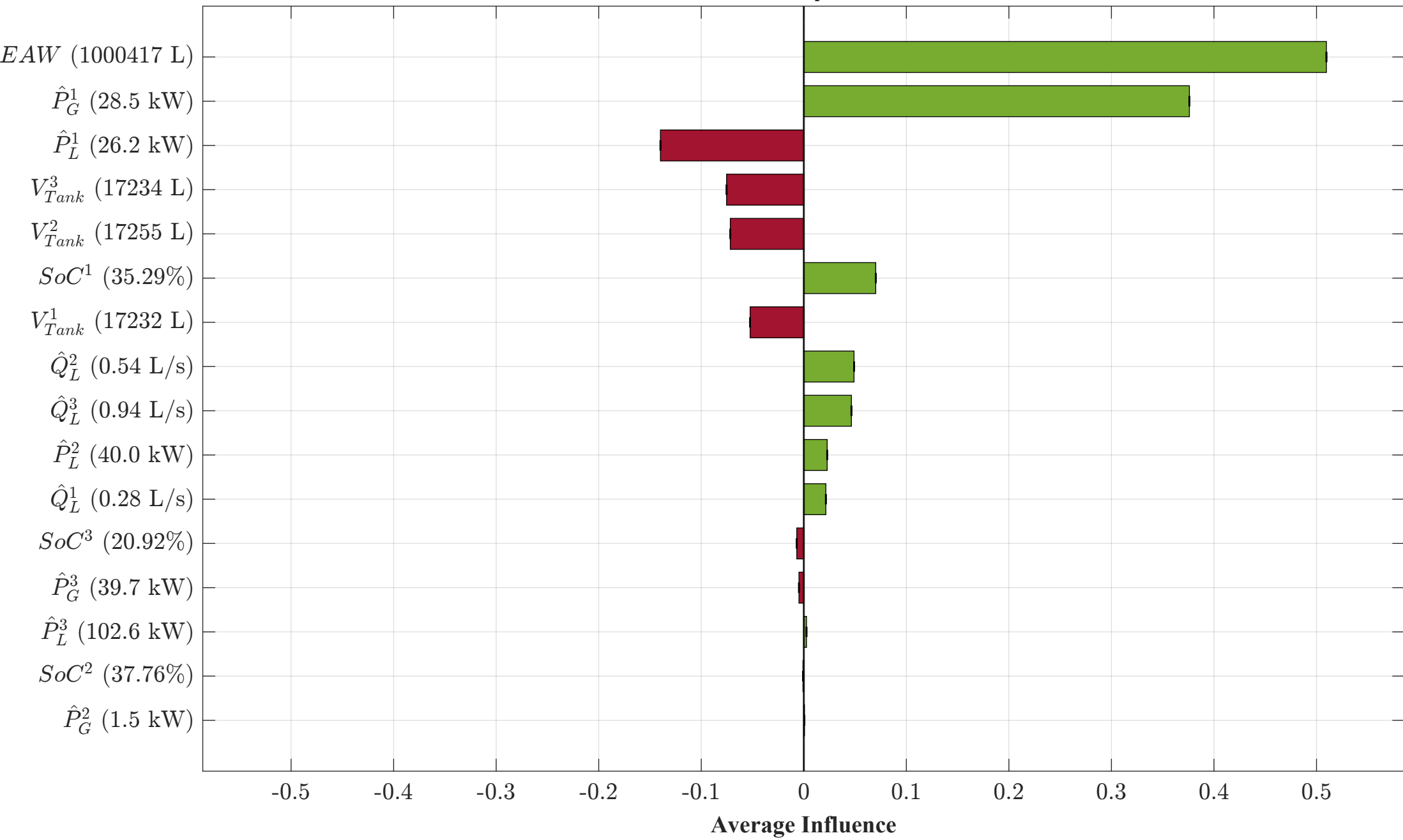
Scenario A: Energy Efficiency (Solar Pumping) MG3 — Day 1, 05:30 — Q_p^3 = 0.000 L/s (Pumping)
