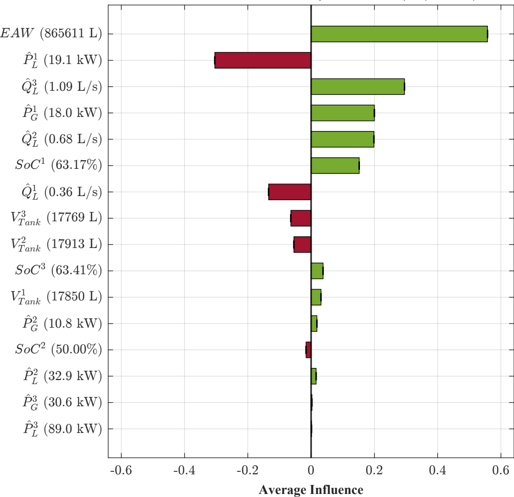
Scenario C: Direct Demand Satisfaction MG2 — Day 7, 07:30 — Q_t^2 = -0.928 L/s (Import)
