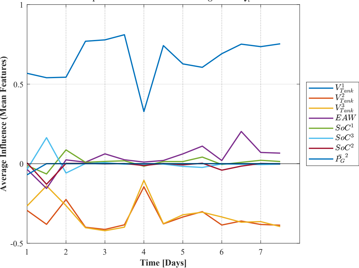
Temporal Evolution of LIME Weights for Q_t^1
