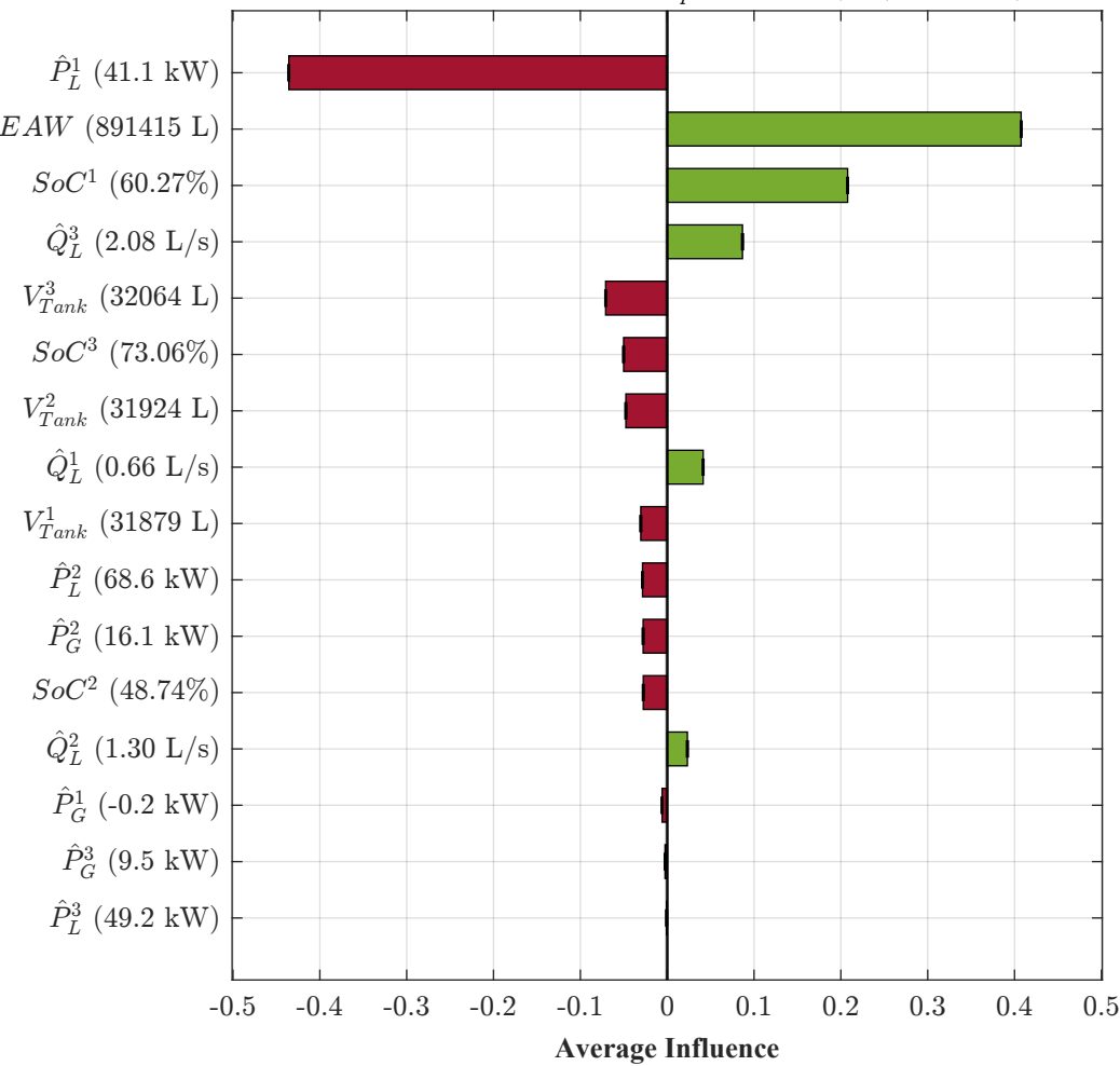
Scenario B: Aquifer Constraint Compliance MG1 — Day 4, 13:00 — Q_p^1 = 0.000 L/s (Pumping)
