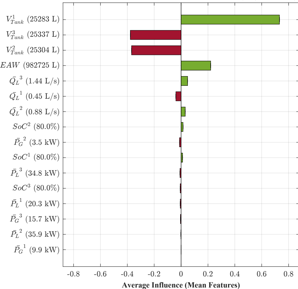
Mean-Feature Analysis: Scenario A: Global Peak Interaction Target: MG1 — Day 2, 08:30 — Q_t^1 = -1.00 L/s (Importing)
