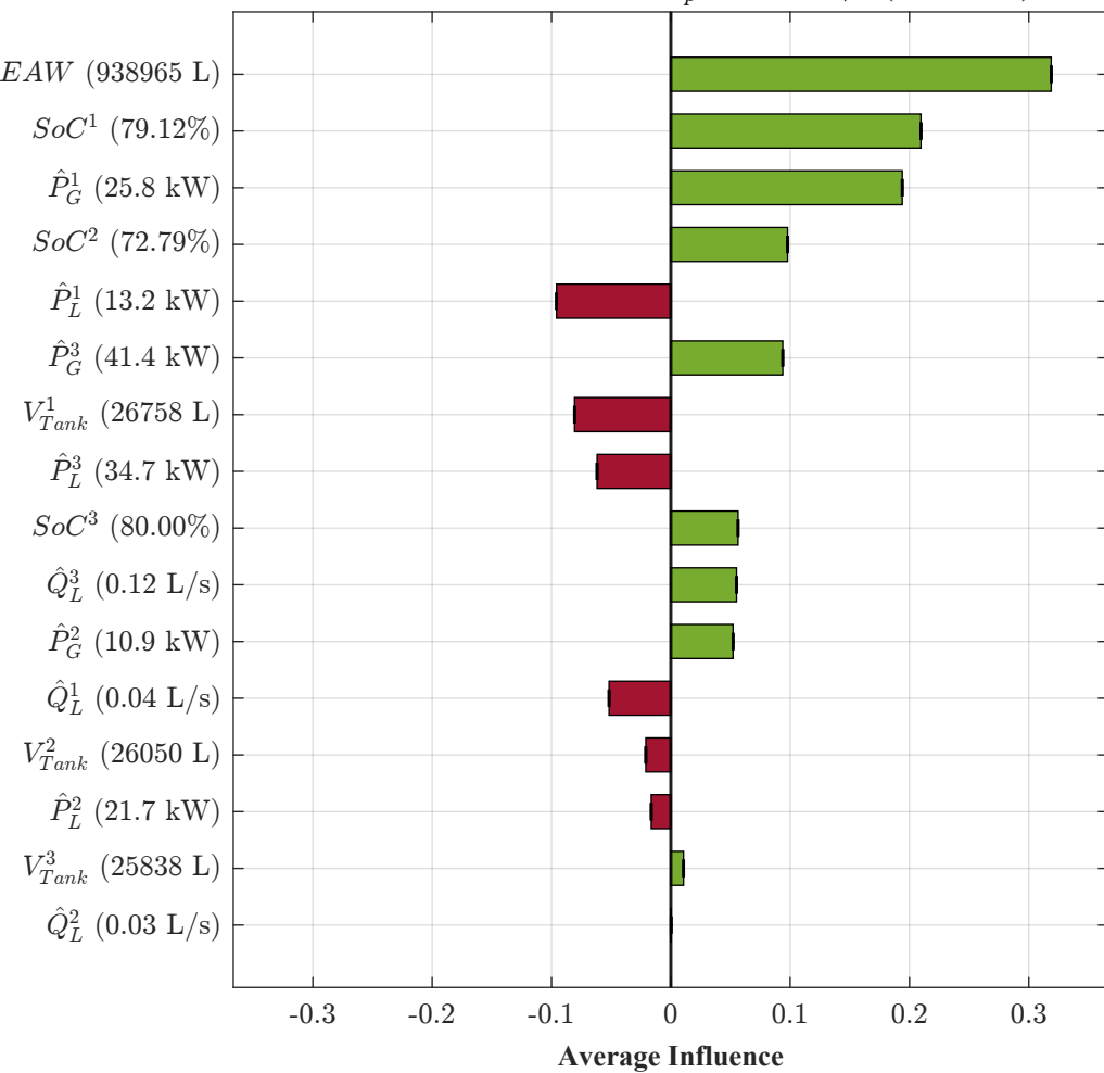
Scenario A: Energy Efficiency (Solar Pumping) MG1 — Day 3, 10:00 — Q_p^1 = 1.779 L/s (Pumping)
