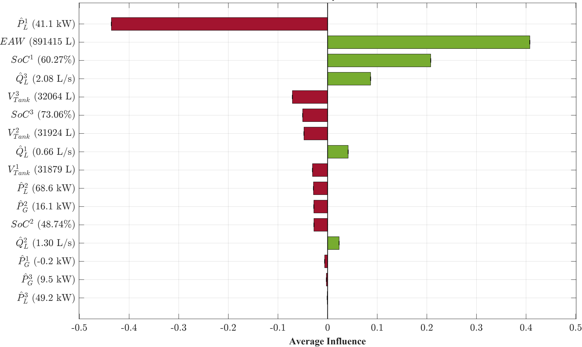
Scenario B: Aquifer Constraint Compliance MG1 — Day 4, 13:00 — Q_p^1 = 0.000 L/s (Pumping)
