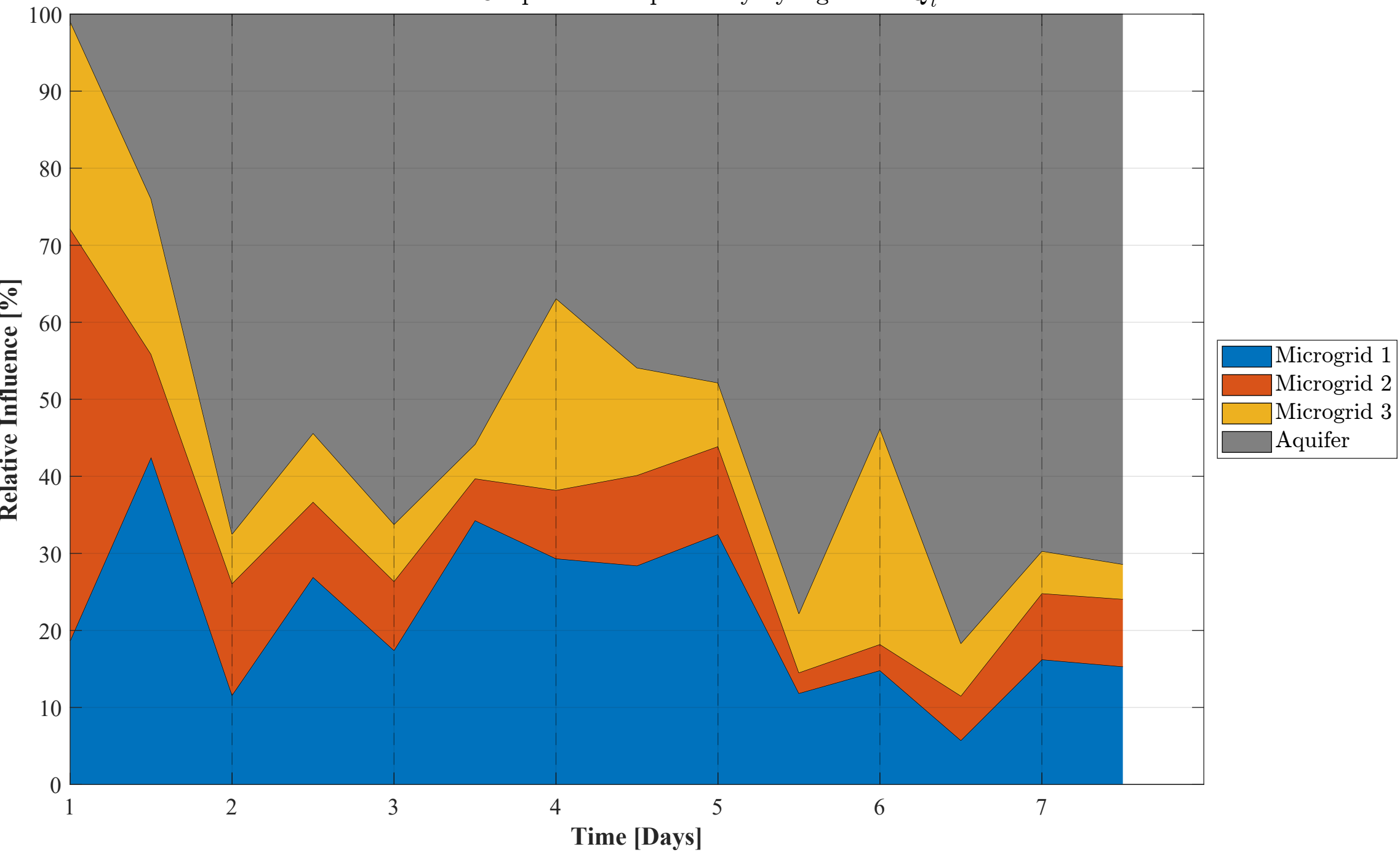
Evolution of Cooperative Dependency by Agent for Q_t^3
