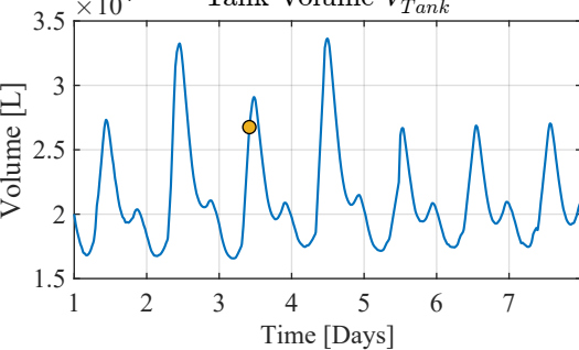
Tank Volume V_{Tank}^1
