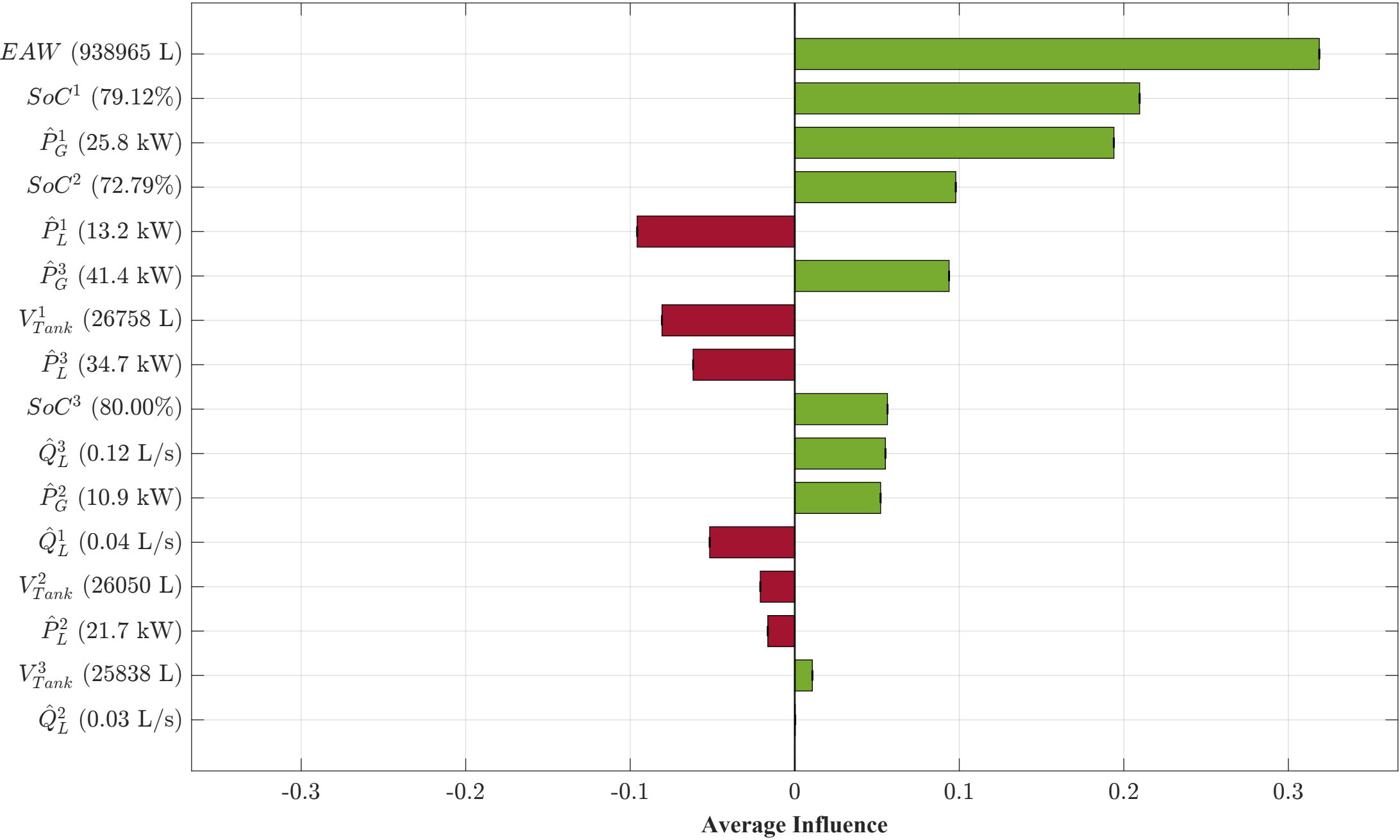
Scenario A: Energy Efficiency (Solar Pumping) MG1 — Day 3, 10:00 — Q_p^1 = 1.779 L/s (Pumping)
