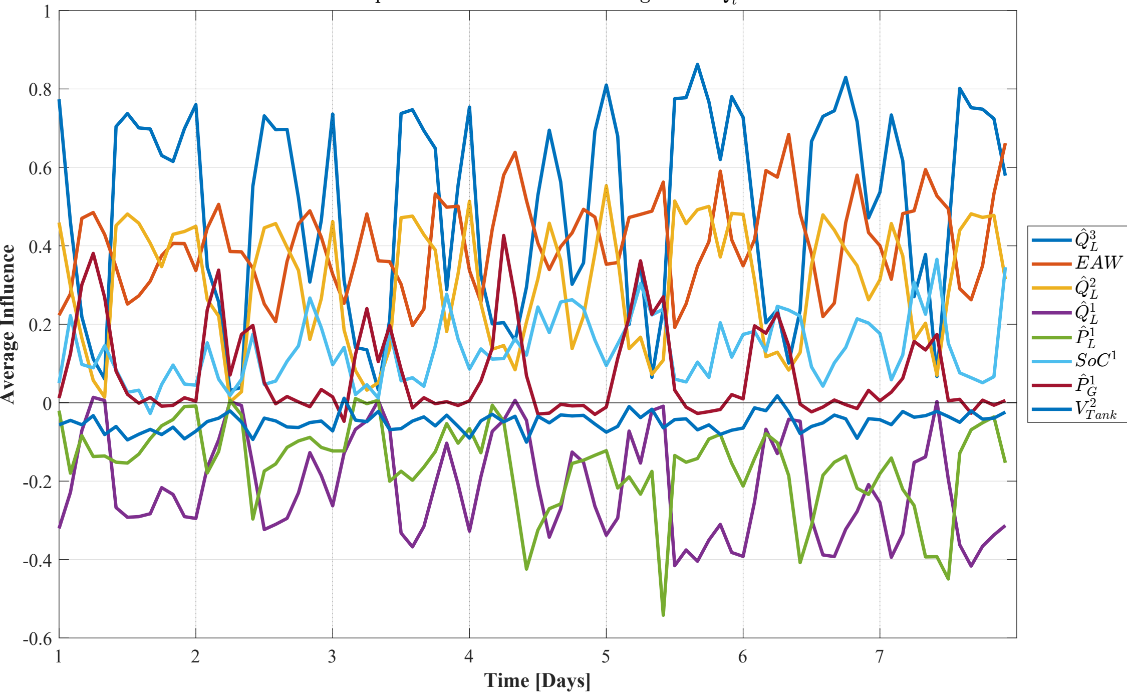
Temporal Evolution of LIME Weights for Q_t^3
