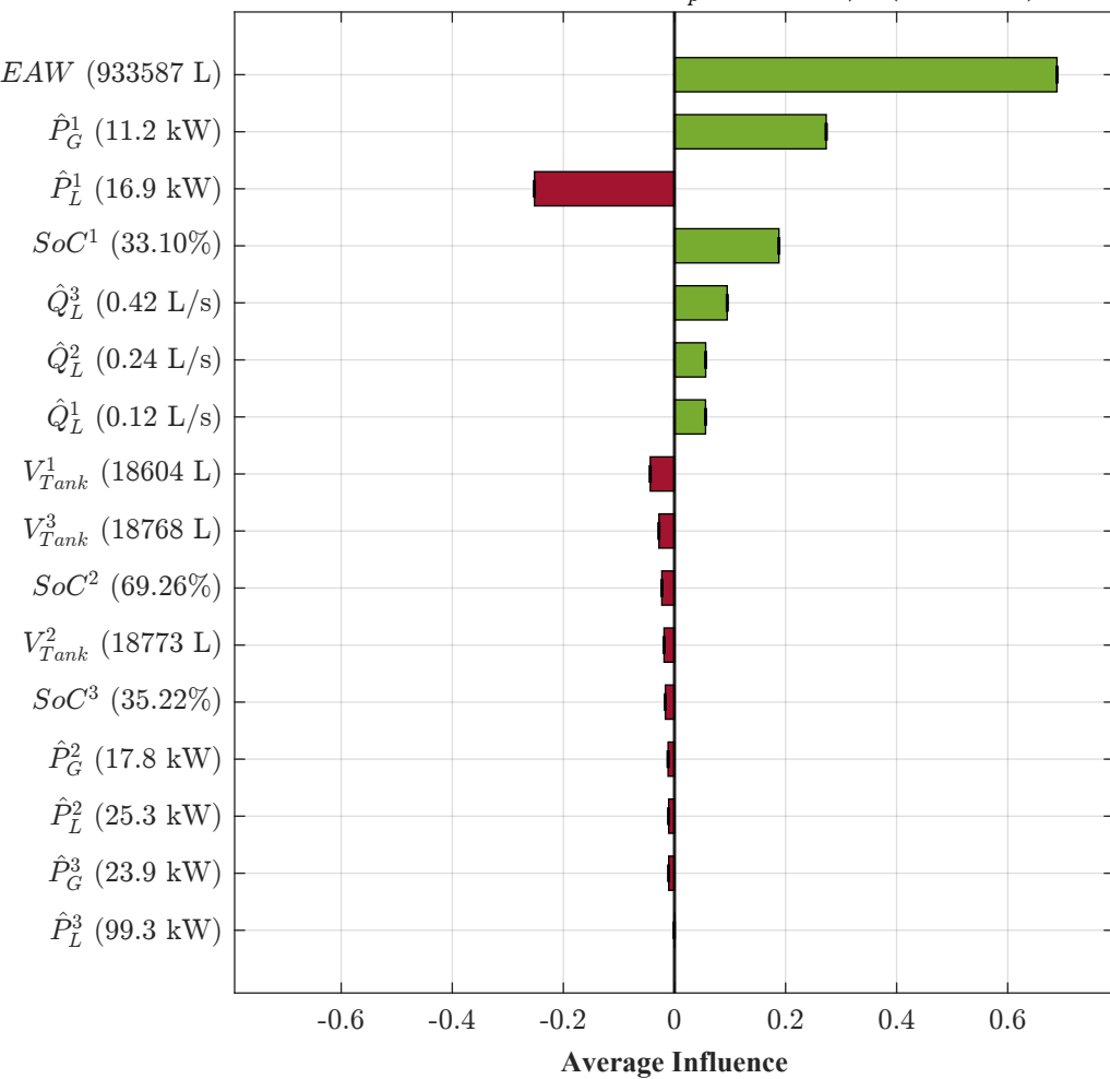
Scenario A: Energy Efficiency (Solar Pumping) MG2 — Day 4, 08:00 — Q_p^2 = 3.816 L/s (Pumping)
