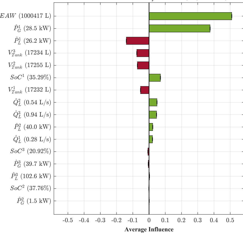
Scenario A: Energy Efficiency (Solar Pumping) MG3 — Day 1, 05:30 — Q_p^3 = 0.000 L/s (Pumping)
