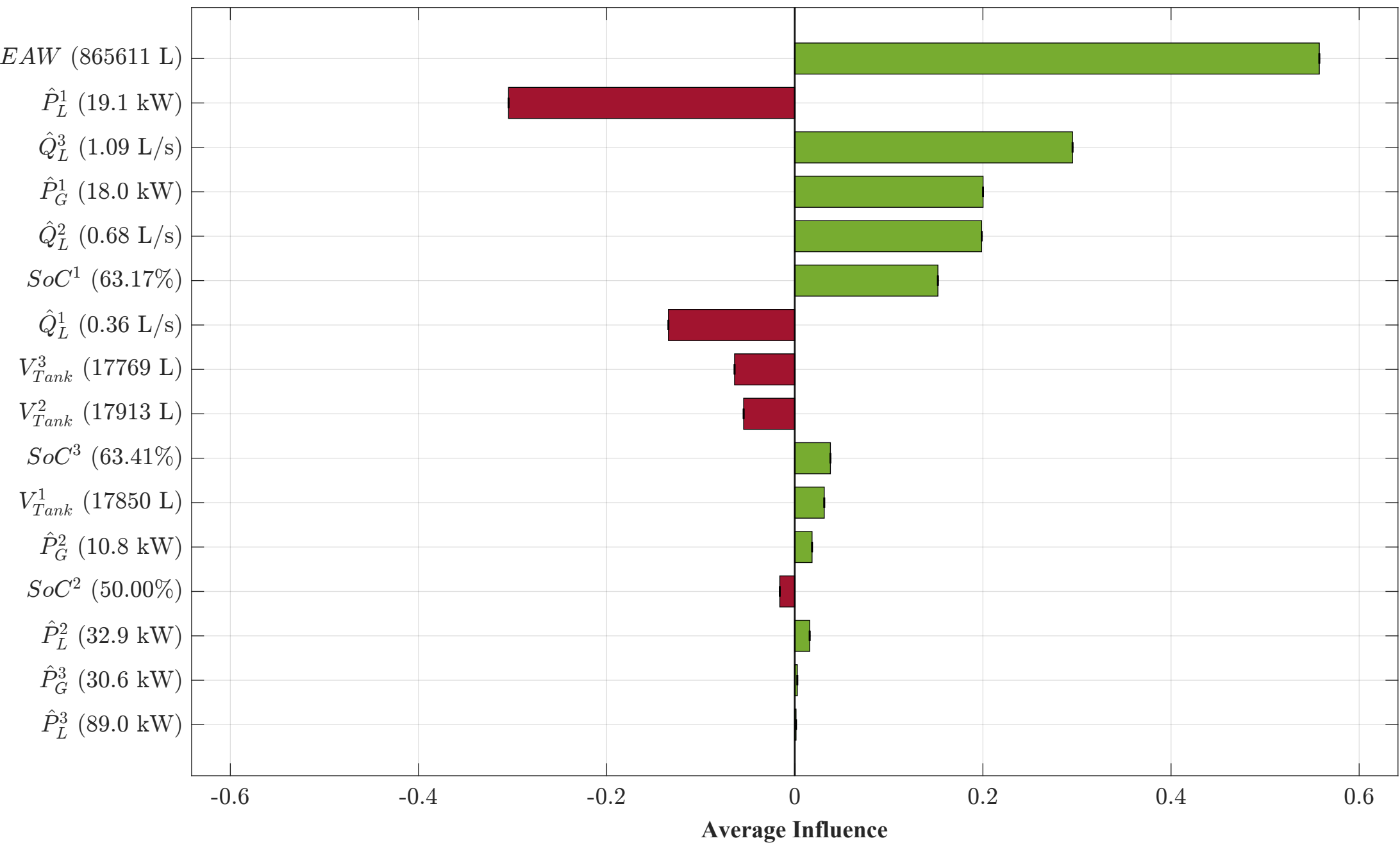
Scenario C: Direct Demand Satisfaction MG2 — Day 7, 07:30 — Q_t^2 = -0.928 L/s (Import)
