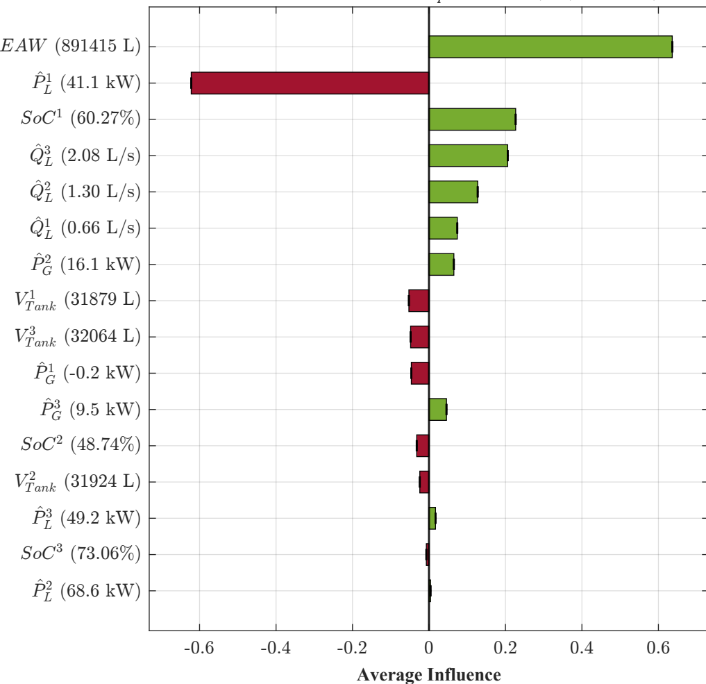
Scenario B: Aquifer Constraint Compliance MG3 — Day 4, 13:00 — Q_p^3 = 0.000 L/s (Pumping)
