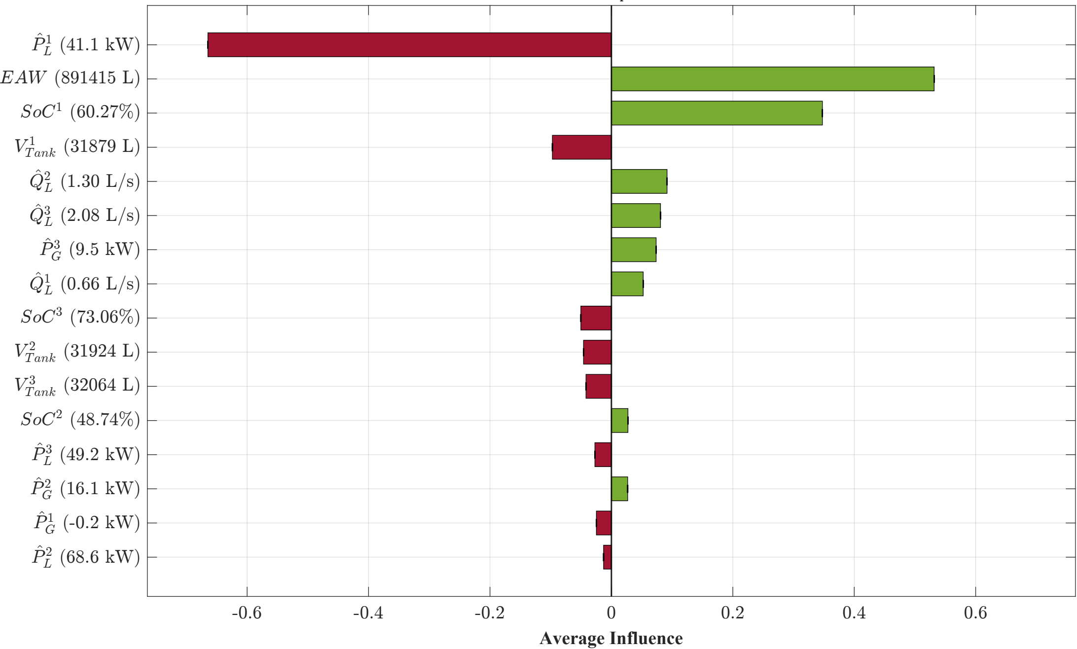
Scenario B: Aquifer Constraint Compliance MG2 — Day 4, 13:00 — Q_p^2 = 0.028 L/s (Pumping)
