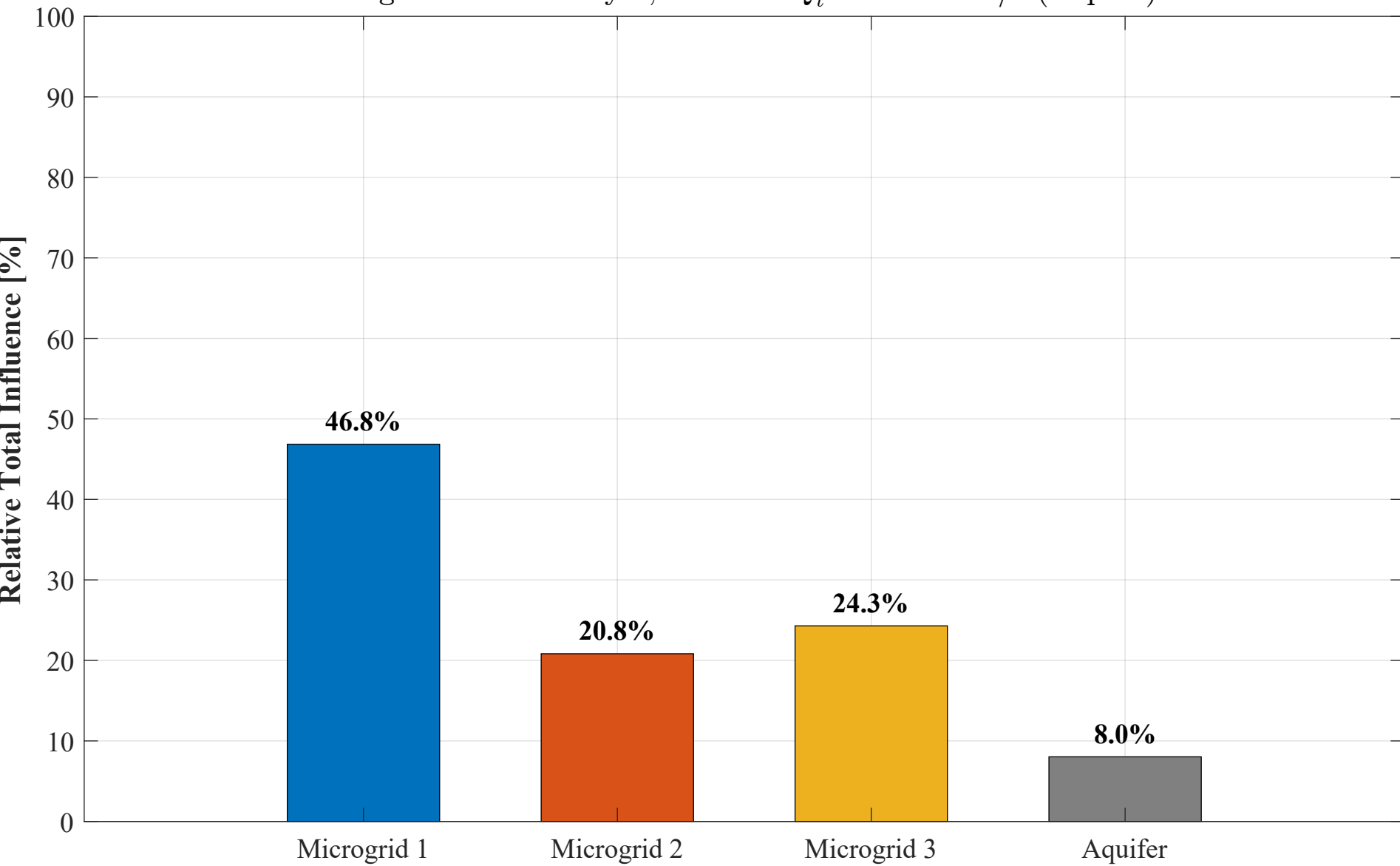
Interaction Analysis: Scenario A: Global Peak Interaction Target: MG1 — Day 2, 08:30 — Q_t^1 = -1.000 L/s (Export)
