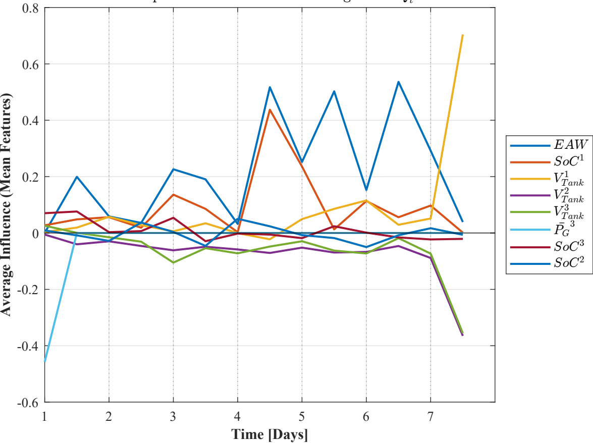
Temporal Evolution of LIME Weights for Q_t^2
