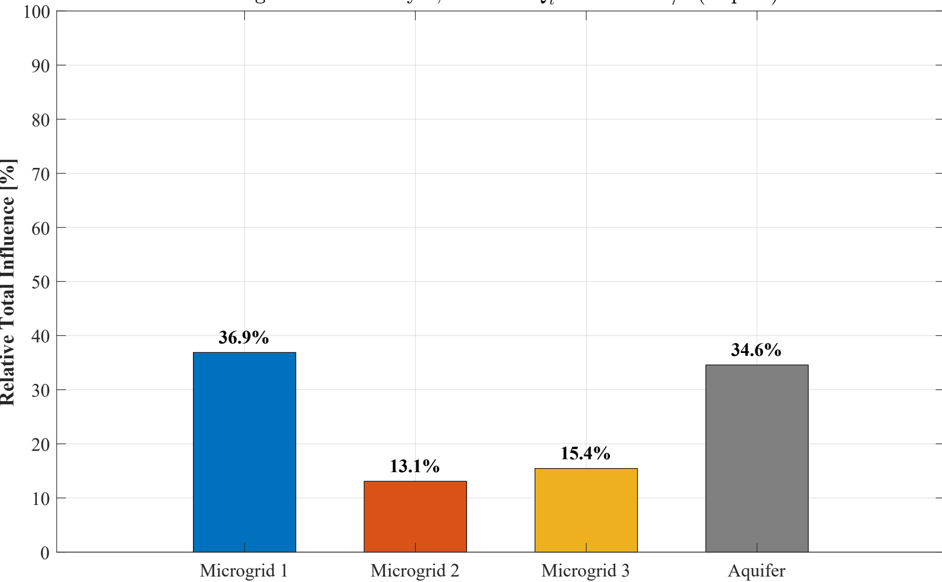
Interaction Analysis: Scenario B: Active Water Export Target: MG3 — Day 2, 08:30 — Q_t^3 = -1.626 L/s (Export)
