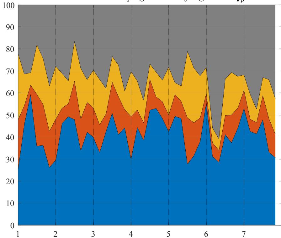
Evolution of Pumping Drivers by Agent for Q_p^1
