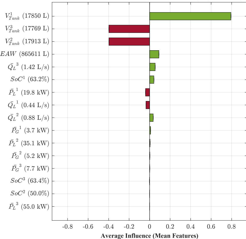
Mean-Feature Analysis: Scenario B: Active Water Export Target: MG1 — Day 7, 07:30 — Q_t^1 = 2.32 L/s (Exporting)
