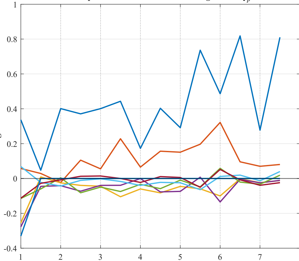
Temporal Evolution of LIME Weights for Q_p^3
