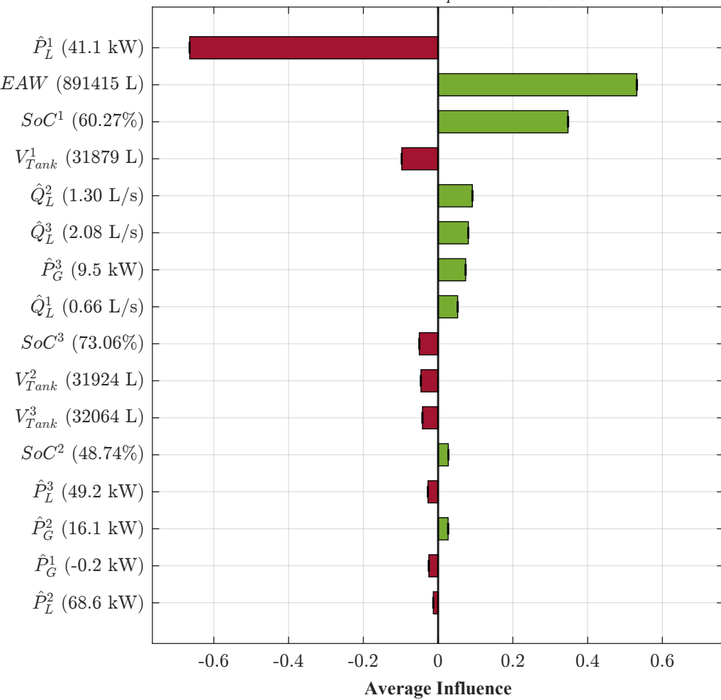
Scenario B: Aquifer Constraint Compliance MG2 — Day 4, 13:00 — Q_p^2 = 0.028 L/s (Pumping)
