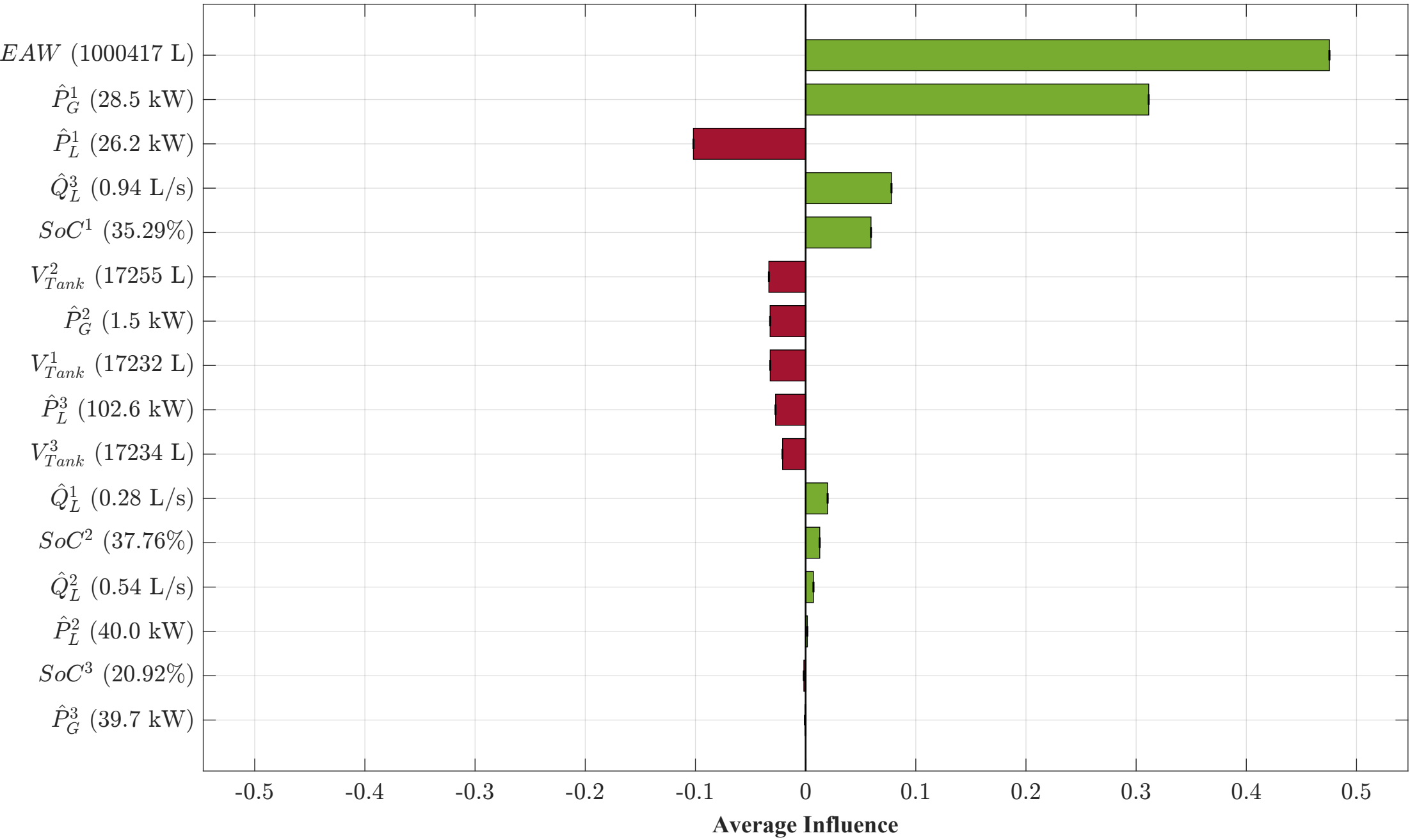
Scenario A: Energy Efficiency (Solar Pumping) MG3 — Day 1, 05:30 — Q_p^3 = -0.486 L/s (Pumping)
