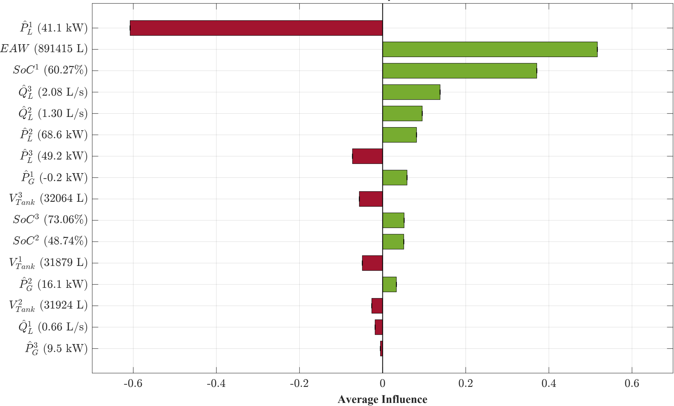
Scenario B: Aquifer Constraint Compliance MG1 — Day 4, 13:00 — Q_p^1 = 0.644 L/s (Pumping)
