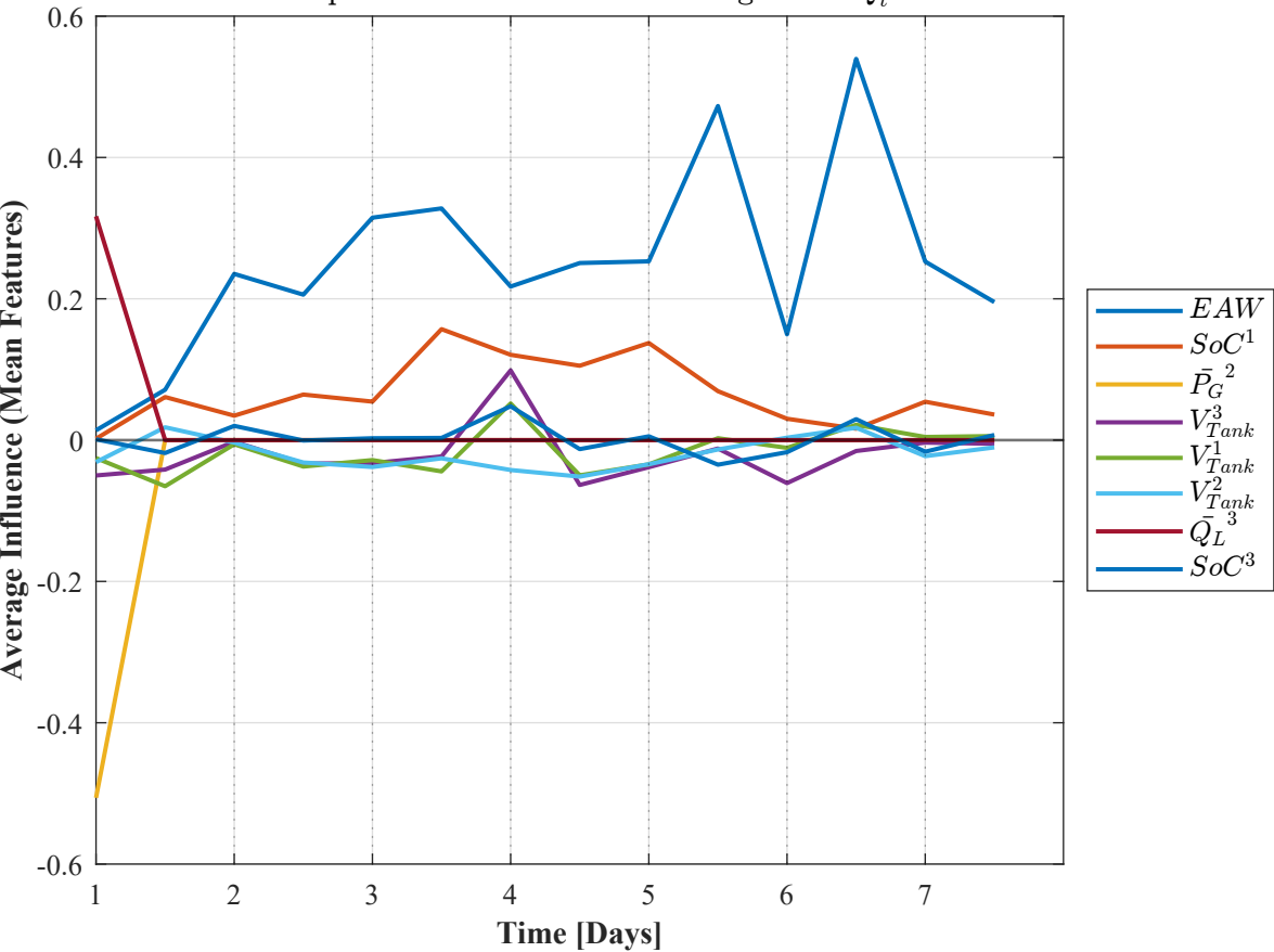
Temporal Evolution of LIME Weights for Q_t^3
