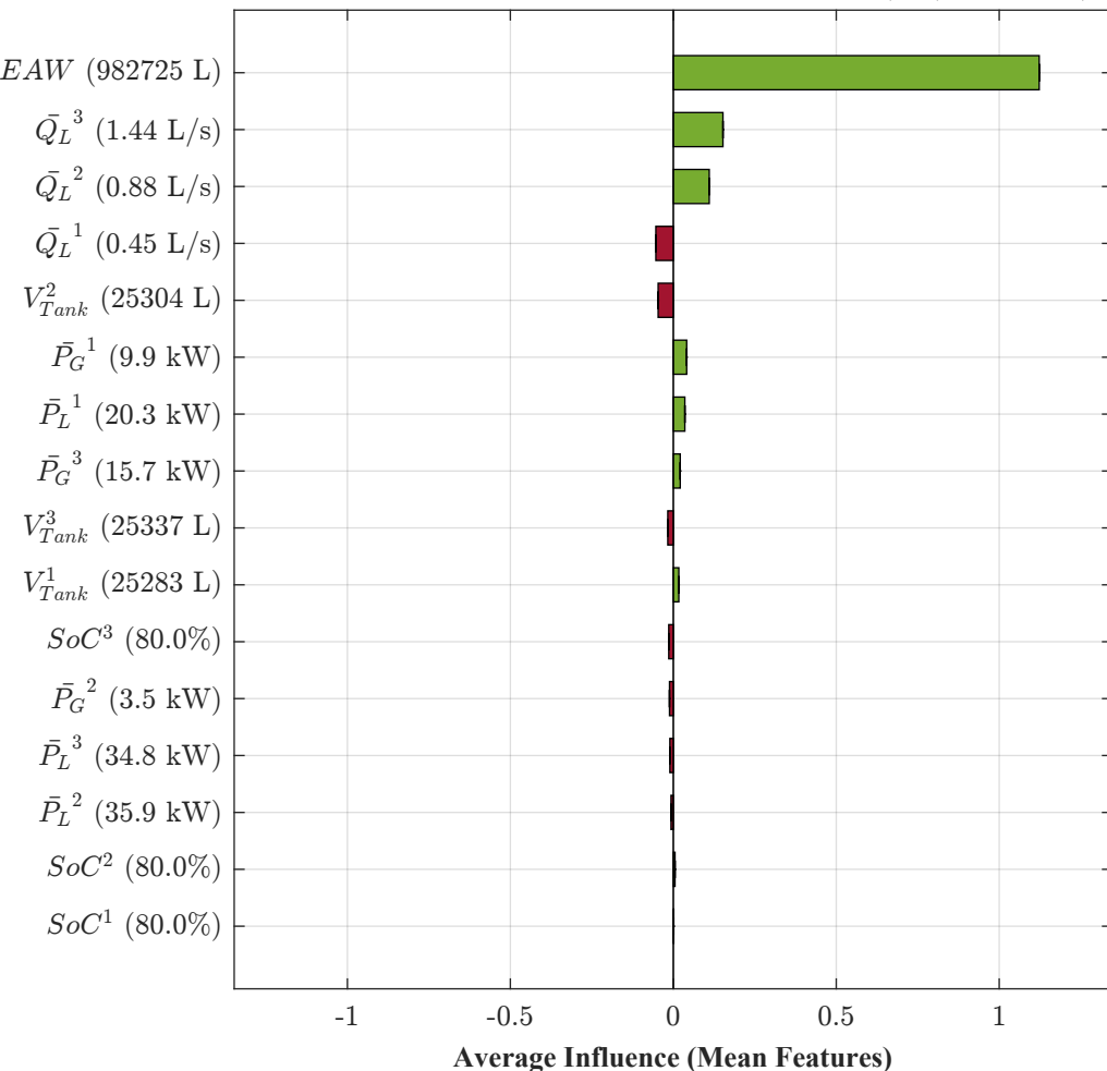
Mean-Feature Analysis: Scenario A: Global Peak Interaction Target: MG2 — Day 2, 08:30 — Q_t^2 = 2.63 L/s (Exporting)
