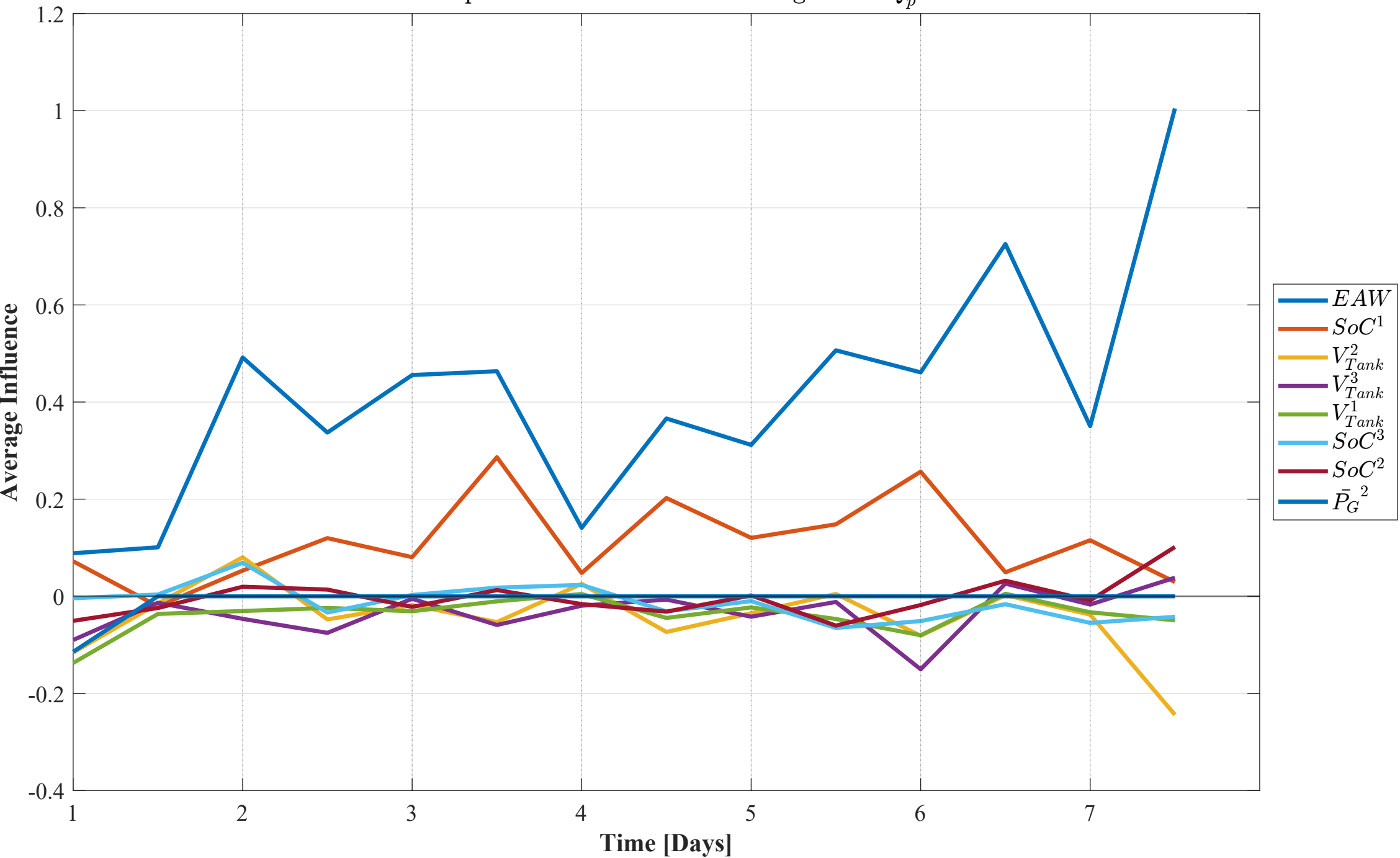
Temporal Evolution of LIME Weights for Q_p^1
