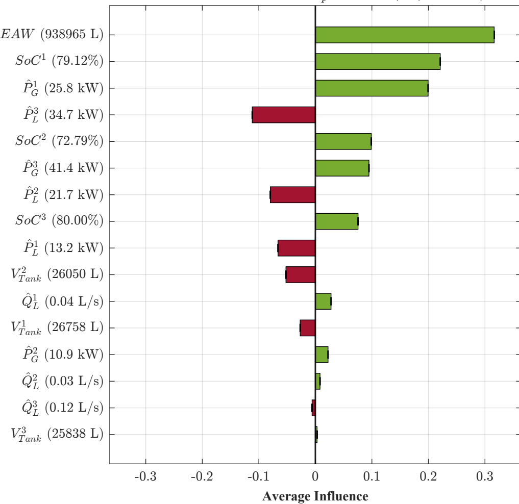
Scenario A: Energy Efficiency (Solar Pumping) MG1 — Day 3, 10:00 — Q_p^1 = 2.205 L/s (Pumping)
