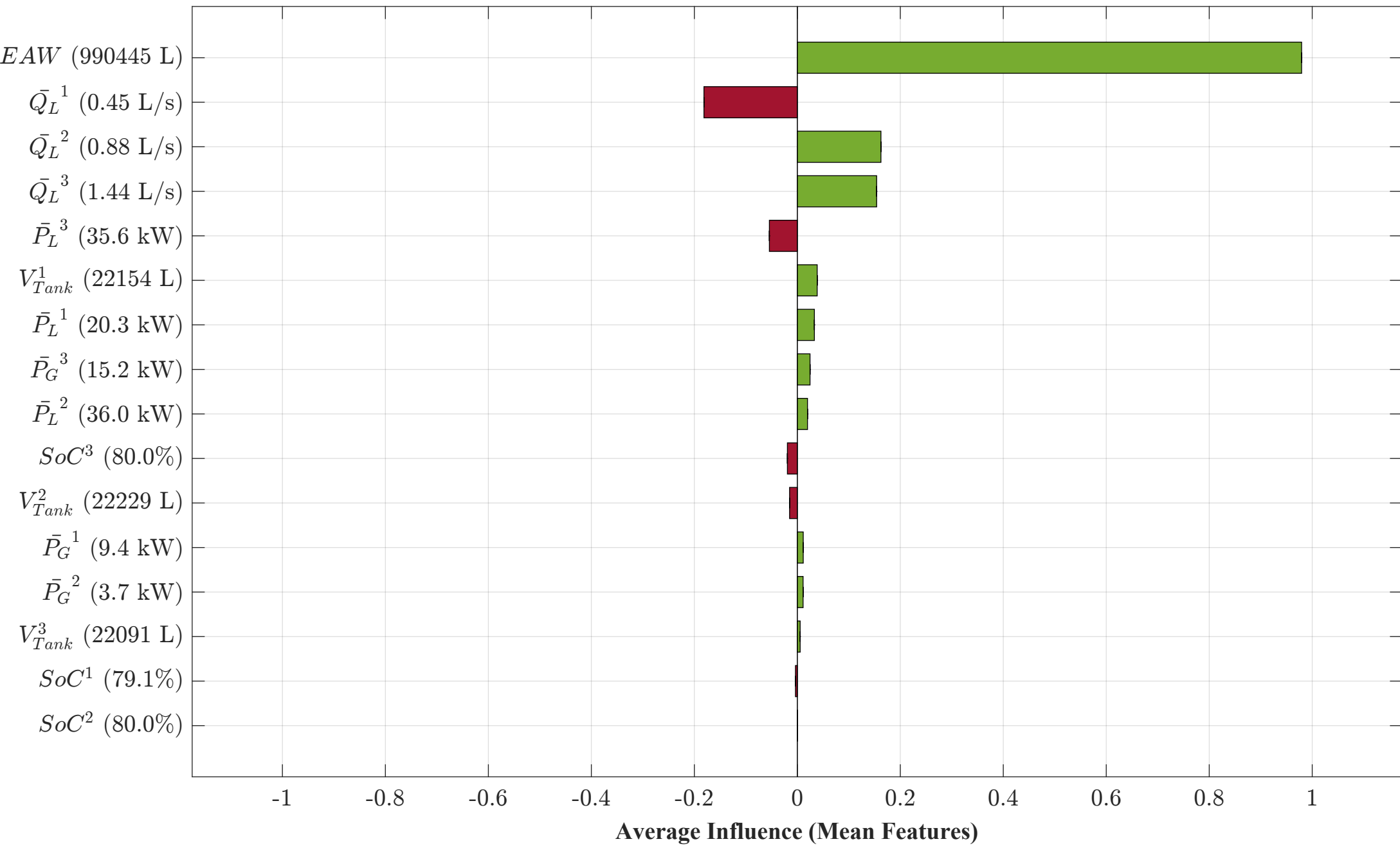
Mean-Feature Analysis: Scenario B: Active Water Export Target: MG2 — Day 2, 08:00 — Q_t^2 = 2.56 L/s (Exporting)
