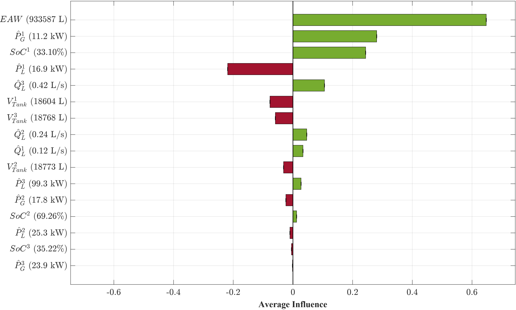
Scenario A: Energy Efficiency (Solar Pumping) MG2 — Day 4, 08:00 — Q_p^2 = 2.446 L/s (Pumping)
