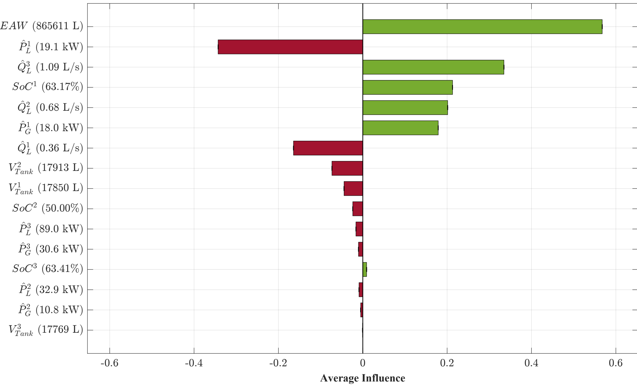
Scenario C: Direct Demand Satisfaction MG3 — Day 7, 07:30 — Q_t^3 = -1.396 L/s (Import)
