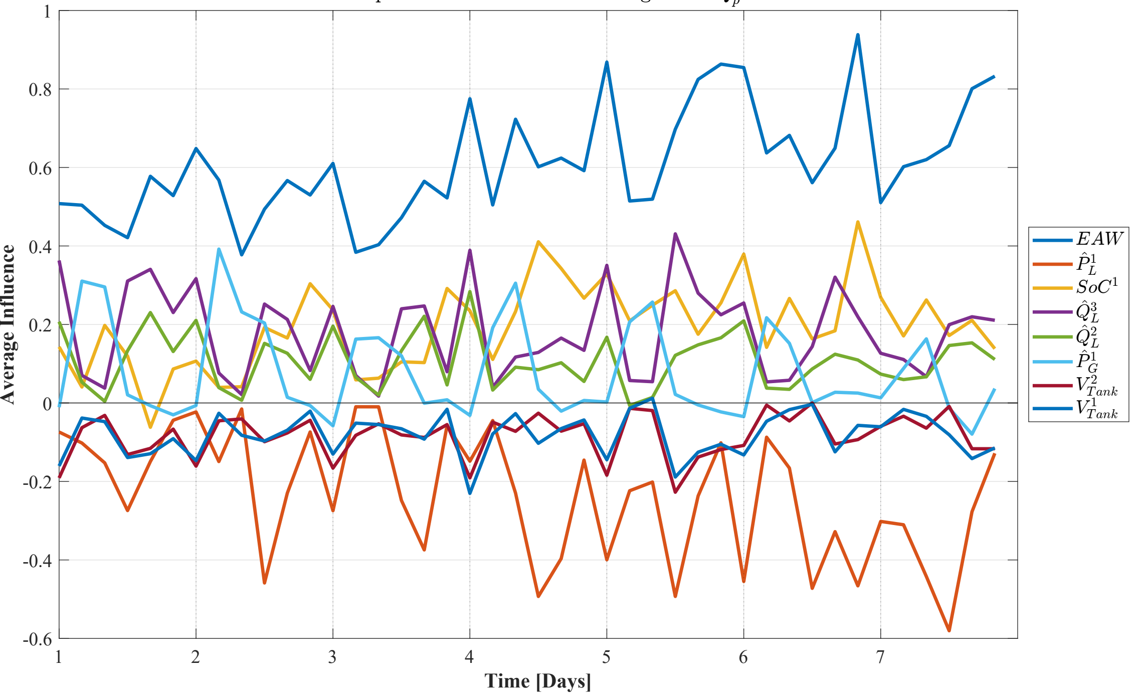
Temporal Evolution of LIME Weights for Q_p^3
