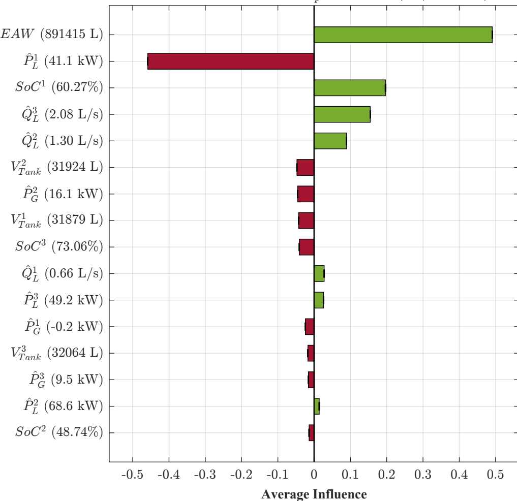
Scenario B: Aquifer Constraint Compliance MG3 — Day 4, 13:00 — Q_p^3 = -0.673 L/s (Pumping)
