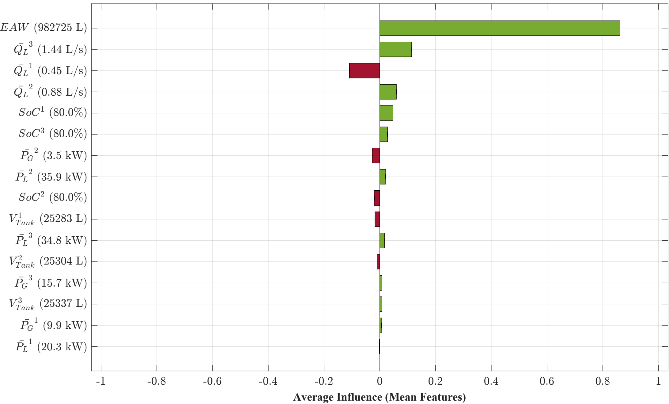
Mean-Feature Analysis: Scenario B: Active Water Export Target: MG3 — Day 2, 08:30 — Q_t^3 = -1.63 L/s (Importing)
