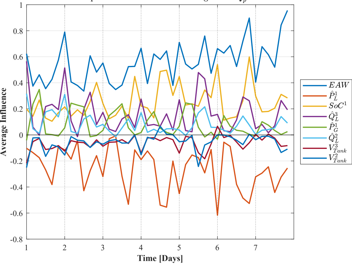
Temporal Evolution of LIME Weights for Q_p^1
