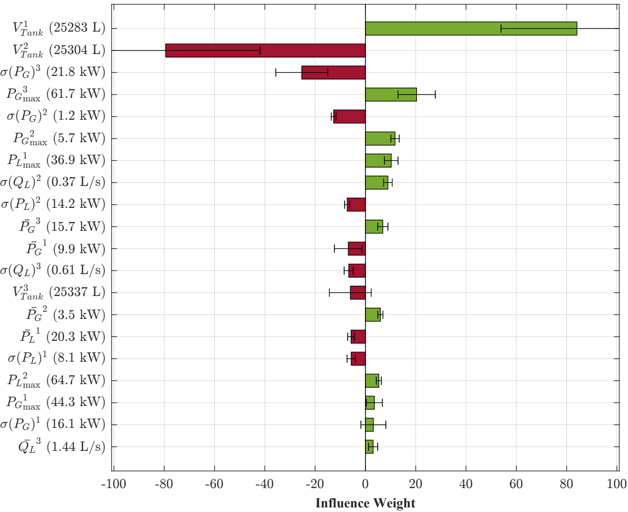
LIME Analysis: Scenario A: Global Peak Target: MG1 — Day 2, 08:30 — Q_s^1 = -1.00 R^2 = 0.60 — RBO=0.83 — Runs=5
