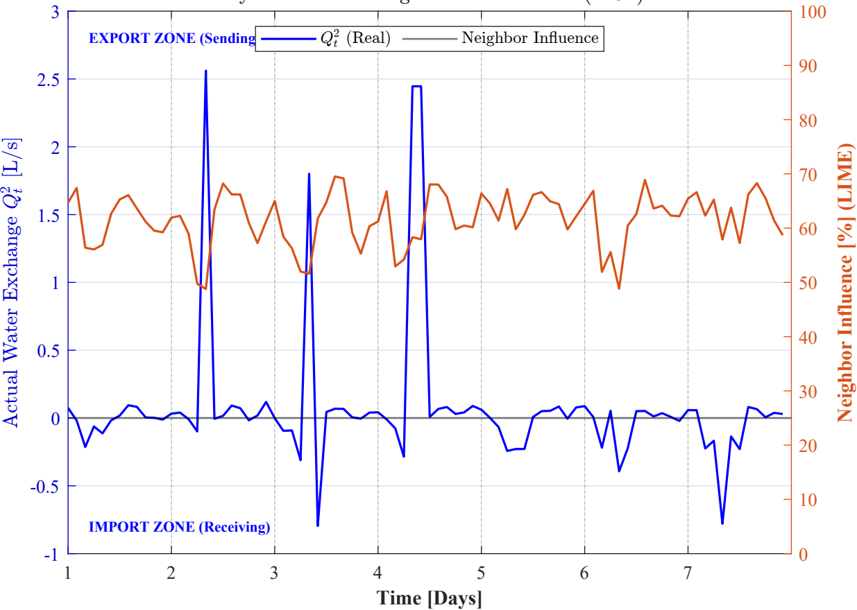
Physical Flow vs. Algorithmic Detection (MG2)
