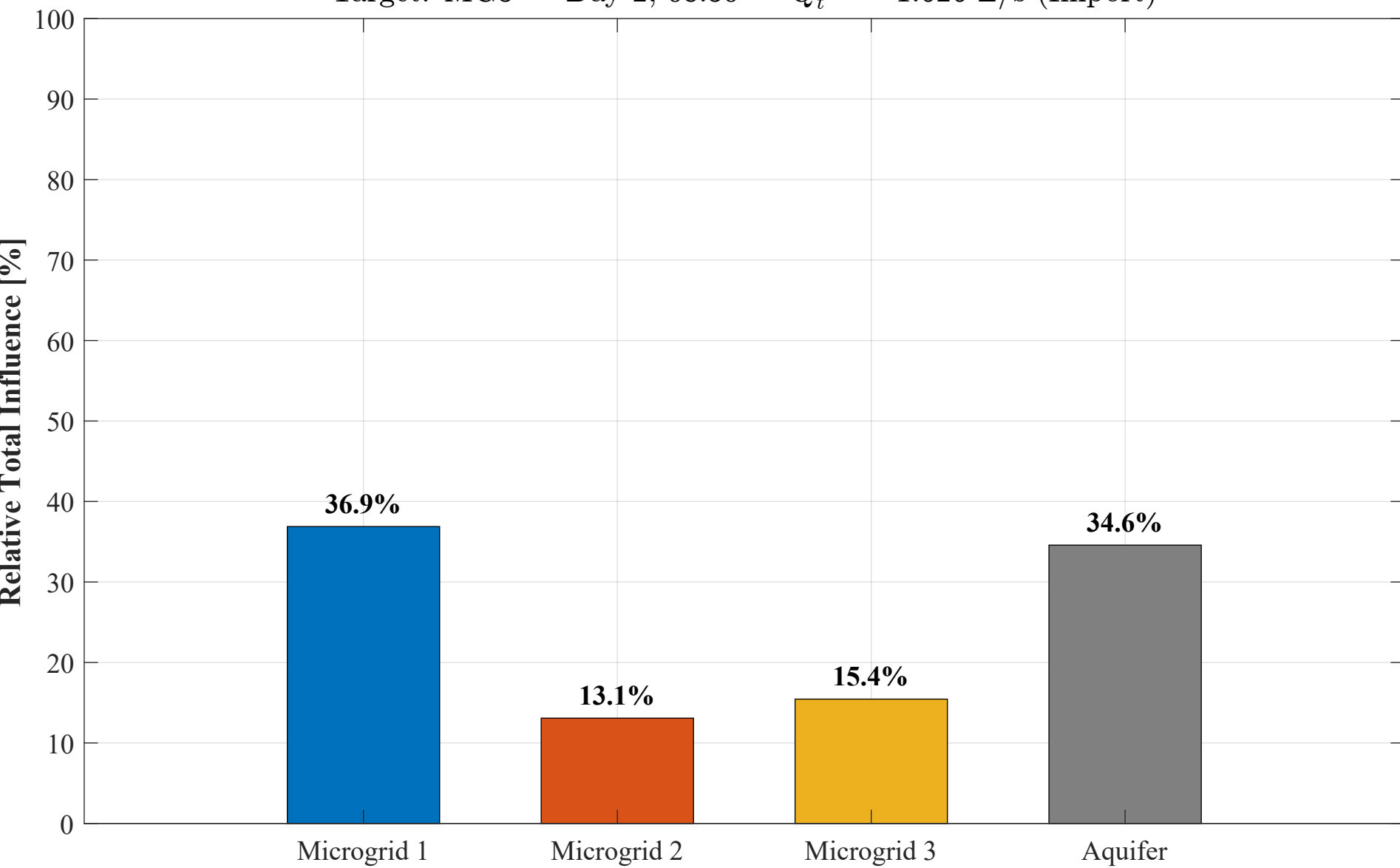
Interaction Analysis: Scenario B: Active Water Export Target: MG3 — Day 2, 08:30 — Q_t^3 = -1.626 L/s (Import)
