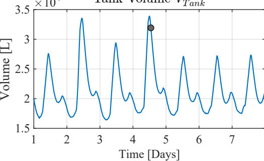
Tank Volume V_{Tank}^2
