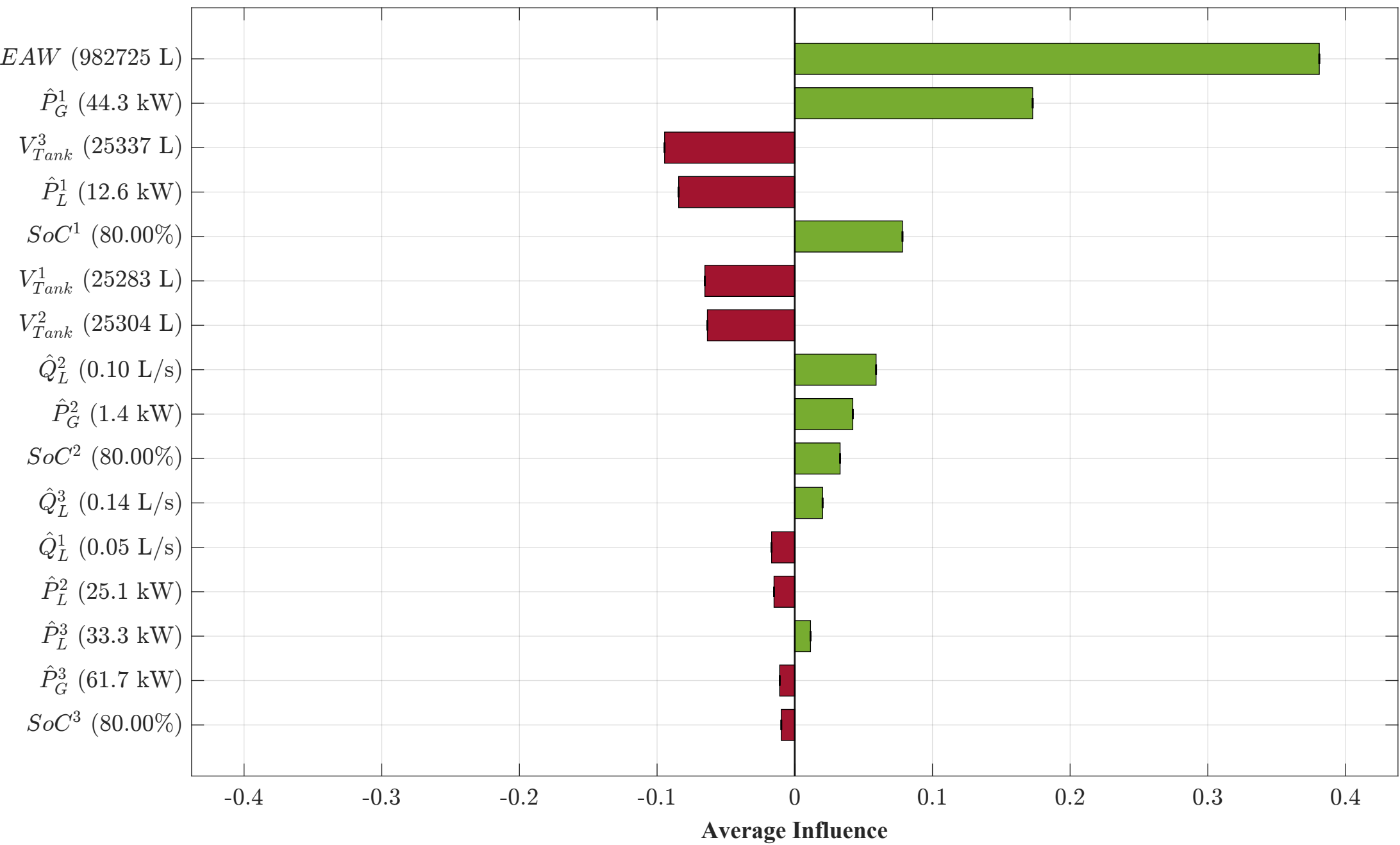
Scenario A: Global Peak Interaction MG3 — Day 2, 08:30 — Q_t^3 = -1.626 L/s (Export)
