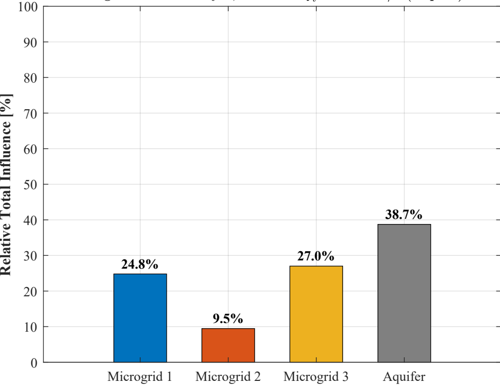
Interaction Analysis: Scenario B: Active Water Export Target: MG2 — Day 2, 08:00 — Q_t^2 = 2.561 L/s (Export)
