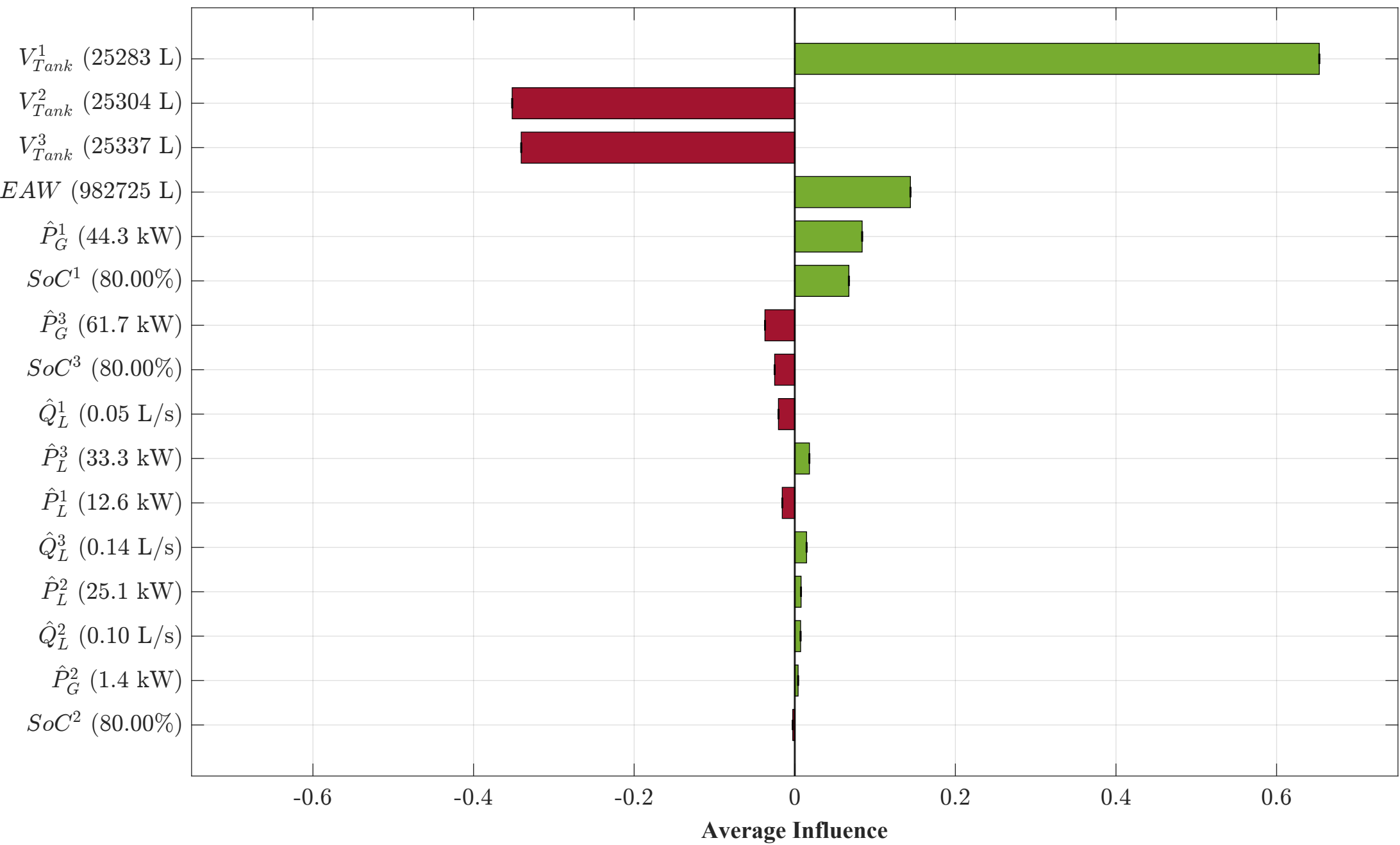
Scenario A: Global Peak Interaction MG1 — Day 2, 08:30 — Q_t^1 = -1.000 L/s (Export)
