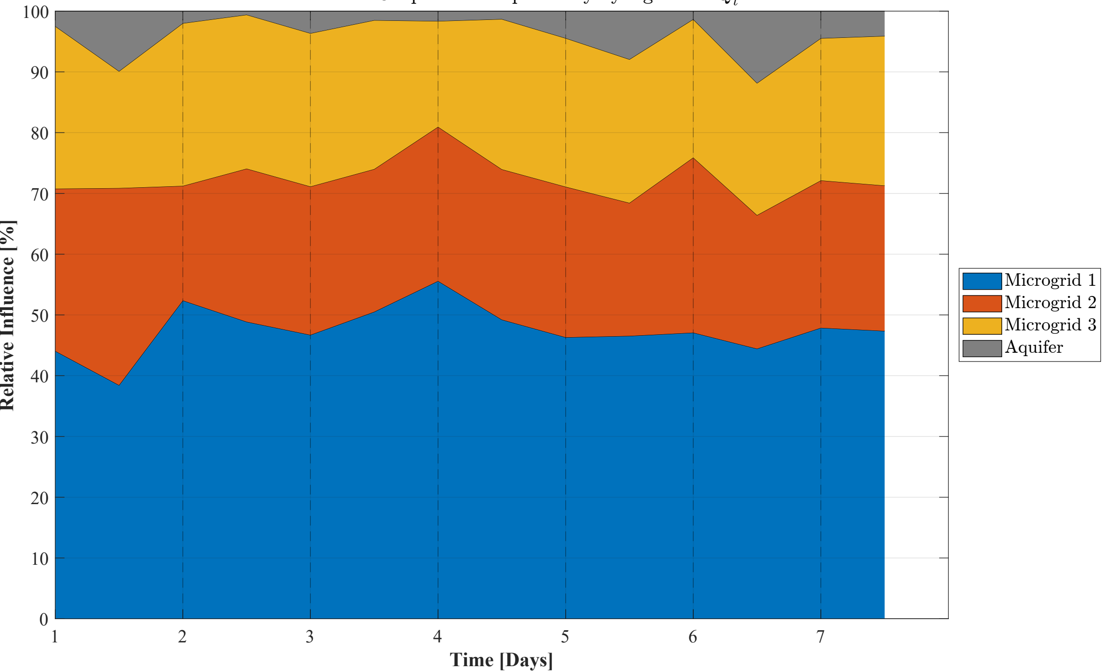
Evolution of Cooperative Dependency by Agent for Q_t^1
