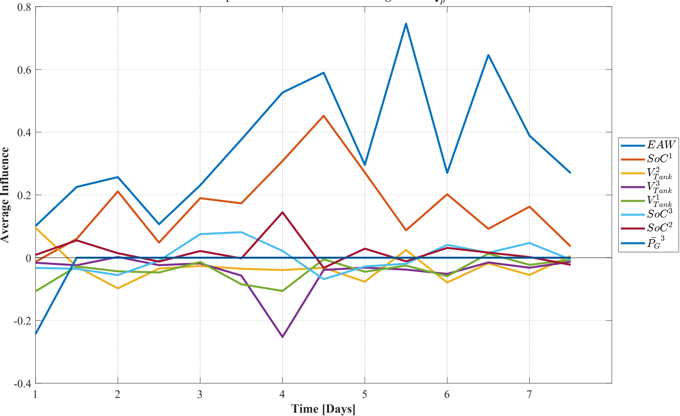
Temporal Evolution of LIME Weights for Q_p^2
