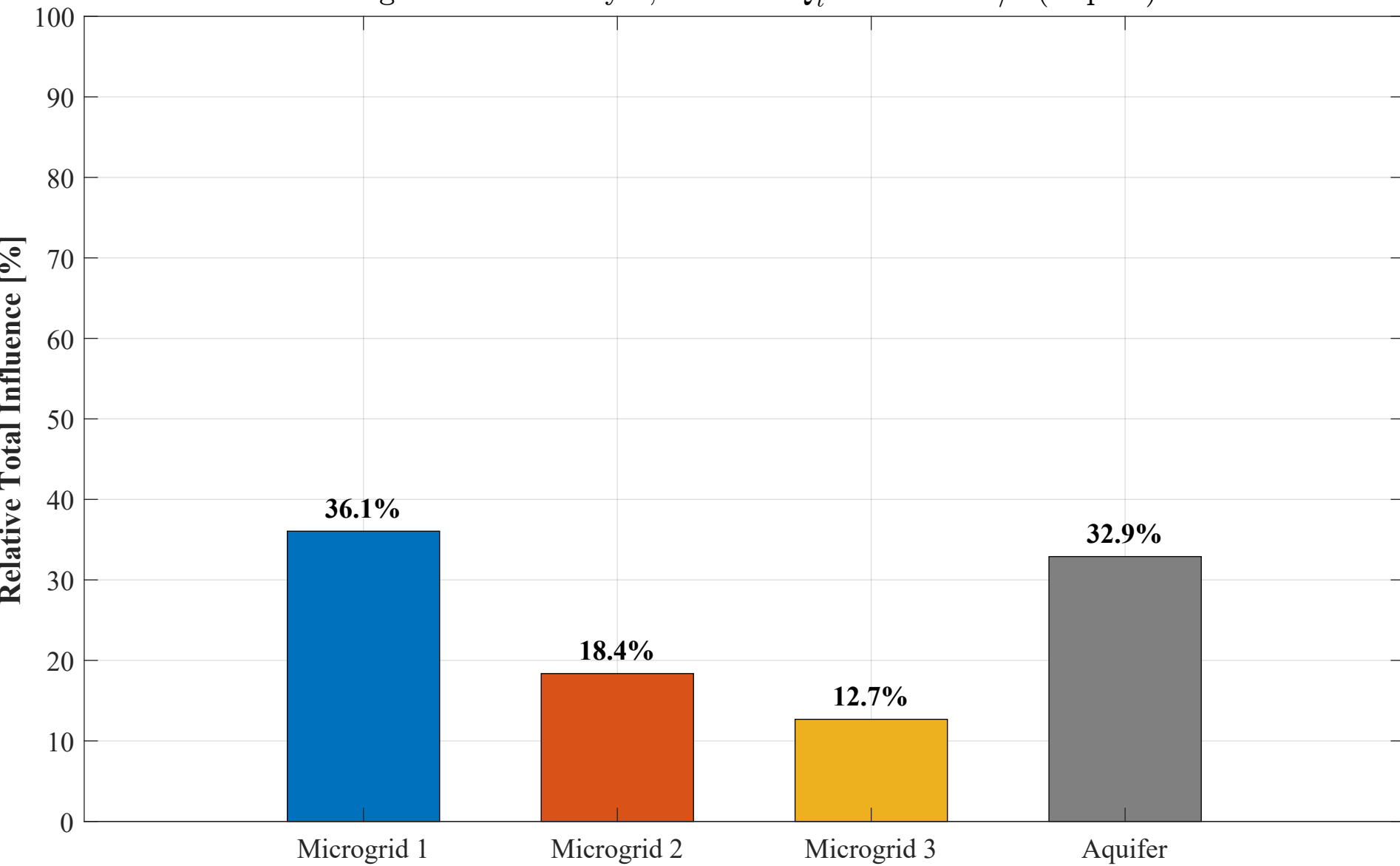
Interaction Analysis: Scenario A: Global Peak Interaction Target: MG3 — Day 2, 08:30 — Q_t^3 = -1.626 L/s (Import)
