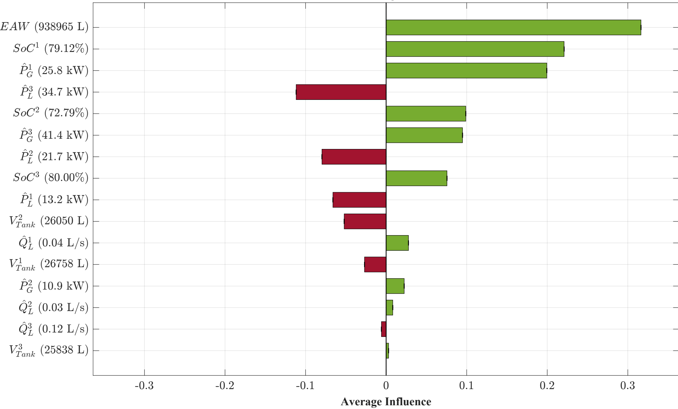
Scenario A: Energy Efficiency (Solar Pumping) MG1 — Day 3, 10:00 — Q_p^1 = 2.205 L/s (Pumping)
