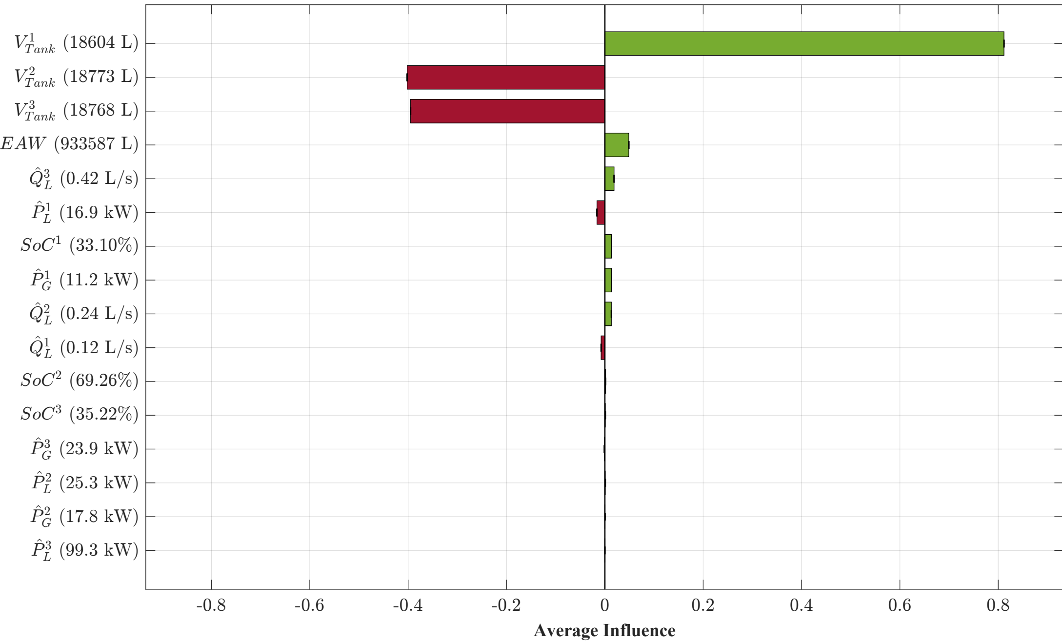
Scenario C: Direct Demand Satisfaction MG1 — Day 4, 08:00 — Q_t^1 = -0.925 L/s (Import)
