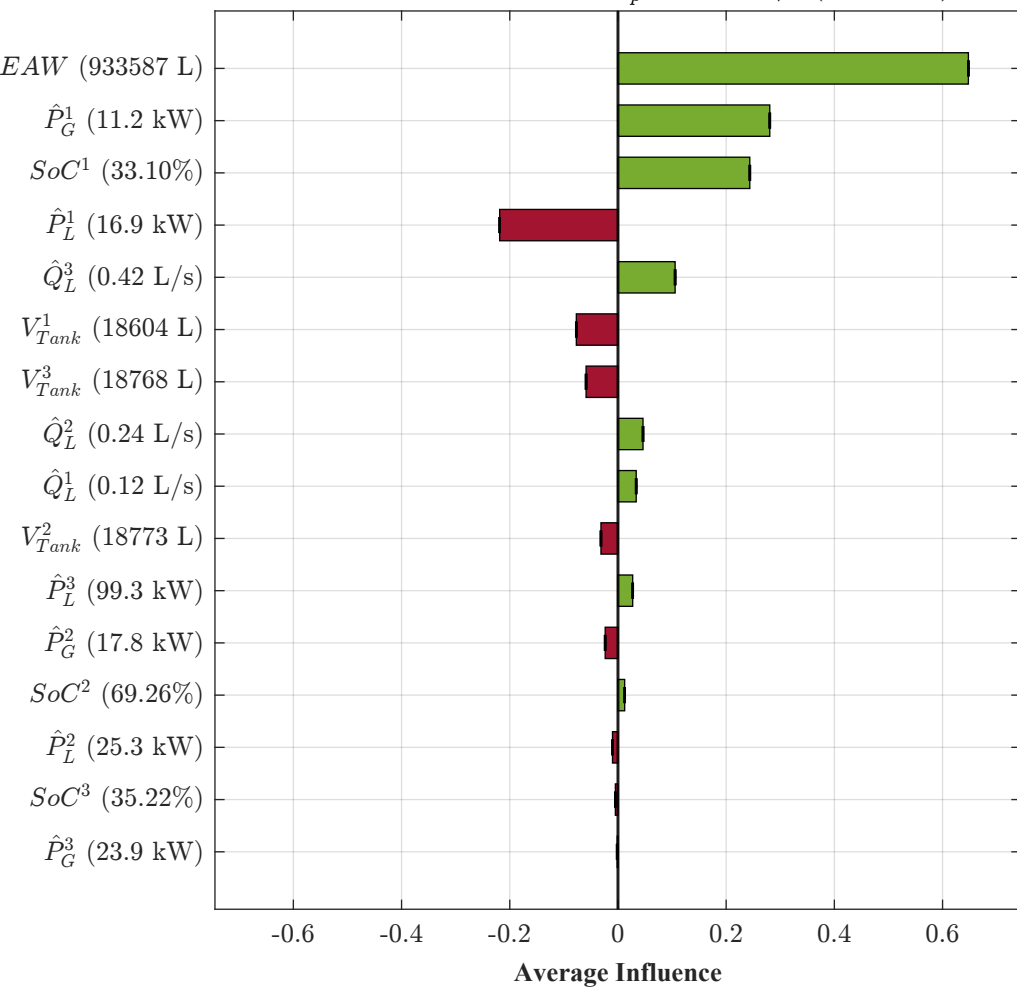
Scenario A: Energy Efficiency (Solar Pumping) MG2 — Day 4, 08:00 — Q_p^2 = 2.446 L/s (Pumping)
