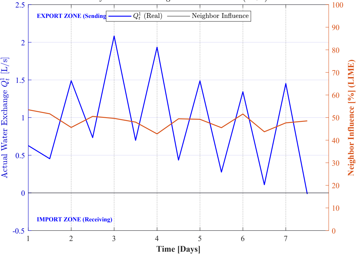
Physical Flow vs. Algorithmic Detection (MG1)
