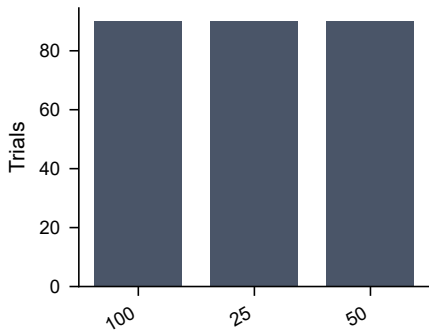
Efficiency
