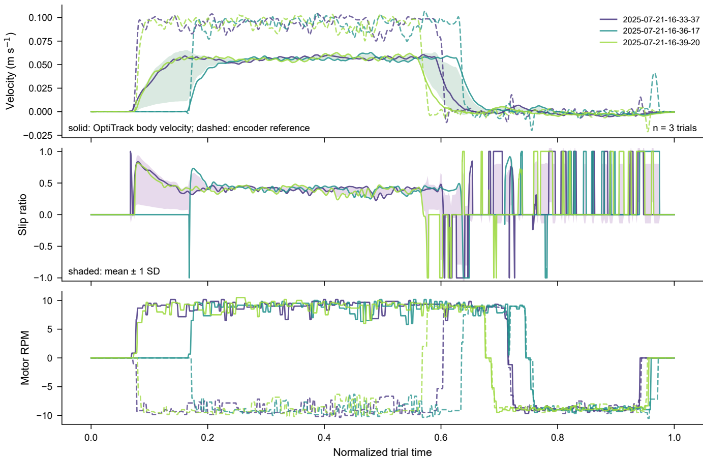
Repeatability of rover kinematics and slip labels across repeated trials (Example group: Vel3_50_Lev3_OFF)
