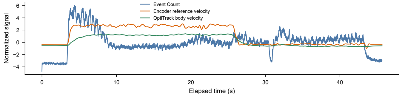
Validation of temporal synchronization across sensing modalities (Example trial: 2025_07_21_16_39_20_Vel3_50_Lev3_OFF)
