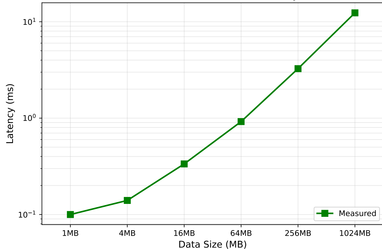
8 GPU NCCL All-Reduce Latency
