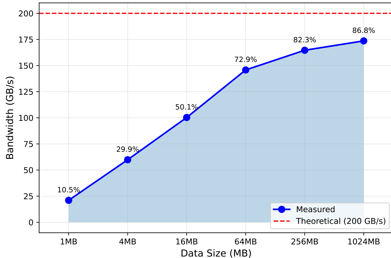
8 GPU NCCL All-Reduce Bandwidth
