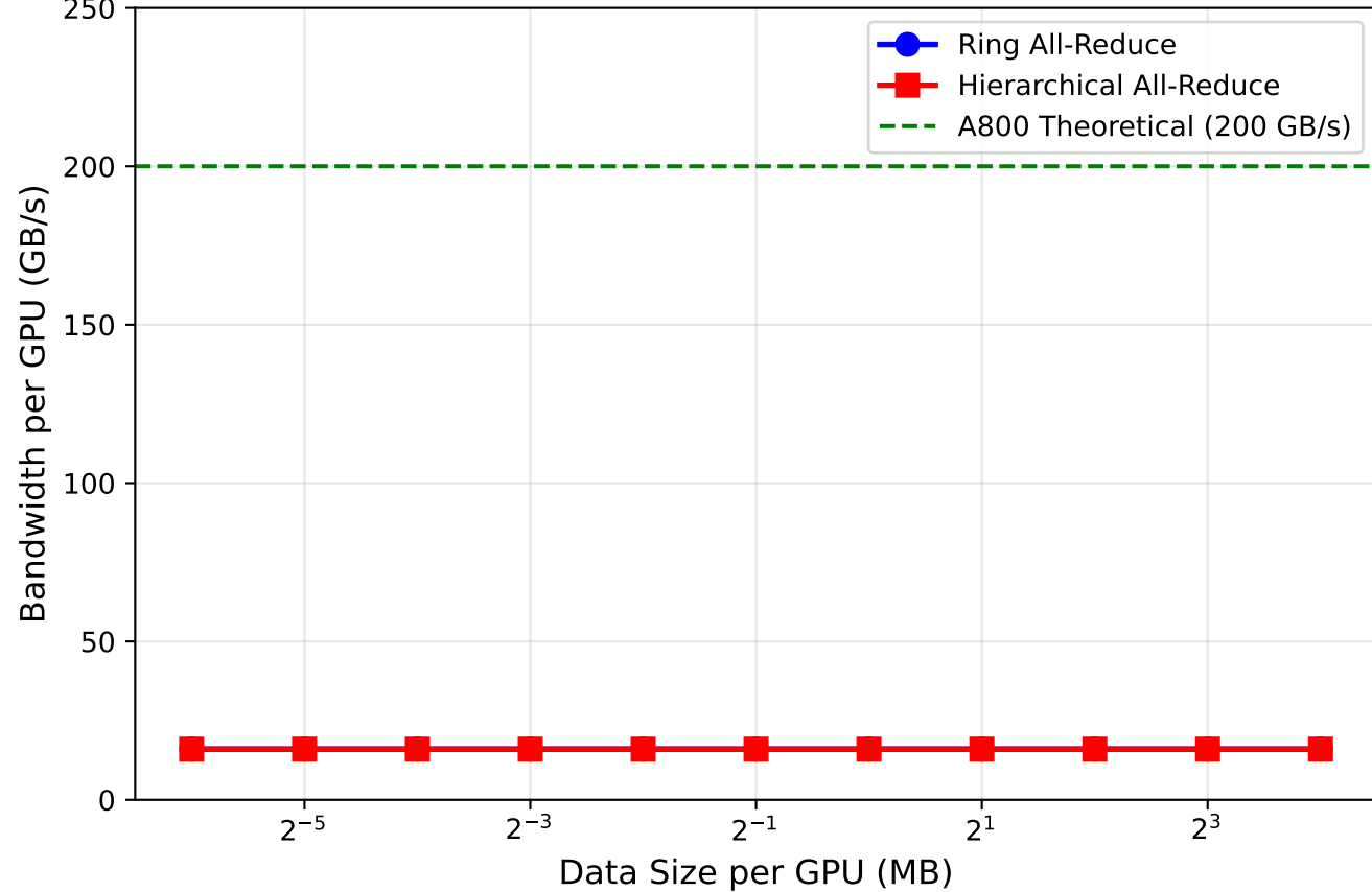
CNSim 64 GPU NVSwitch - Bandwidth
