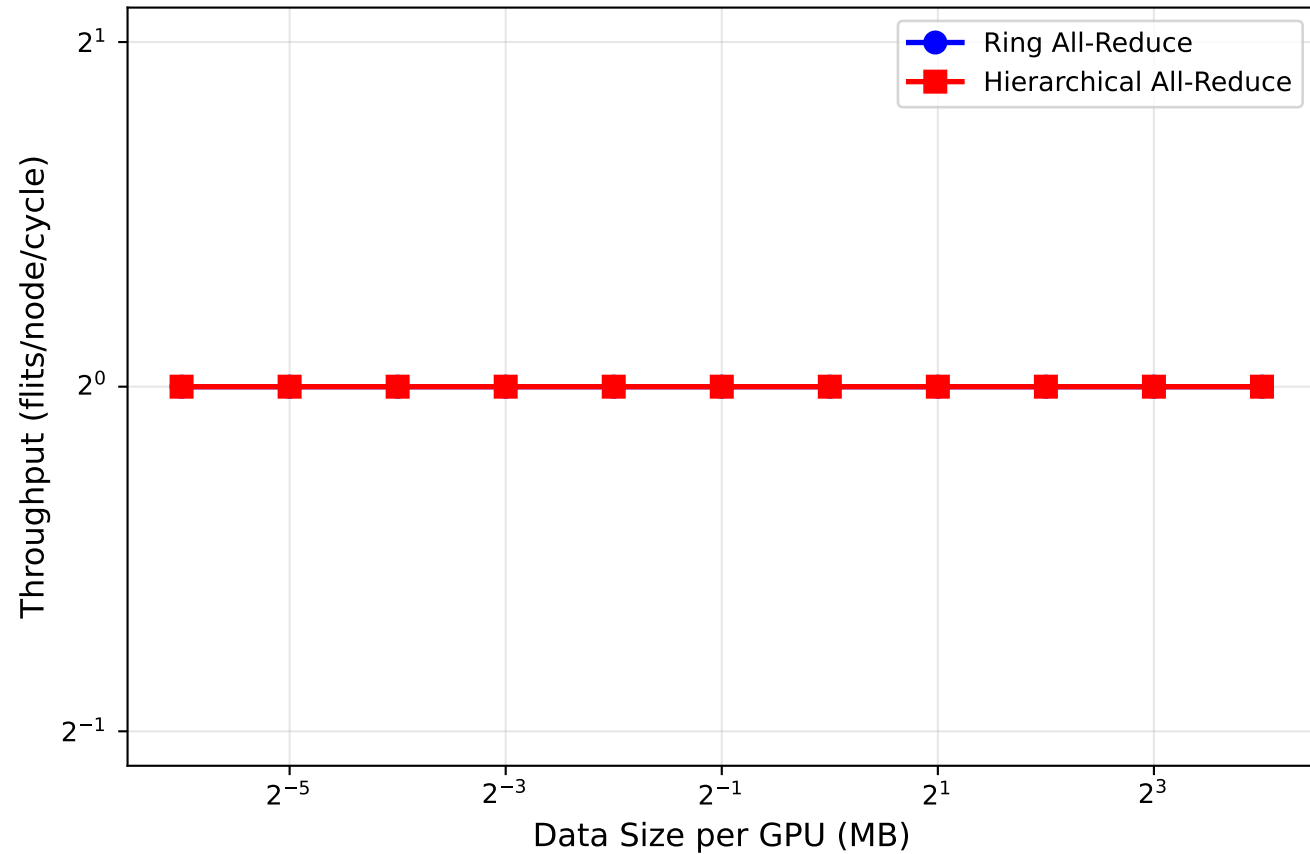
CNSim 64 GPU NVSwitch - Throughput
