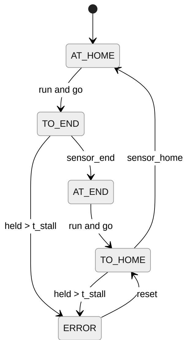
Figure 5. FB_Actuator_T1 robust (1.6)
