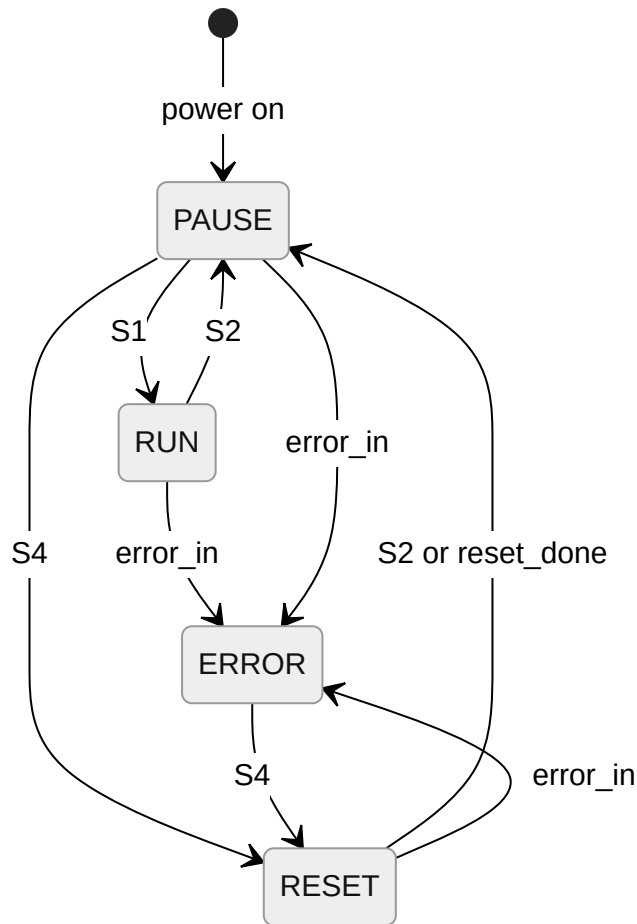
Figure 2. FB_Panel finite-state diagram (1.4)
