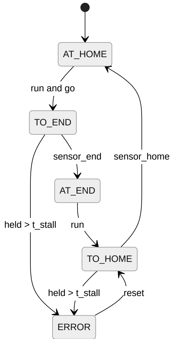
Figure 7. FB_Actuator_T2 robust (1.8)
