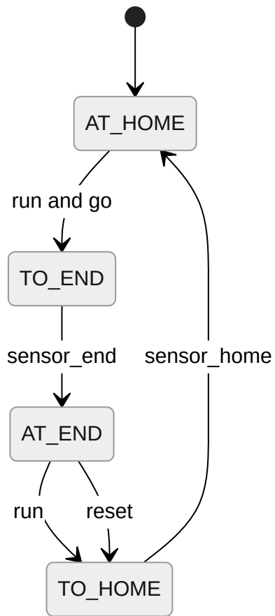
Figure 6. FB_Actuator_T2 proper (1.7)
