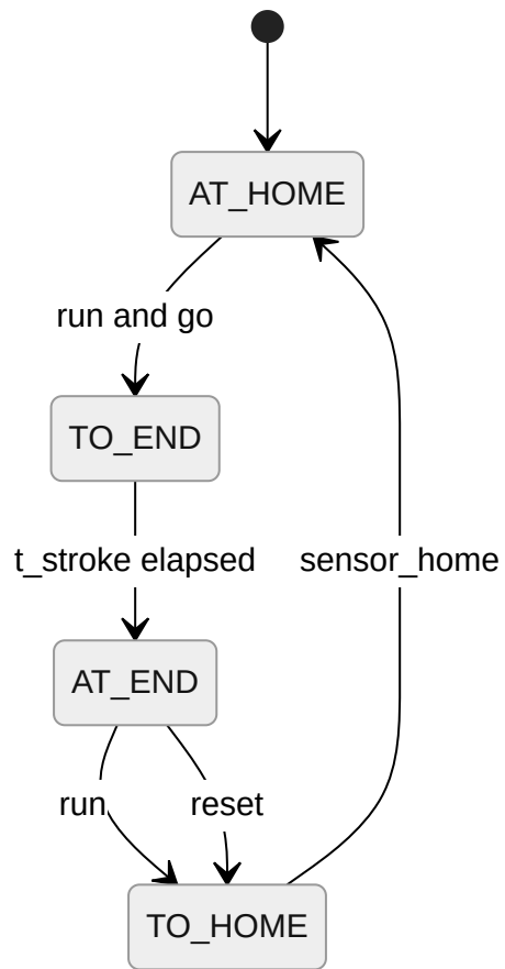
Figure 9. FB_Actuator_T3 proper (2.4)
