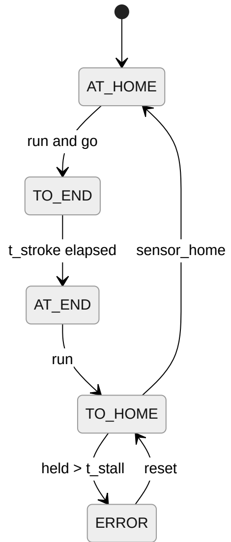
Figure 10. FB_Actuator_T3 robust (2.5)
