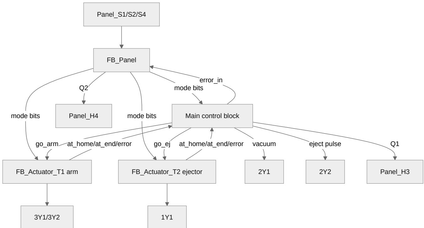
Figure 3. Distributing block diagram (4 blocks, 1.9)
