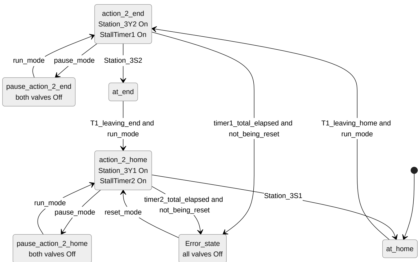
Figure 6. FB_Actuator_T1 finite-state diagram, robust (1.6)
