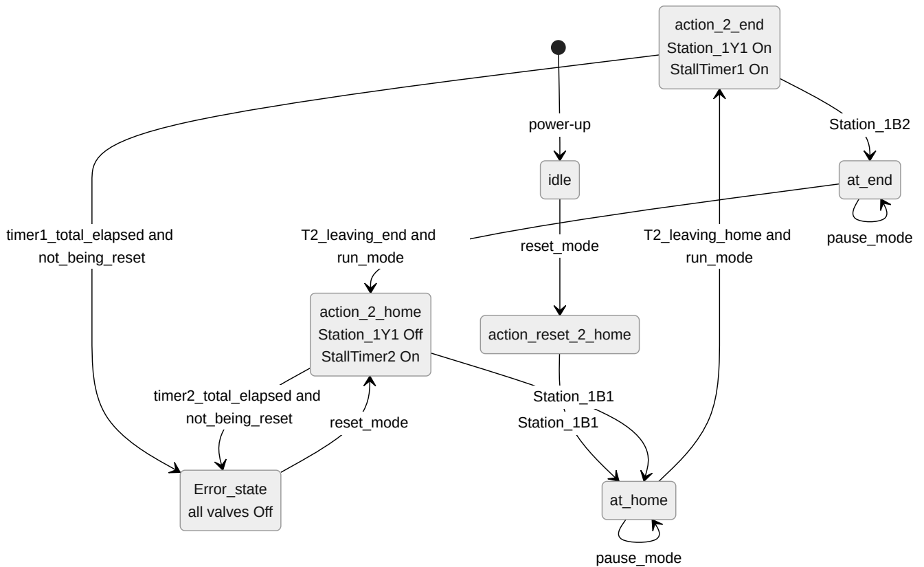
Figure 9. Block diagram updated for robustness, ejection cylinder (1.8)
