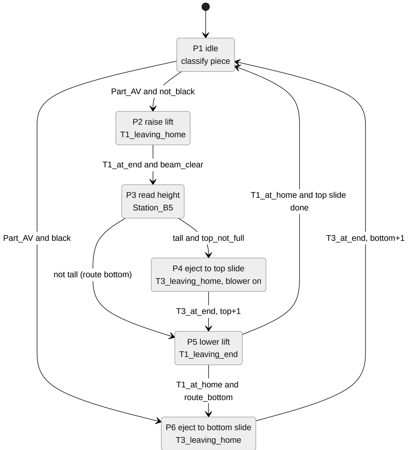
Figure 19. Env per-piece sequence, written in the actuator blocks' signals (2.6)
