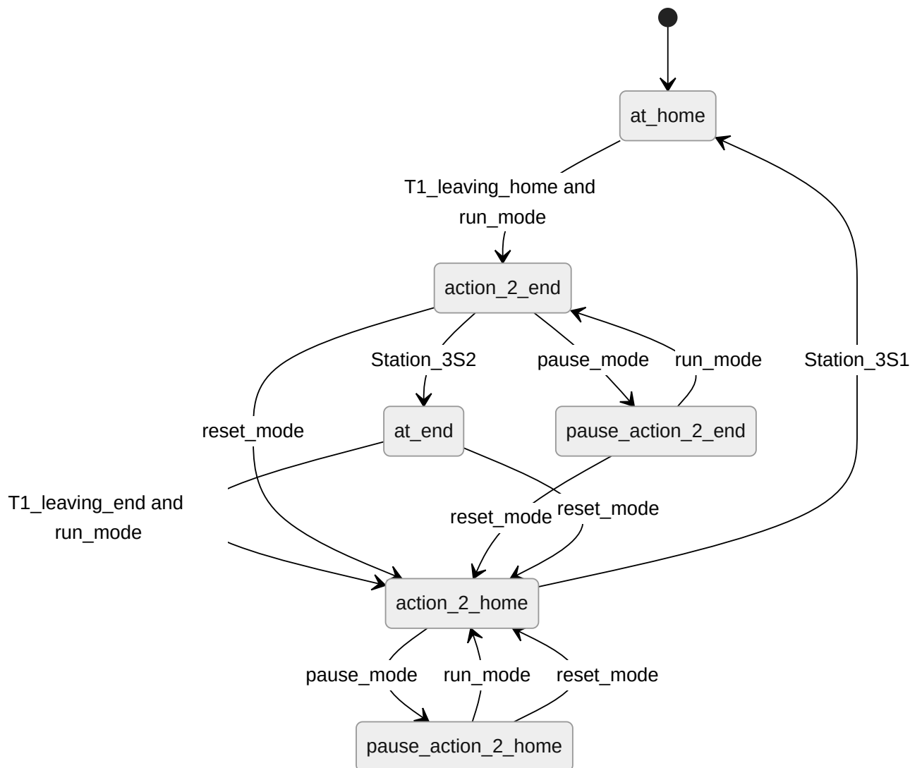
Figure 4. FB_Actuator_T1 finite-state diagram, proper (1.5)
