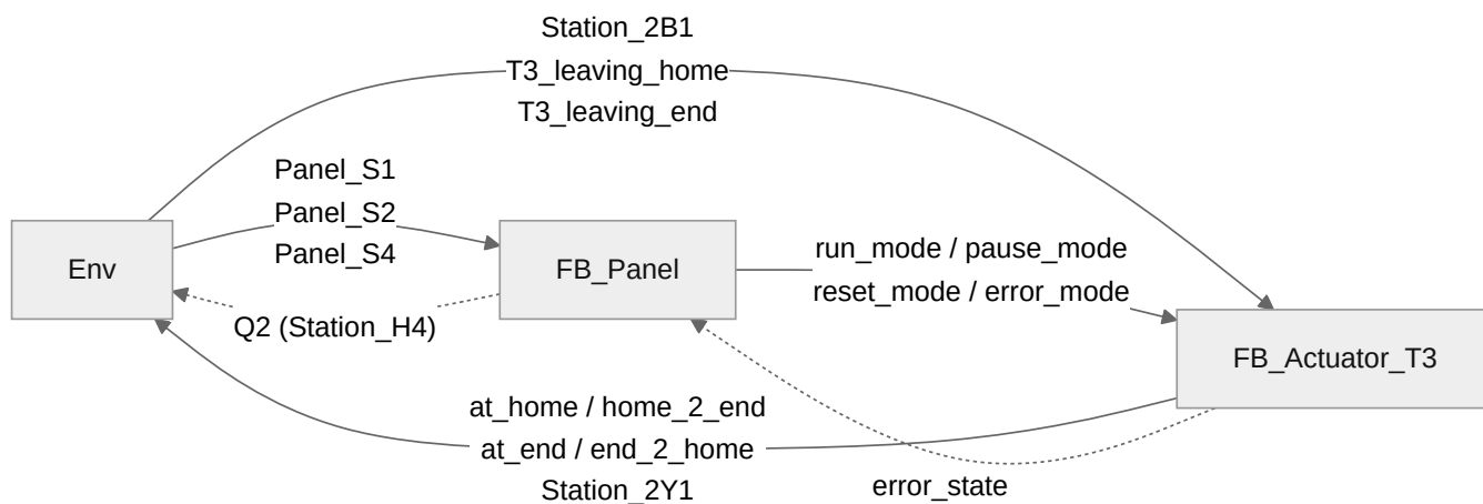
Figure 15. Block diagram, Testing ejecting cylinder (2.4; dashed additions are the 2.5 robustness update)
