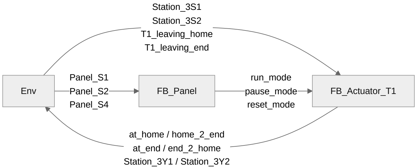
Figure 3. Block diagram, swivel arm (1.5)
