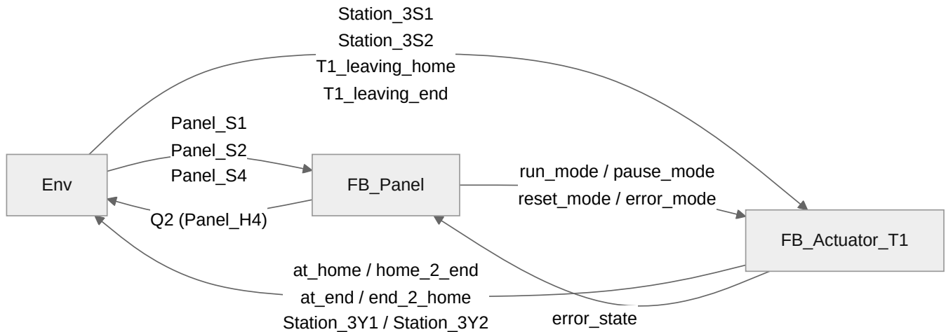
Figure 5. Block diagram updated for robustness, swivel arm (1.6)
