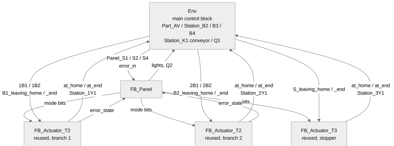
Figure 20. Sorting block diagram (5 blocks, 3.2)
