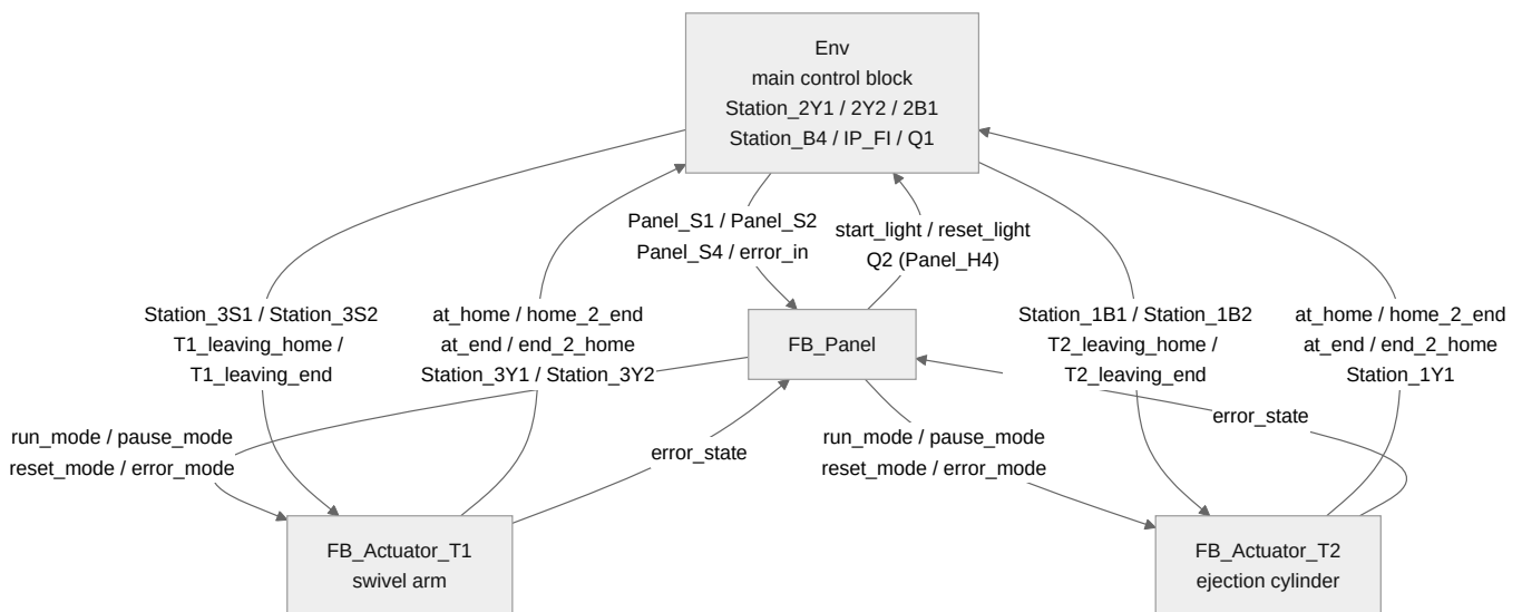
Figure 11. Distributing block diagram (4 blocks, 1.9)
