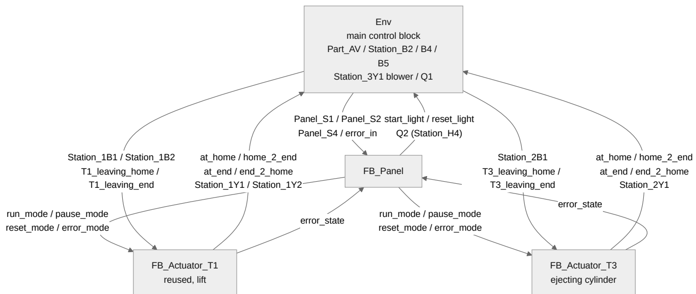
Figure 18. Testing block diagram (4 blocks, 2.6)
