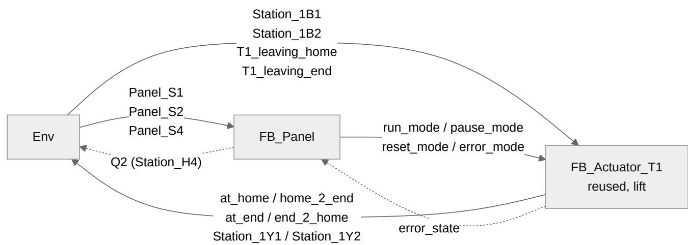
Figure 14. Block diagram, Testing lift (2.2; dashed additions are the 2.3 robustness update)
