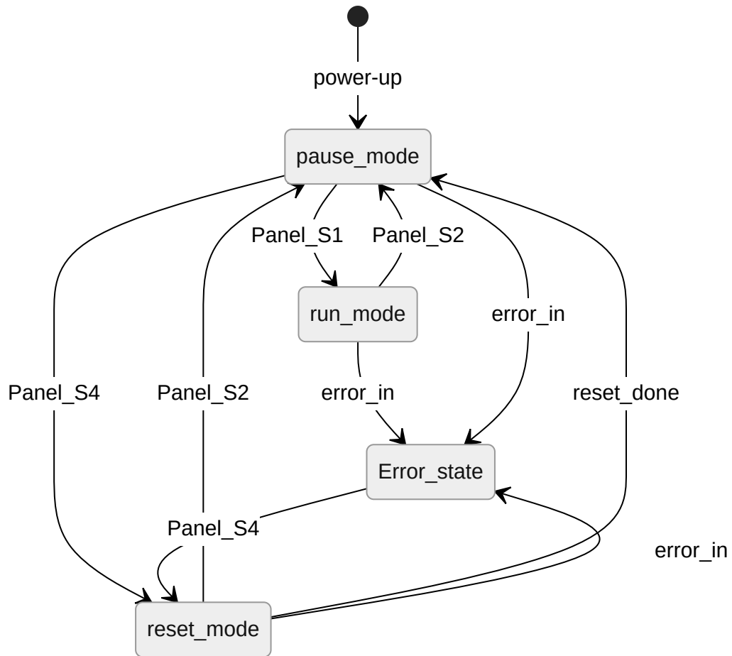
Figure 12. FB_Panel finite-state diagram updated for the full station (1.9 / 1.10)
