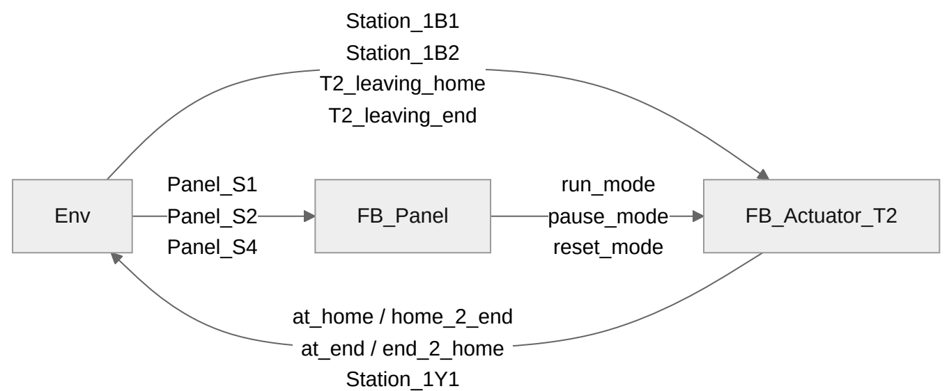
Figure 7. Block diagram, ejection cylinder (1.7)
