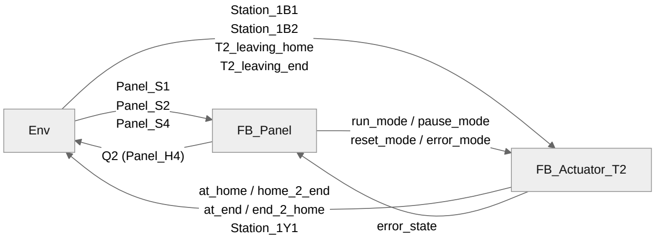
Figure 9. Block diagram updated for robustness, ejection cylinder (1.8)
