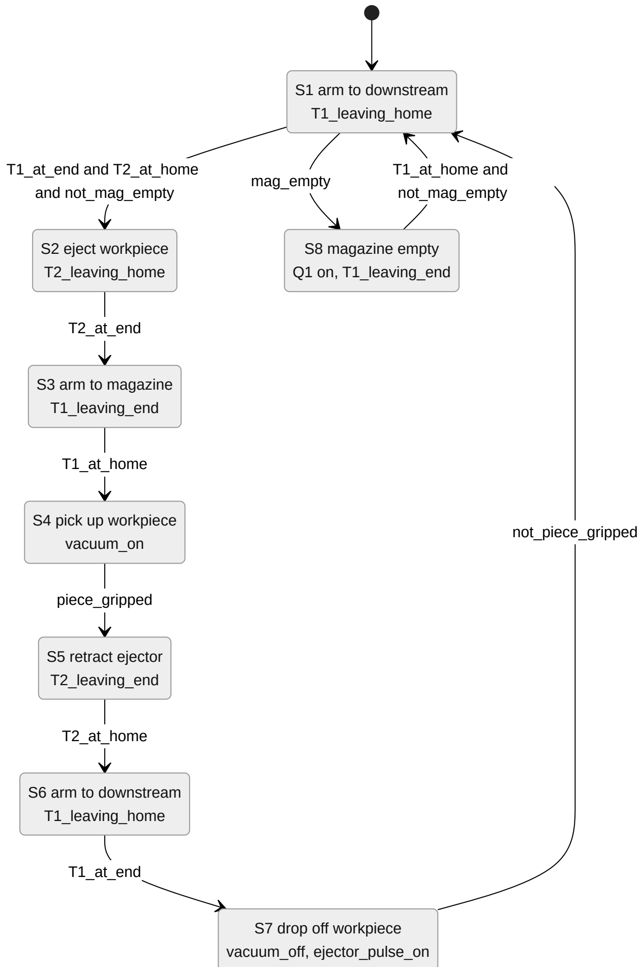
Figure 13. Env station sequence, written in the actuator blocks' signals (1.9)
