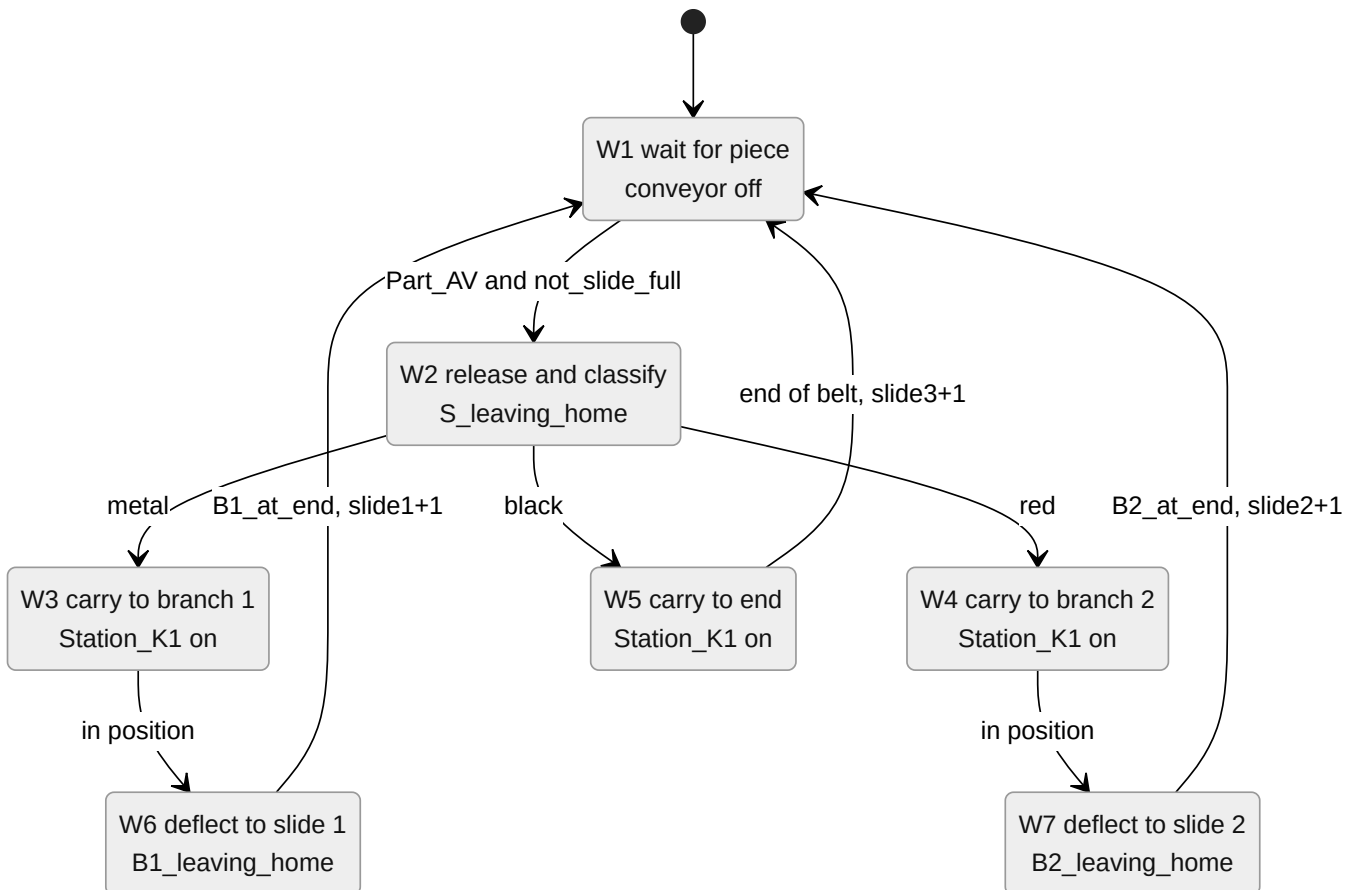
Figure 21. Env per-piece sequence, written in the actuator blocks' signals (3.2)
