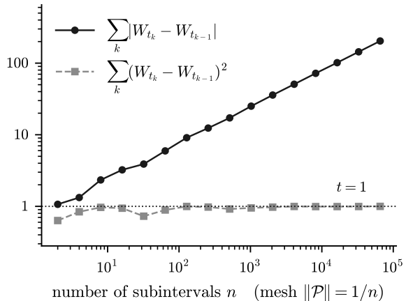
Partition sums as the mesh is refined
