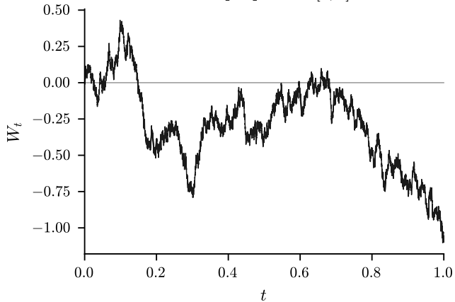
A sample path on [0, 1]
