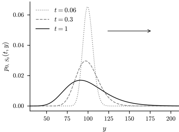
Forward: the density spreads out
