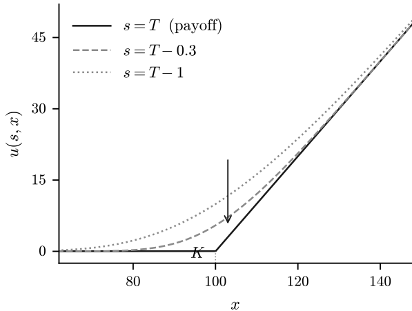
Backward: the payoff is smoothed
