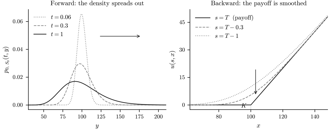
Figure 1.3: The two equations of the table, for geometric Brownian motion with \sigma = 0.25 , r = 0 and S_0 = 100 . Left : the forward (Fokker–Planck) equation (1.87) transports the density forwards from the point mass at S_0 , which spreads as t increases; this is the direction calibration works in, since S_0 is observed today. Right : the backward equation (1.83) transports the call payoff (x - K)^+ backwards from maturity, smoothing the kink at the strike as the remaining time T - s grows; this is the direction pricing works in. The arrows mark the direction of time in each panel.
