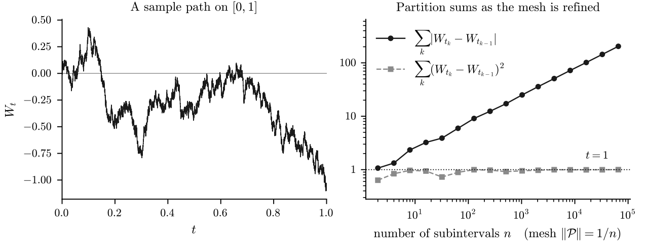
Figure 1.2: A Brownian path on [0, 1] (left) and its partition sums (right, logarithmic on both axes) over the dyadic partitions \mathcal{P}_n with \|\mathcal{P}_n\| = 1/n . The sum of absolute increments grows without bound, with slope \frac{1}{2} on these axes, so that it diverges like \sqrt{n} — while the sum of squared increments settles at t = 1 . This is Proposition 1.45 and (1.42) side by side: the same path has infinite total variation and quadratic variation exactly t , and it is this pair of facts that makes the Riemann–Stieltjes integral unavailable and the Itô integral necessary.
