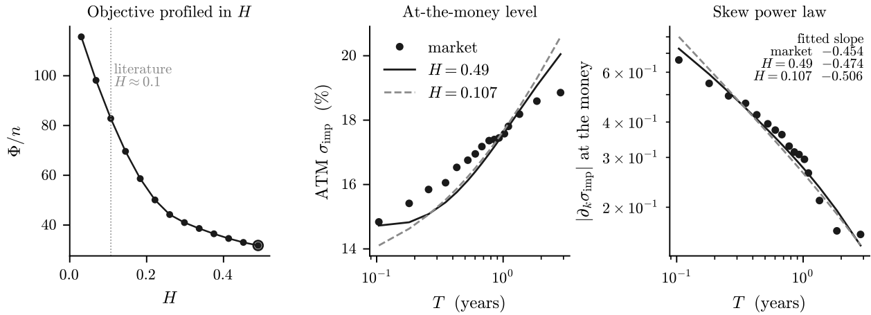
Figure 4.3: Left: the objective profiled in H , the other five parameters re-optimised at each point; it is strictly monotone and its minimum is the boundary H = 0.49 , marked. Centre: the at-the-money term structure, market against the two calibrated models. Right: the same two models and the market on log axes, with the fitted slopes of |\partial_k \sigma_{\text{imp}}| against T . The three slopes agree to within 0.06 although the two models differ in H by a factor of nearly five, which is Table 4.7 drawn: over this maturity range the skew power law does not separate rough from smooth.
