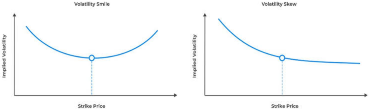
Figure 2.1: The two shapes described above. Left: the usual foreign exchange smile, symmetric about the money and rising into both wings. Right: the typical equity skew, falling monotonically in the strike, so that downside protection carries the highest implied volatility. The curves are illustrative shapes and not drawn from market quotes.
