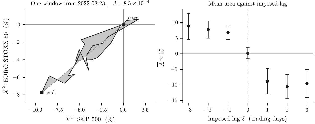
Figure 4.4: Left: one monthly window drawn as a path in the plane of the two cumulative log-returns, with the chord joining its endpoints dashed. The Lévy area A_{0,T} is the shaded signed area between path and chord; the endpoints alone fix \text{Sym } \mathbb{X}_{0,T} and say nothing about it, which is Proposition 3.73. Right: the mean area over 135 such windows as a function of an imposed lag \ell , with \pm 2 standard errors. The response reverses in sign with \ell though it is not exactly odd in magnitude, is detected at more than four standard errors at every non-zero lag, and crosses zero at \ell = 0 alone.
