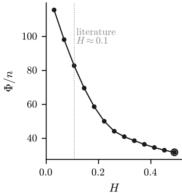
Objective profiled in H
