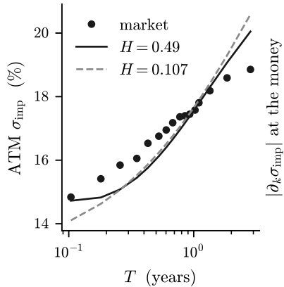
At-the-money level
