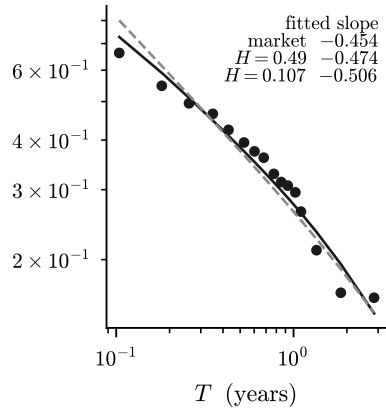
Skew power law
