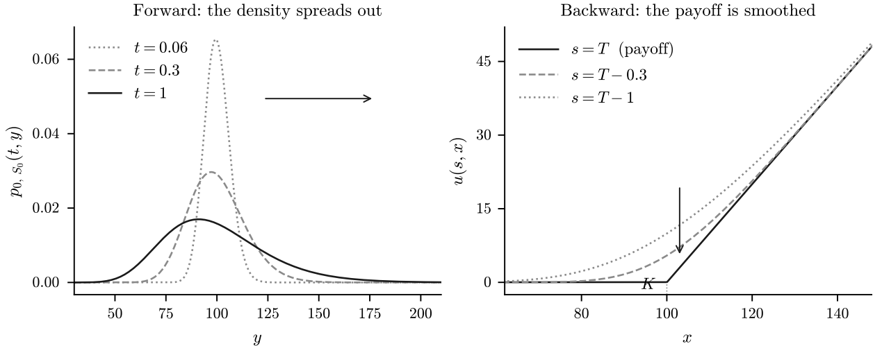
Figure 1.3: The two equations of Table 1.3, for geometric Brownian motion with \sigma = 0.25 , r = 0 and S_0 = 100 . Left: the forward (Fokker–Planck) equation (1.85) transports the density forwards from the point mass at S_0 , which spreads as t increases. Right: the backward equation (1.81) transports the call payoff (x - K)^+ backwards from maturity, smoothing the kink at the strike as the remaining time T - s grows; this is the direction pricing works in.
