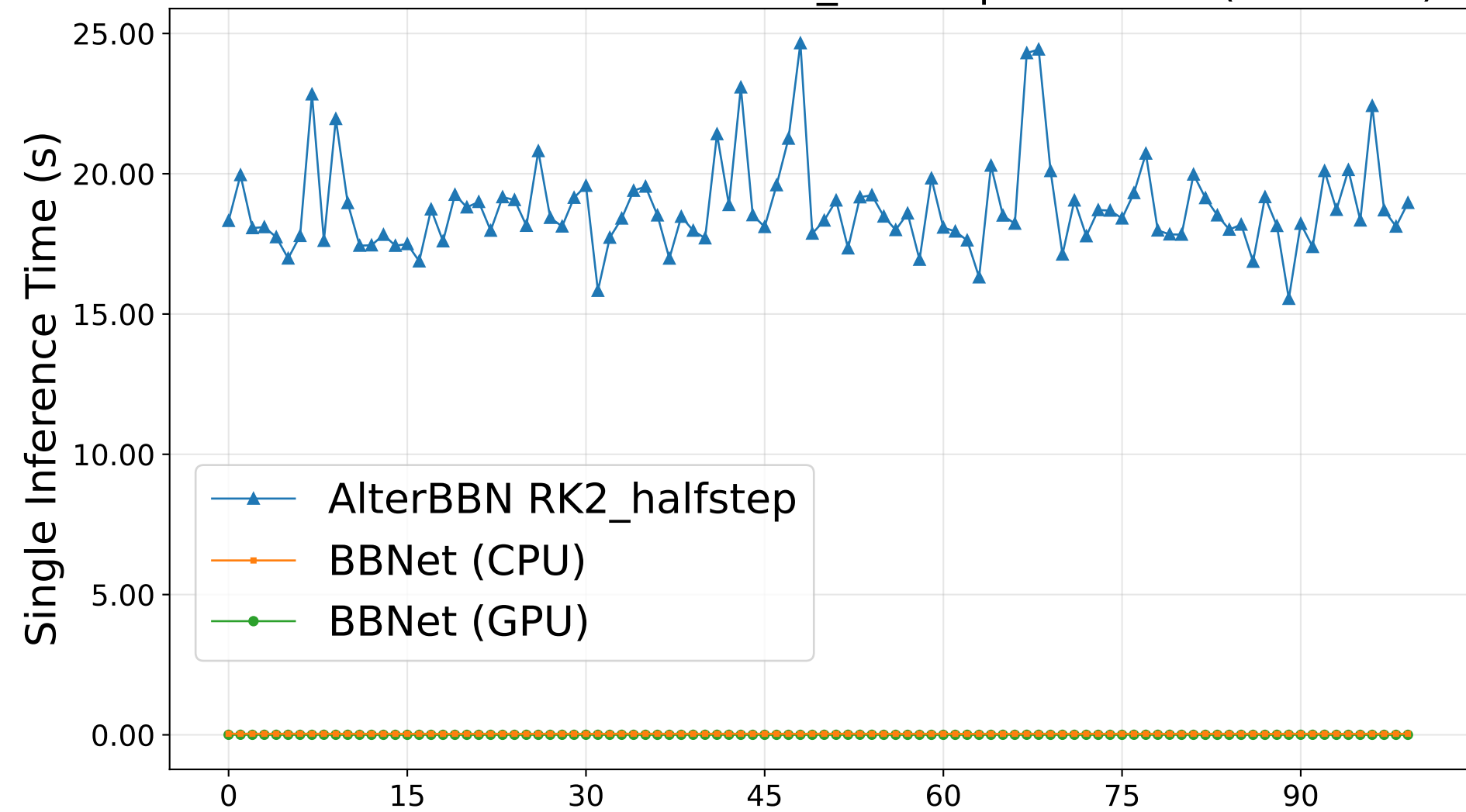
Inference Time: AlterBBN RK2_halfstep vs BBNNet (CPU/GPU)
