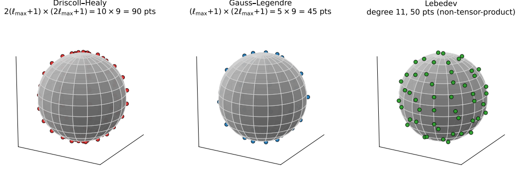
Figure 1: Three quadrature node layouts on S^2 for \ell_{\max} = 4 . Driscoll–Healy uses an equiangular tensor-product grid with 2(\ell_{\max} + 1) latitude rings, twice what Gauss–Legendre needs for the same exactness. Lebedev avoids the tensor-product structure entirely, distributing roughly the same number of points more uniformly. All three are exact for spherical polynomials of degree \leq 2\ell_{\max} .
