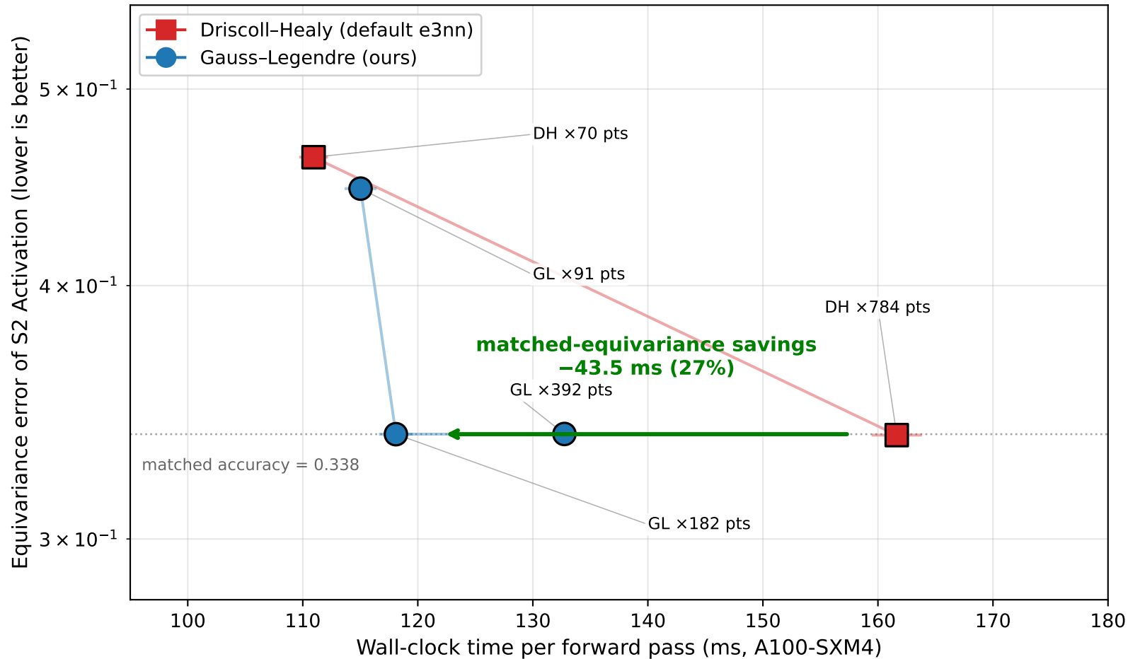
Pareto frontier: equivariance vs wall-clock EquiformerV2 fairchem default (12 layers, lmax=6, mmax=2), batch=8
